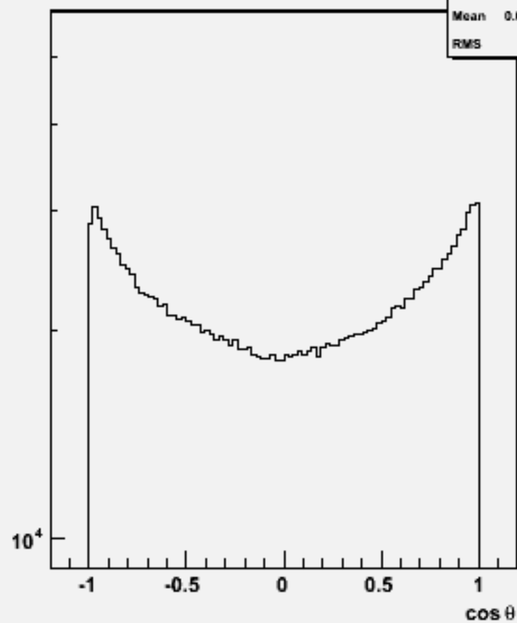
Particle cos \theta : 106429 physsim-ttz-all-all
