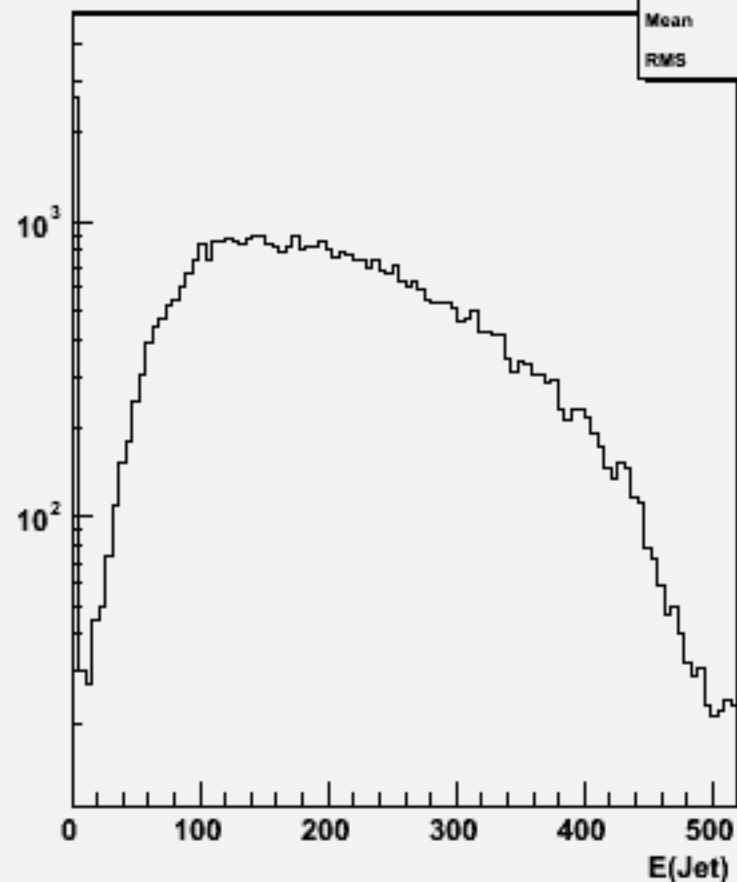
Jet energies(All jets)106429 physsim-ttz-all-all
