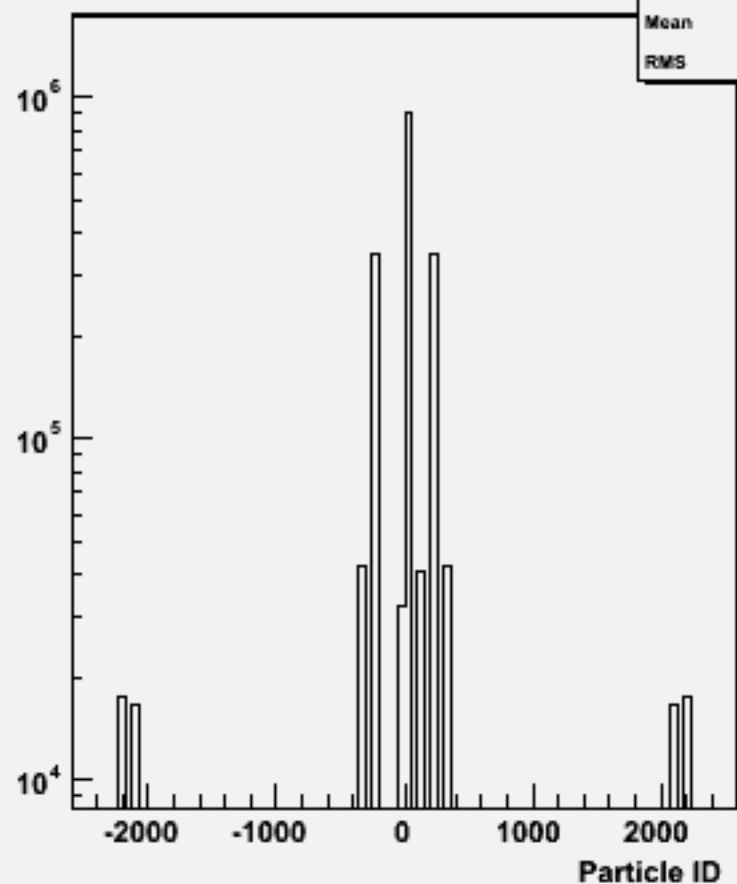
Particle ID : 106429 physsim-ttz-all-all
