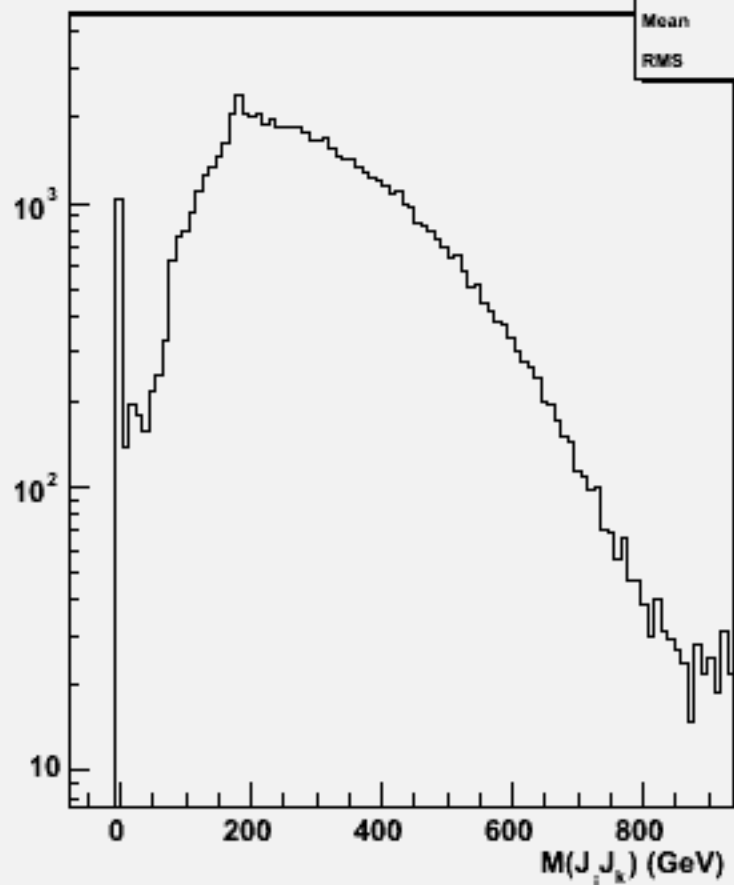
2jets mass(All comb)106429 physsim-ttz-all-all
