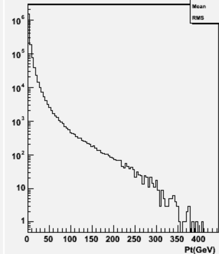
Particle Pt : 106429 physsim-ttz-all-all
