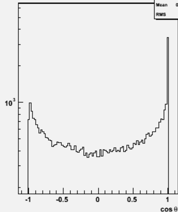
Jet cosθ (All jets)106429 physsim-ttz-all-all
