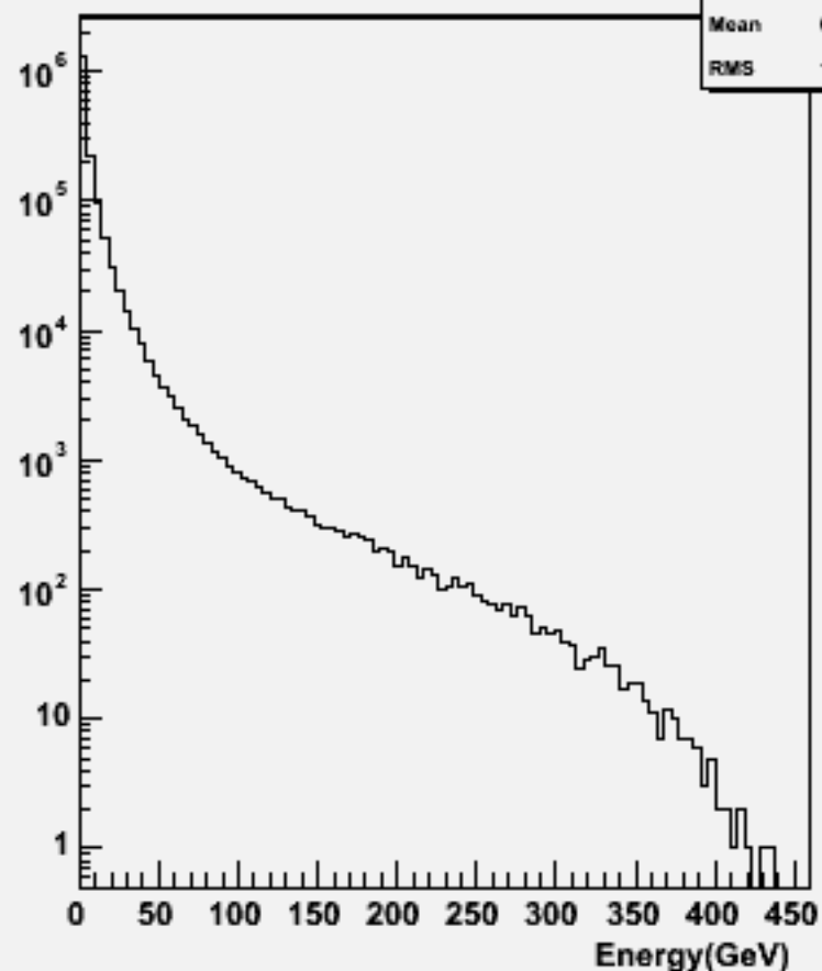
Particle Energy : 106429 physsim-ttz-all-all
