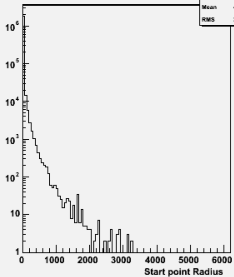
Start point R : 106429 physsim-ttz-all-all
