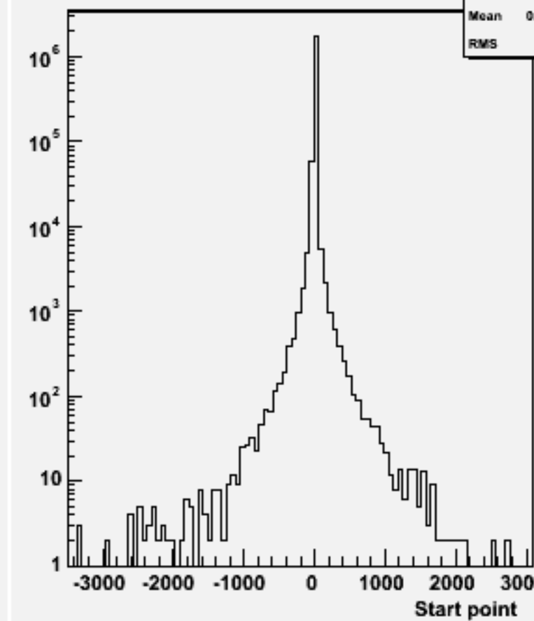
Start point Z : 106429 physsim-ttz-all-all
