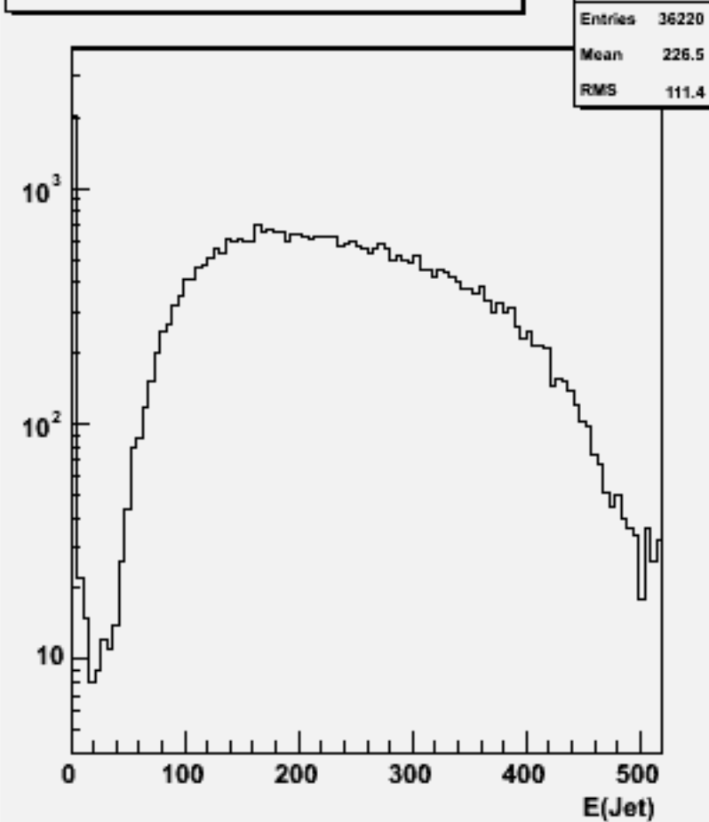
Jet energies(All jets)106402 physsim-tth-6q-hbb
