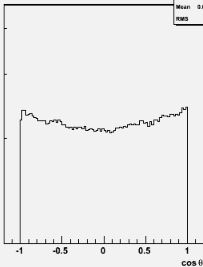
Particle cos \theta : 106402 physsim-tth-6q-hbb
