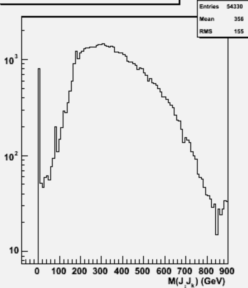
2jets mass(All comb)106402 physsim-tth-6q-hbb
