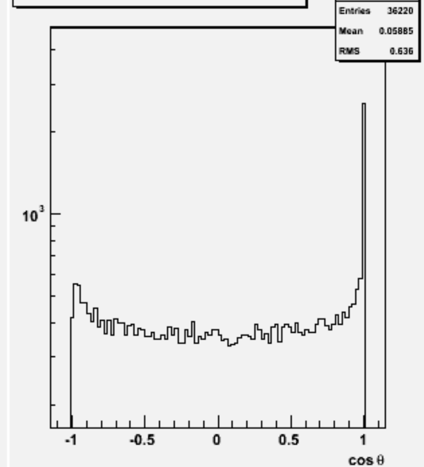
Jet cos \theta (All jets)106402 physsim-tth-6q-hbb
