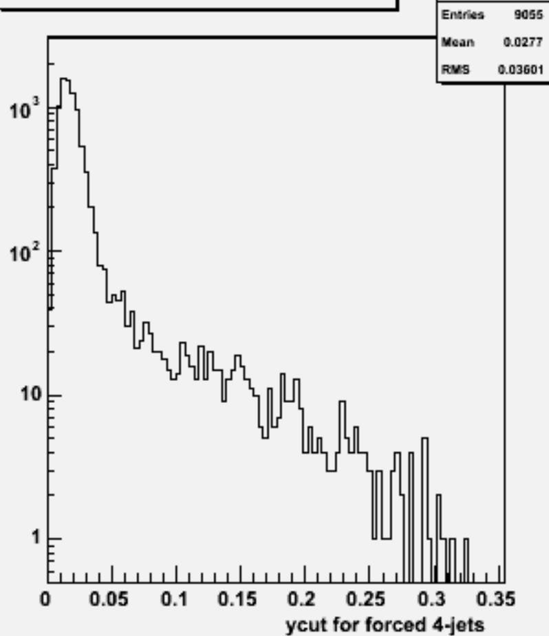
Ycut for 4-jets :106402 physsim-tth-6q-hbb
