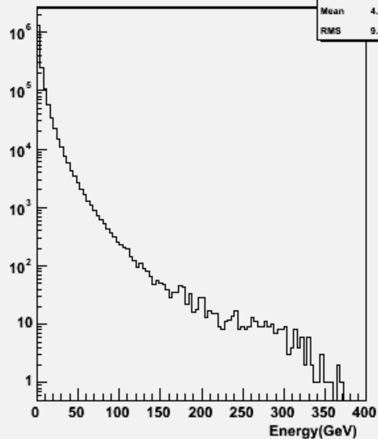
Start point R : 106402 physsim-tth-6q-hbb
