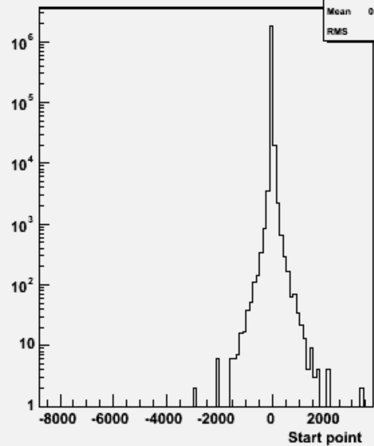
Start point Z : 106402 physsim-tth-6q-hbb
