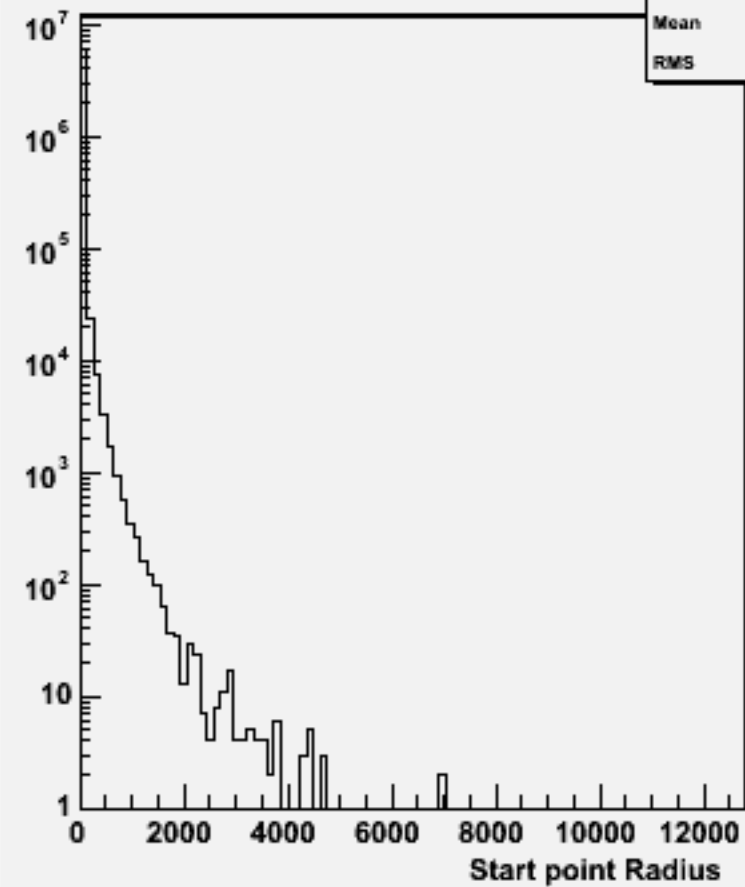
Start point R : p106148 physsim-ttz-2l2nbb_zqq
