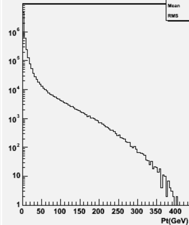
Start point Z : p106148 physsim-ttz-2l2nbb_zqq
