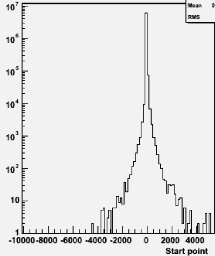
Start point Z : p106147 physsim-ttz-2l2nbb_zqq
