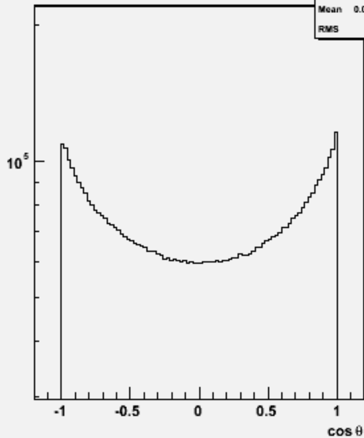
Particle cos θ : p106147 physsim-ttz-2l2nbb_zqq
