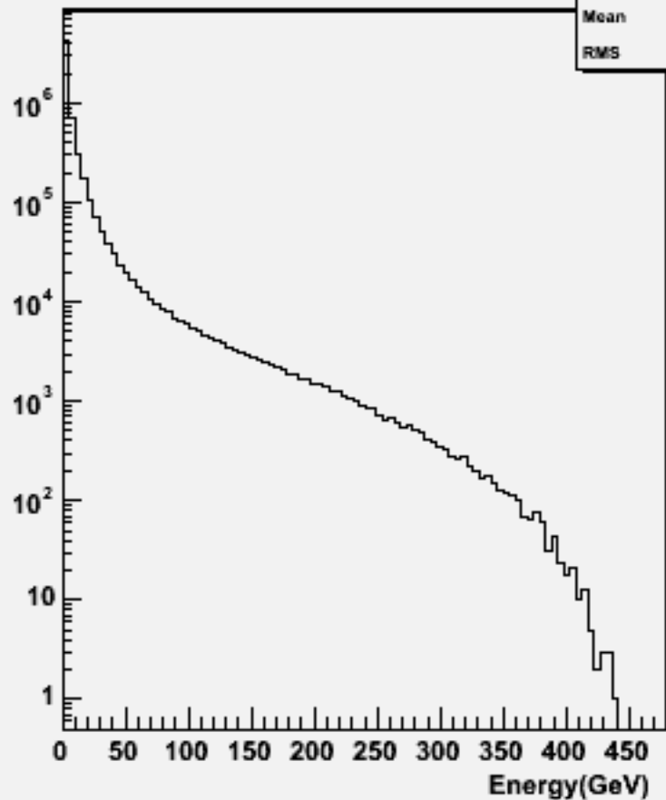
Start point R : p106147 physsim-ttz-2l2nbb_zqq
