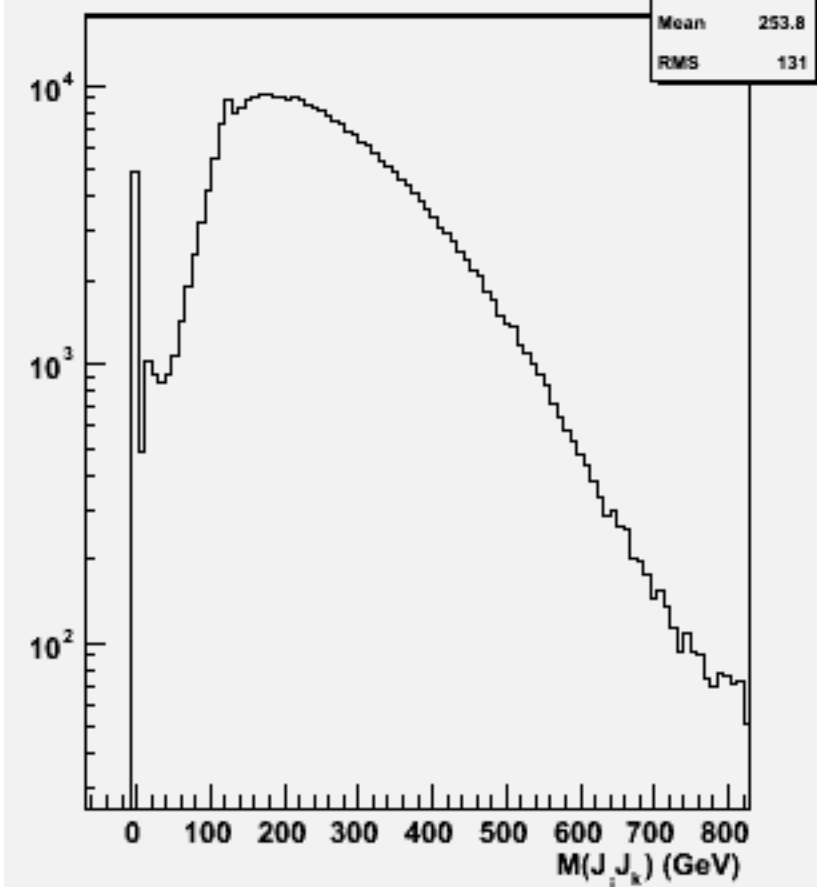
2jets mass(All comb)p106141 physsim-tth-2l2nbb_hbb
