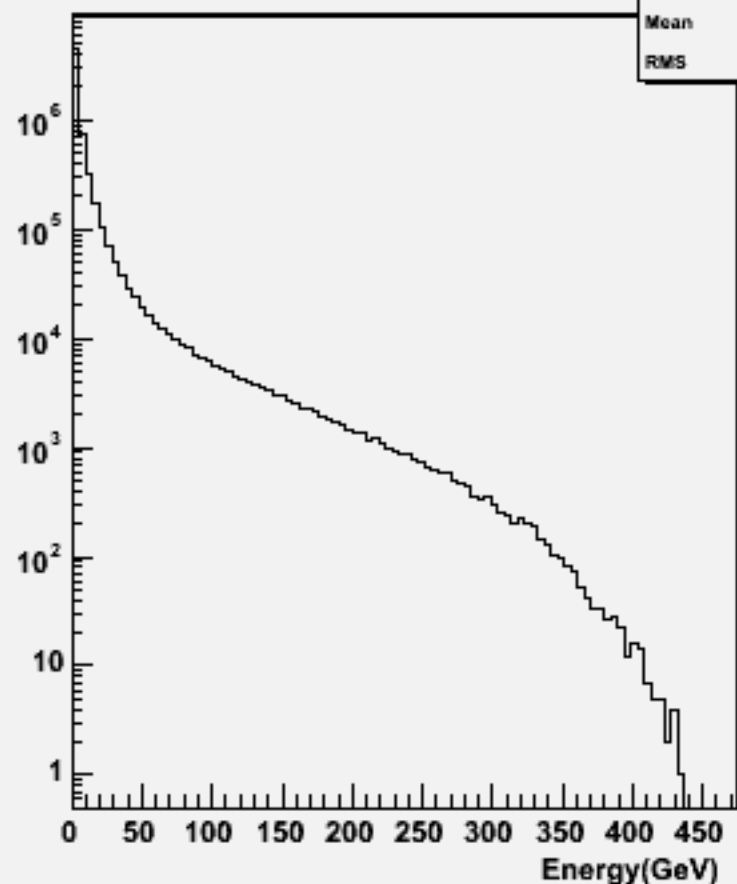
Start point R : p106141 physsim-tth-2l2nbb_hbb
