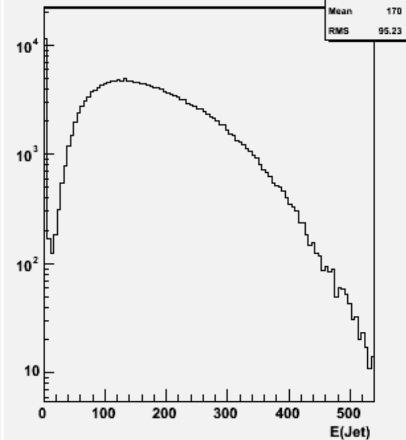
Jet energies(All jets)p106141 physsim-tth-2l2nbb_hbb
