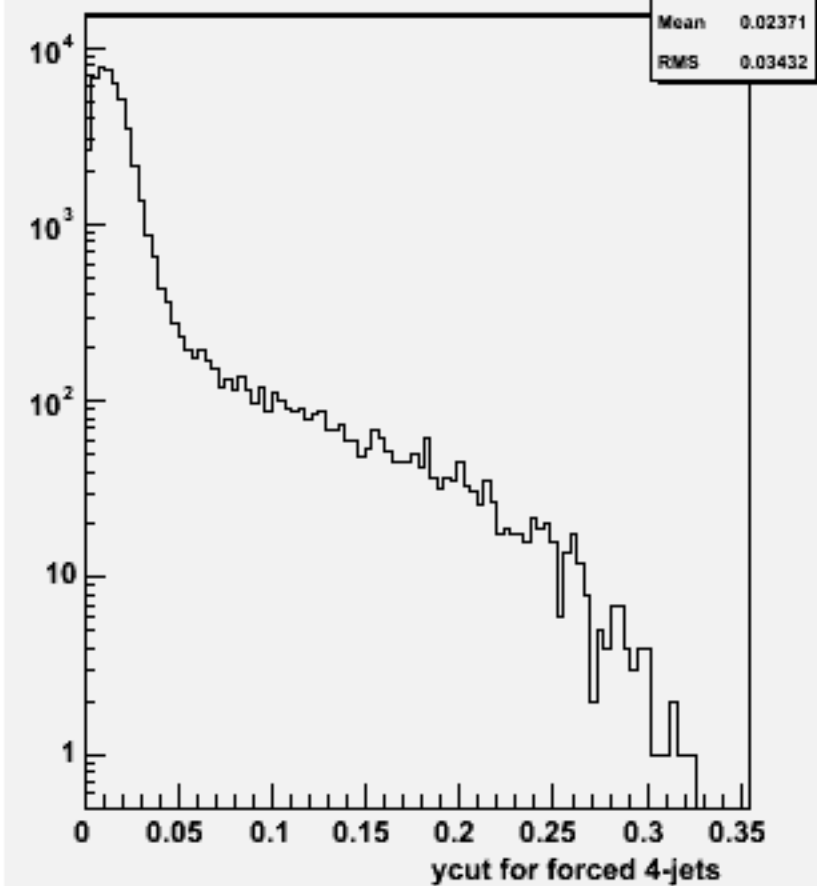
Ycut for 4-jets :p106141 physsim-tth-2l2nbb_hbb
