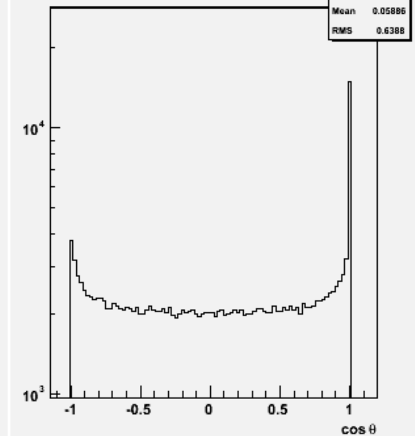
Jet cos \theta (All jets)p106141 physsim-tth-2l2nbb_hbb
