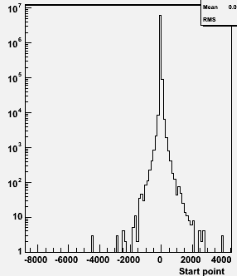
Start point Z : p106141 physsim-tth-2l2nbb_hbb
