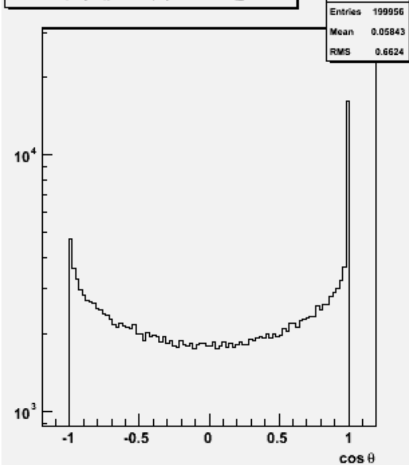
Jet cos \theta (All jets)p106140 physsim-ttz-ln4q_znn
