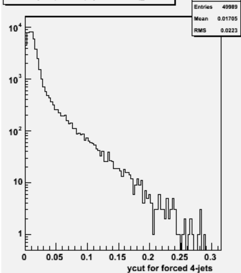
Ycut for 4-jets :p106140 physsim-ttz-ln4q_znn
