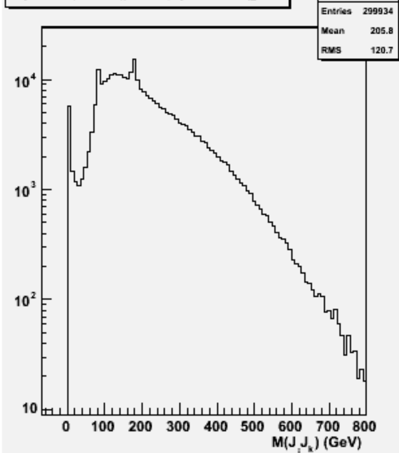
2jets mass(All comb)p106140 physsim-ttz-ln4q_znn
