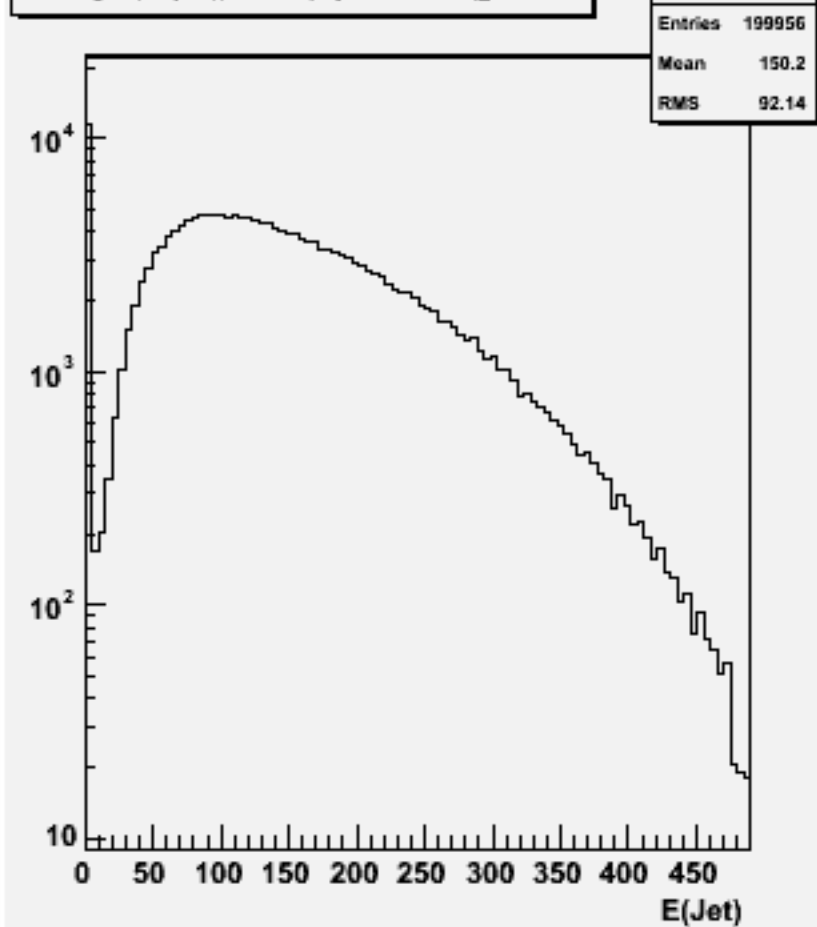
Jet energies(All jets)p106140 physsim-ttz-ln4q_znn
