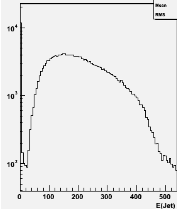
Jet energies(All jets)p106138 physsim-ttz-ln4q_zll
