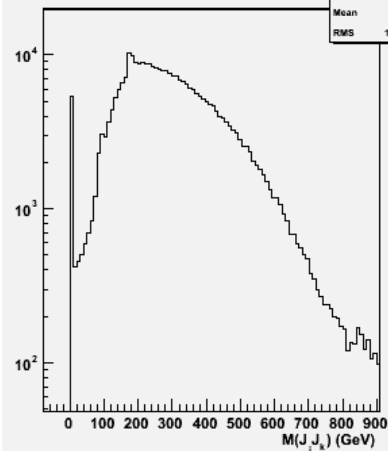
2jets mass(All comb)p106138 physsim-ttz-ln4q_zll
