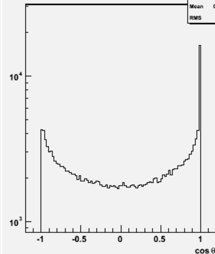
Jet cosθ (All jets)p106138 physsim-ttz-ln4q_zll
