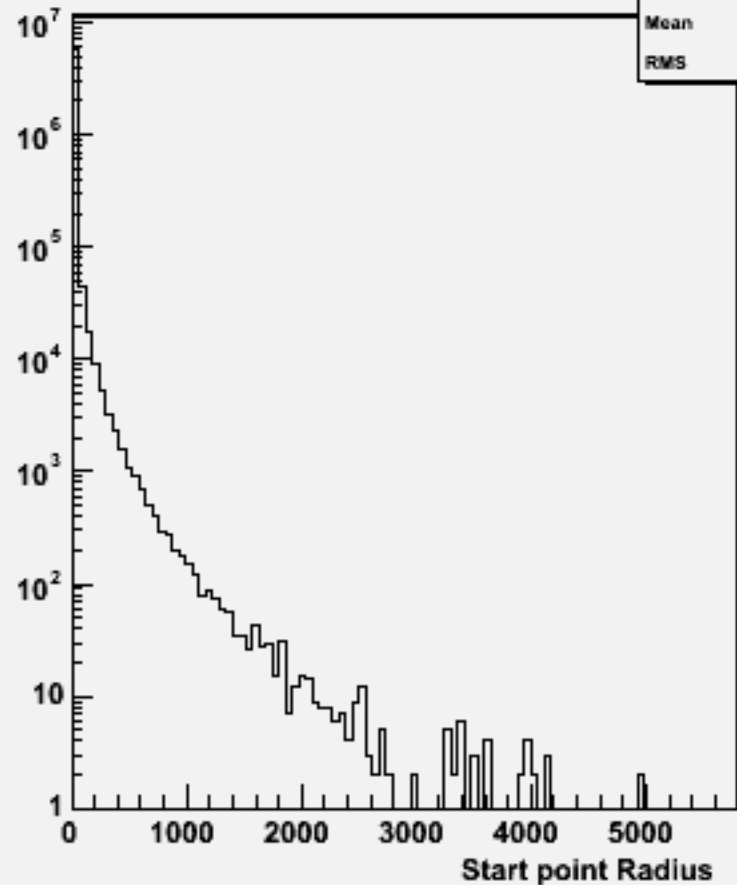
Start point R : p106138 physsim-ttz-ln4q_zll
