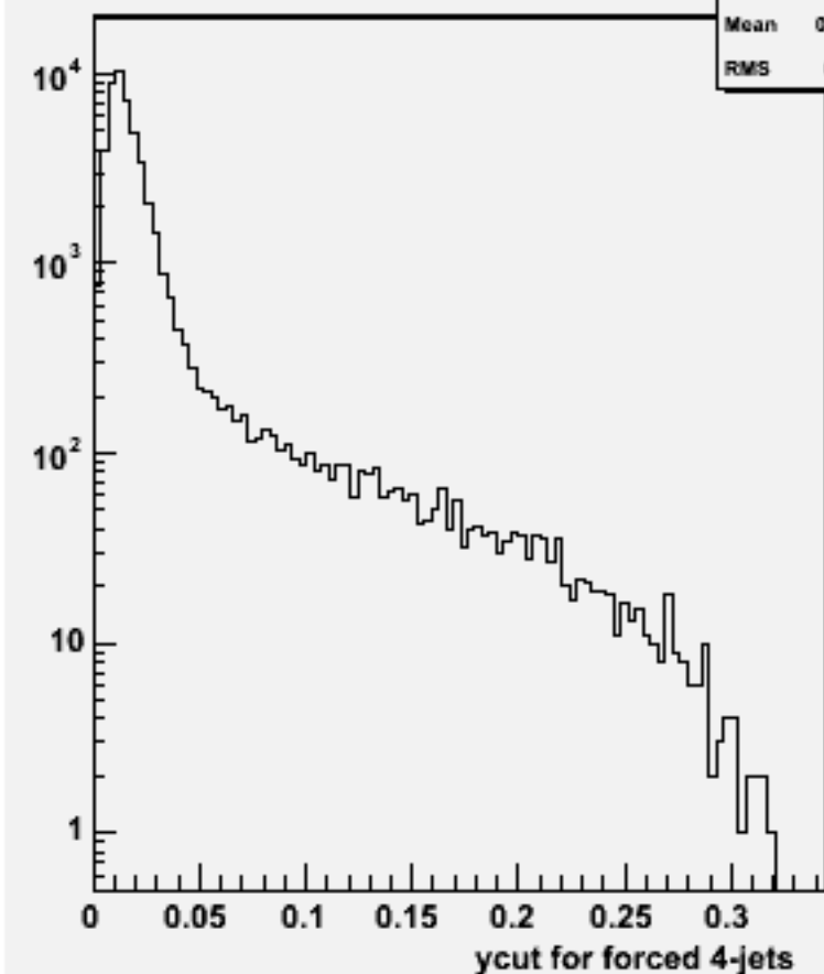
Ycut for 4-jets :p106138 physsim-ttz-ln4q_zll
