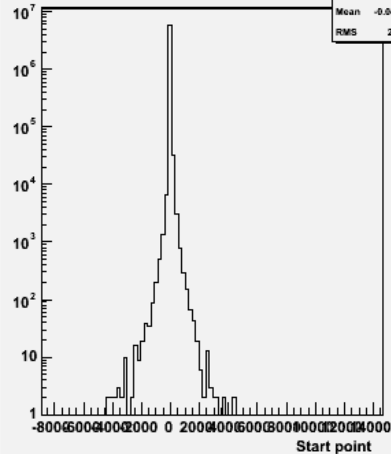
Start point Z : p106138 physsim-ttz-ln4q_zll
