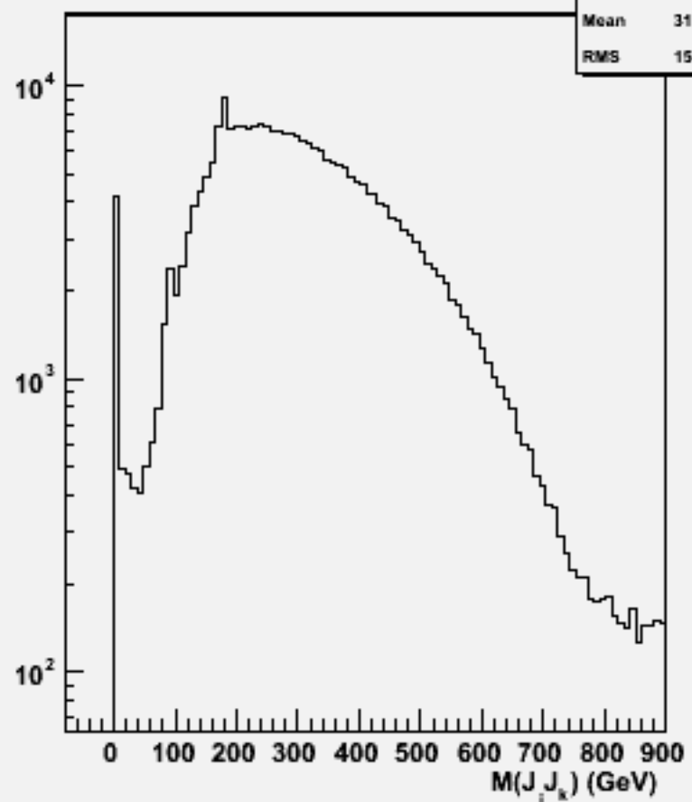
2jets mass(All comb)p106136 physsim-ttz-ln4q_zqq
