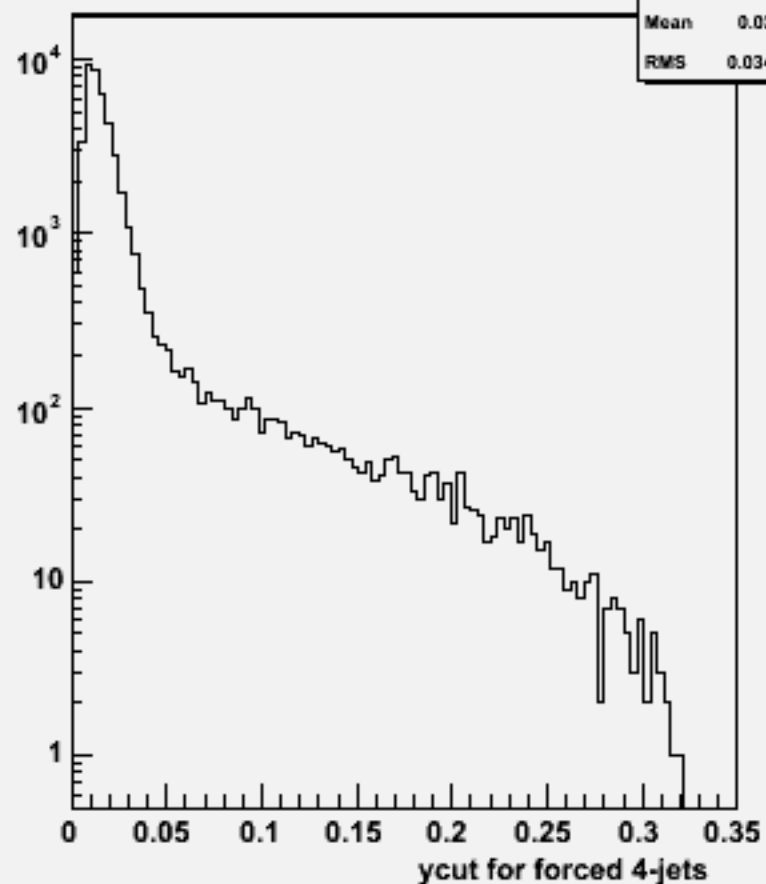
Ycut for 4-jets :p106136 physsim-ttz-ln4q_zqq
