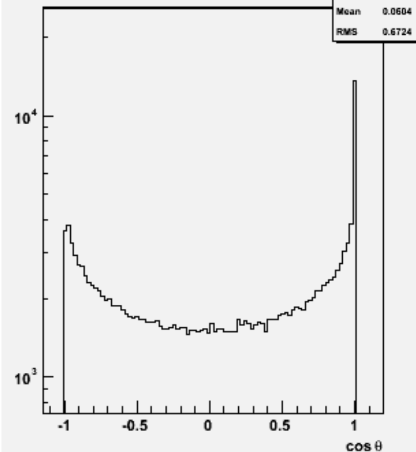
Jet cos \theta (All jets)p106136 physsim-ttz-ln4q_zqq
