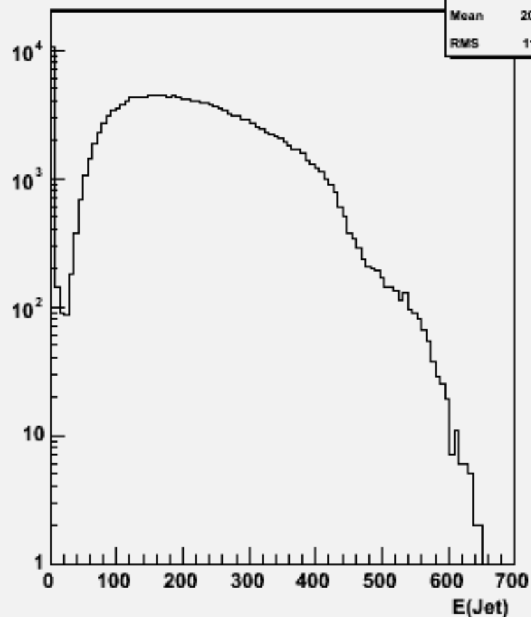
Jet energies(All jets)p106136 physsim-ttz-ln4q_zqq
