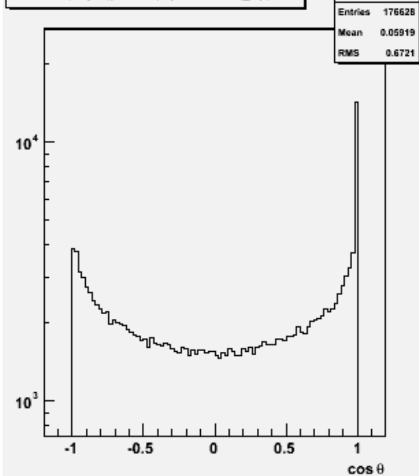
Jet cos \theta (All jets)p106135 physsim-ttz-ln4q_zqq
