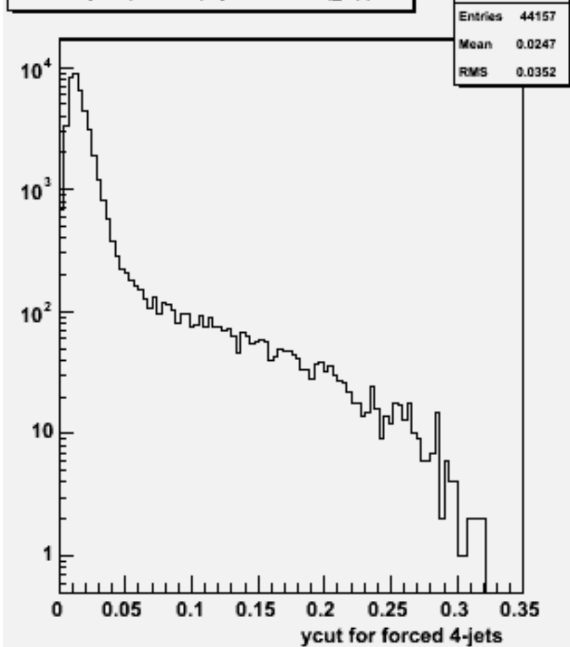
Ycut for 4-jets :p106135 physsim-ttz-ln4q_zqq
