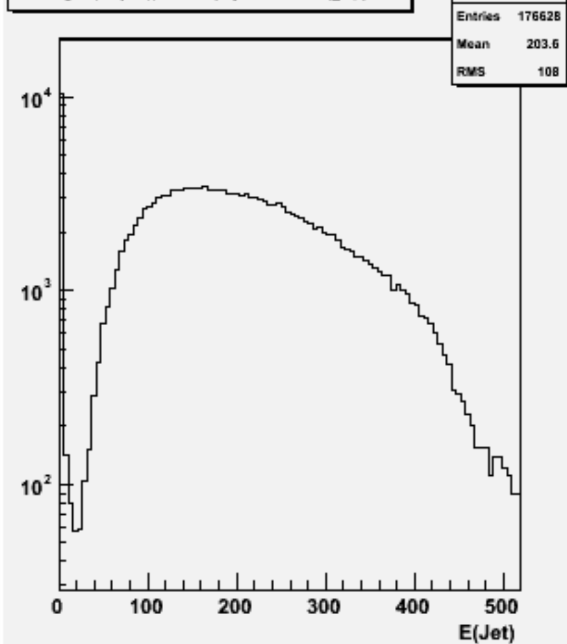
Jet energies(All jets)p106135 physsim-ttz-ln4q_zqq
