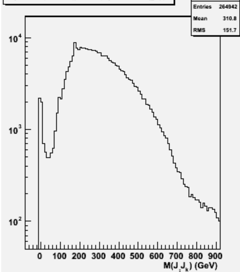
2jets mass(All comb)p106135 physsim-ttz-ln4q_zqq
