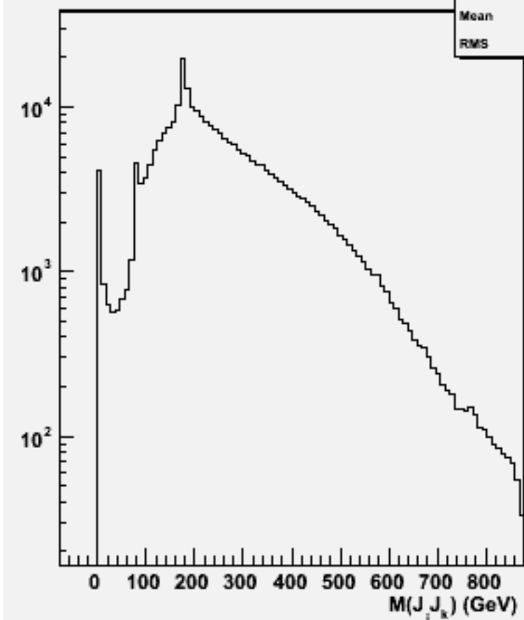
2jets mass(All comb)p106128 physsim-ttz-6q_znn
