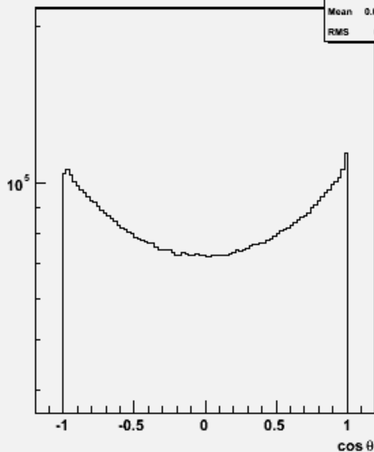
Particle cos \theta : p106128 physsim-ttz-6q_znn
