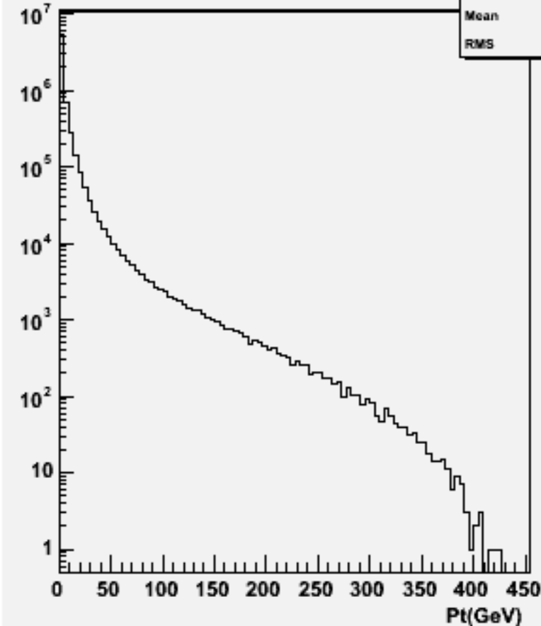
Start point Z : p106128 physsim-ttz-6q_znn
