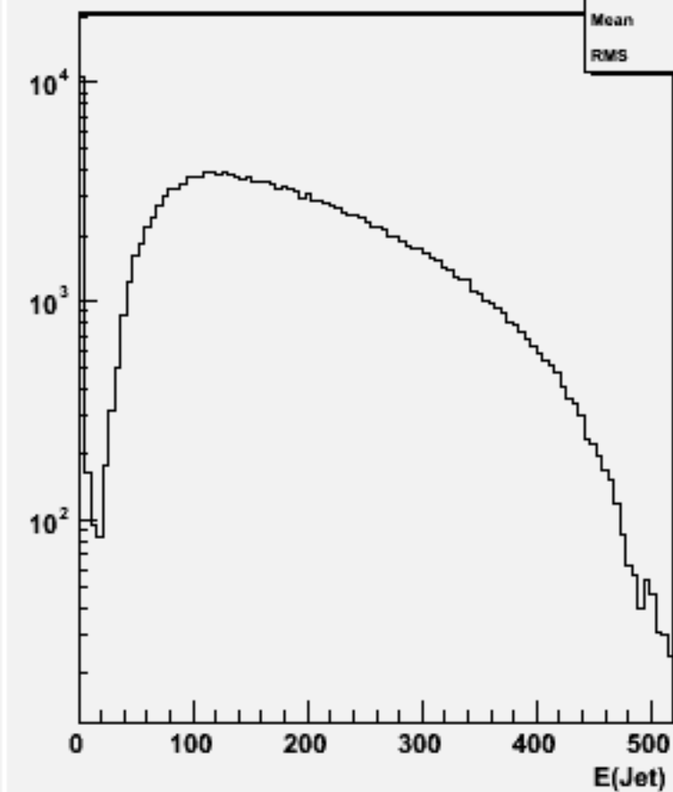
Jet energies(All jets)p106128 physsim-ttz-6q_znn
