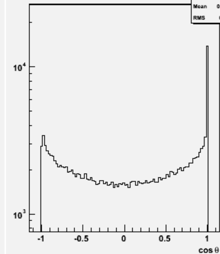
Jet cos \theta (All jets)p106128 physsim-ttz-6q_znn
