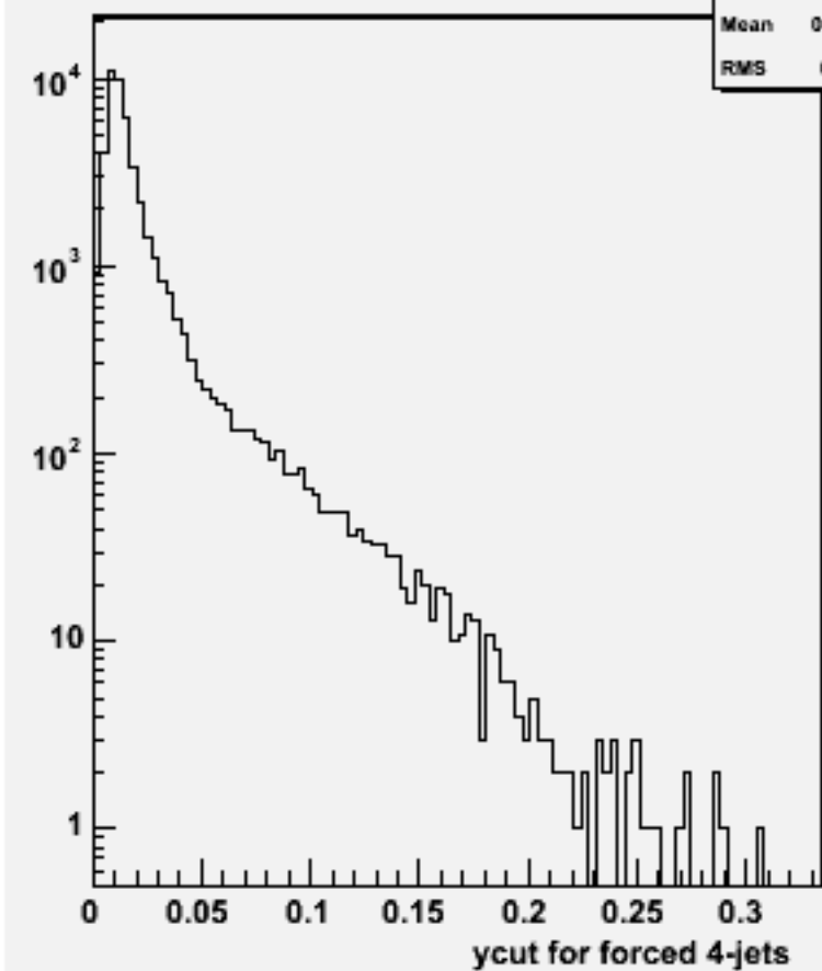
Ycut for 4-jets :p106128 physsim-ttz-6q_znn
