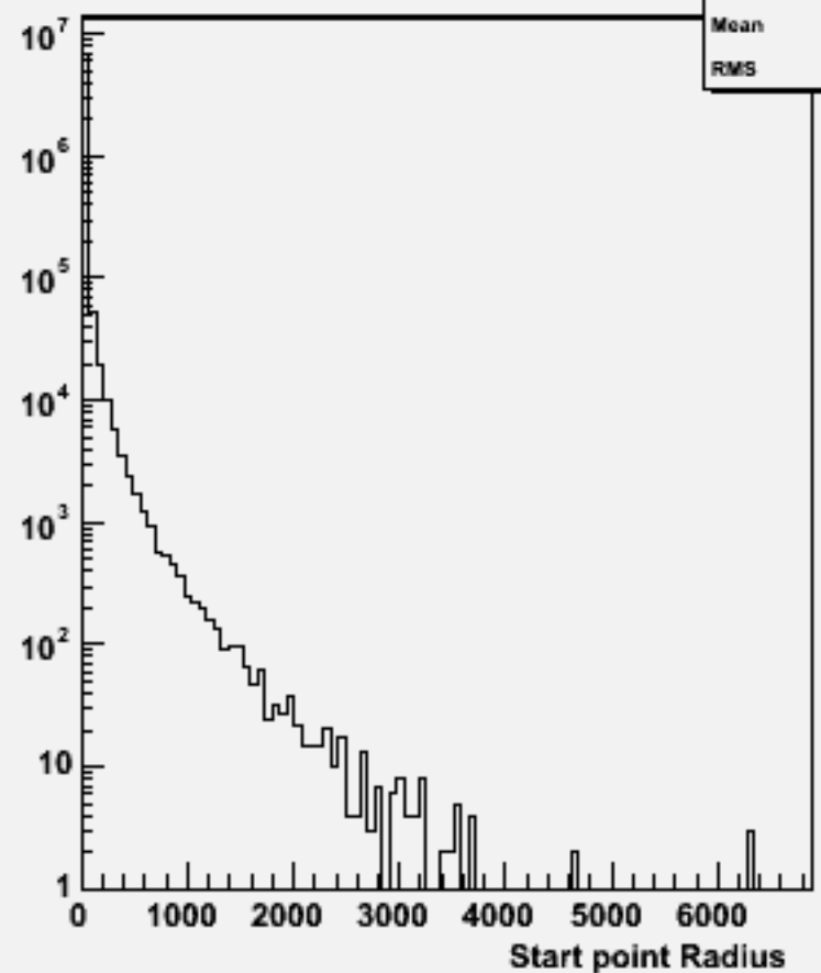
Start point R : p106128 physsim-ttz-6q_znn
