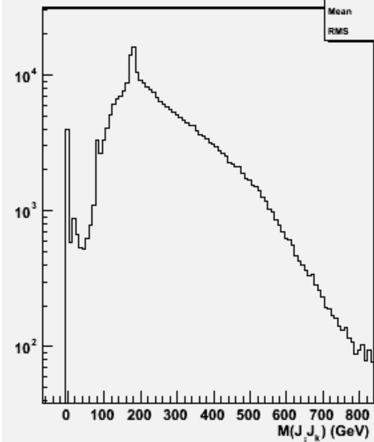
2jets mass(All comb)p106127 physsim-ttz-6q_znn
