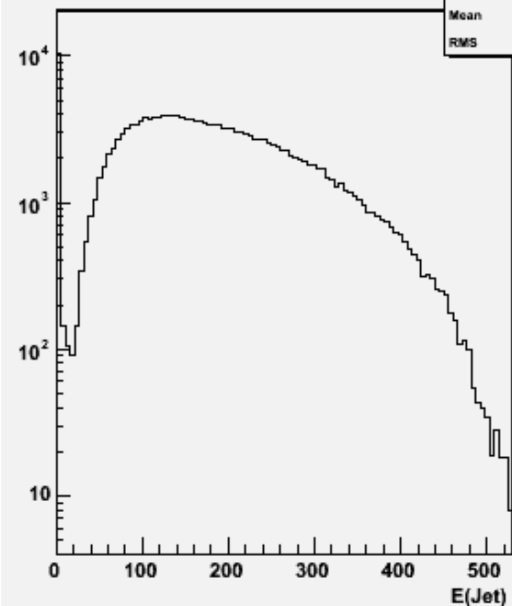
Jet energies(All jets)p106127 physsim-ttz-6q_znn
