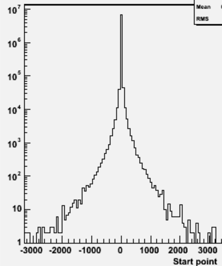
Start point Z : p106127 physsim-ttz-6q_znn
