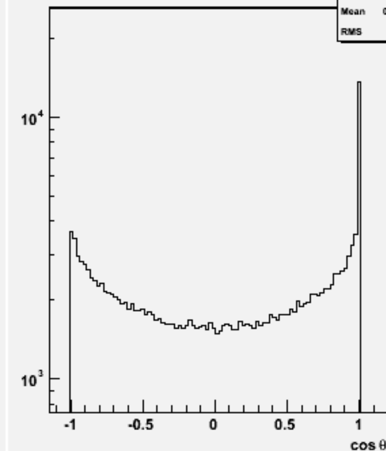
Jet cos \theta (All jets)p106127 physsim-ttz-6q_znn
