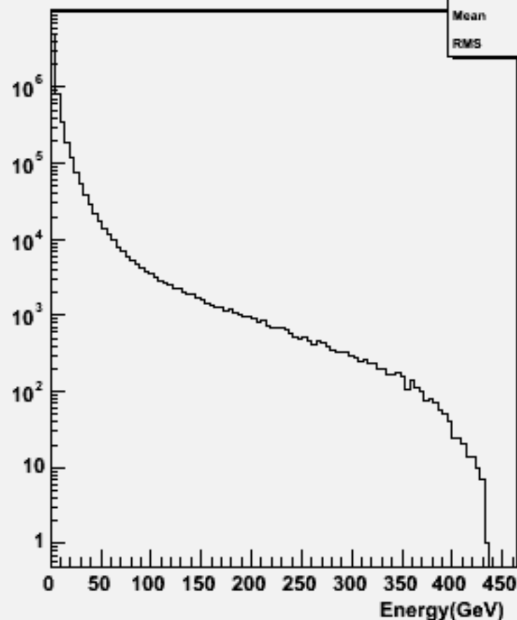
Start point R : p106127 physsim-ttz-6q_znn
