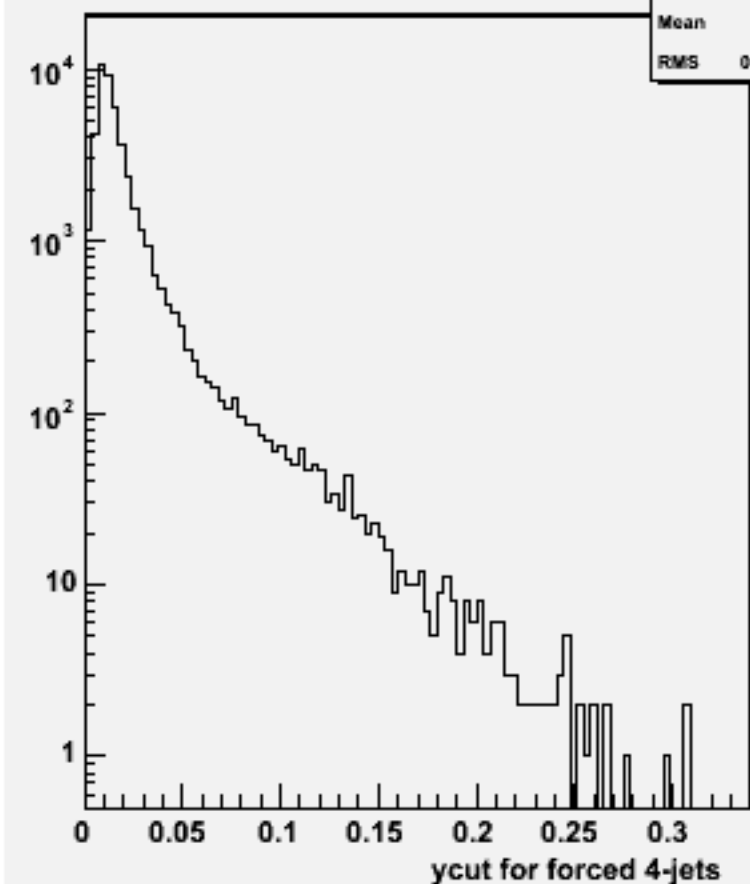
Ycut for 4-jets :p106127 physsim-ttz-6q_znn
