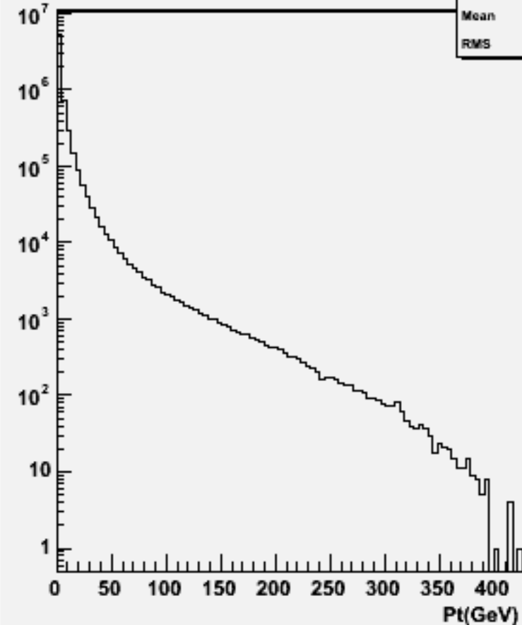
Start point Z : p106127 physsim-ttz-6q_znn
