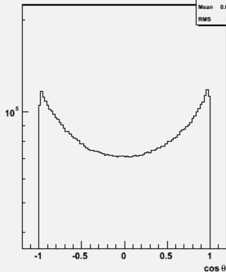
Particle cos \theta : p106124 physsim-ttz-6q_zqq
