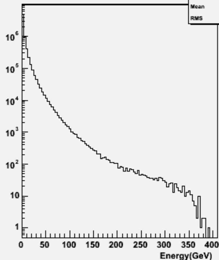
Start point R : p106124 physsim-ttz-6q_zqq
