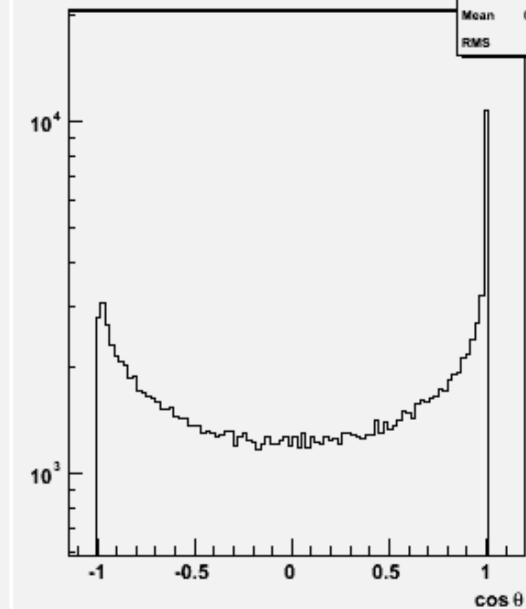
Jet cos \theta (All jets)p106124 physsim-ttz-6q_zqq
