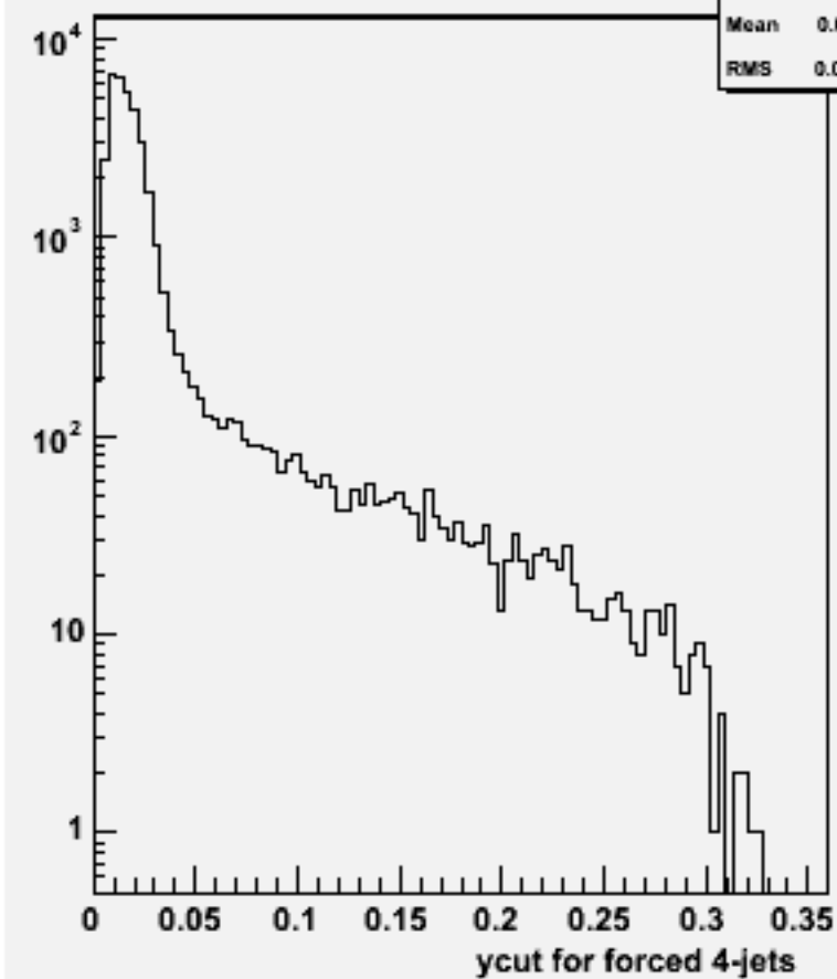
Ycut for 4-jets :p106124 physsim-ttz-6q_zqq
