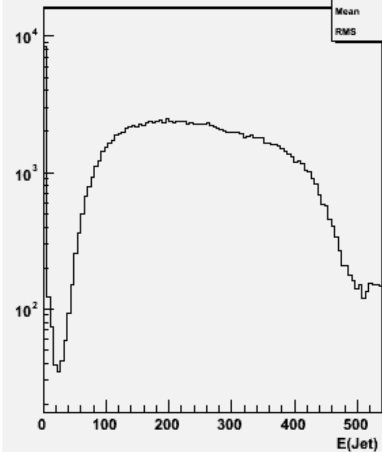
Jet energies(All jets)p106124 physsim-ttz-6q_zqq
