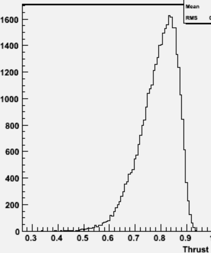
Thrust p106124 physsim-ttz-6q_zqq
