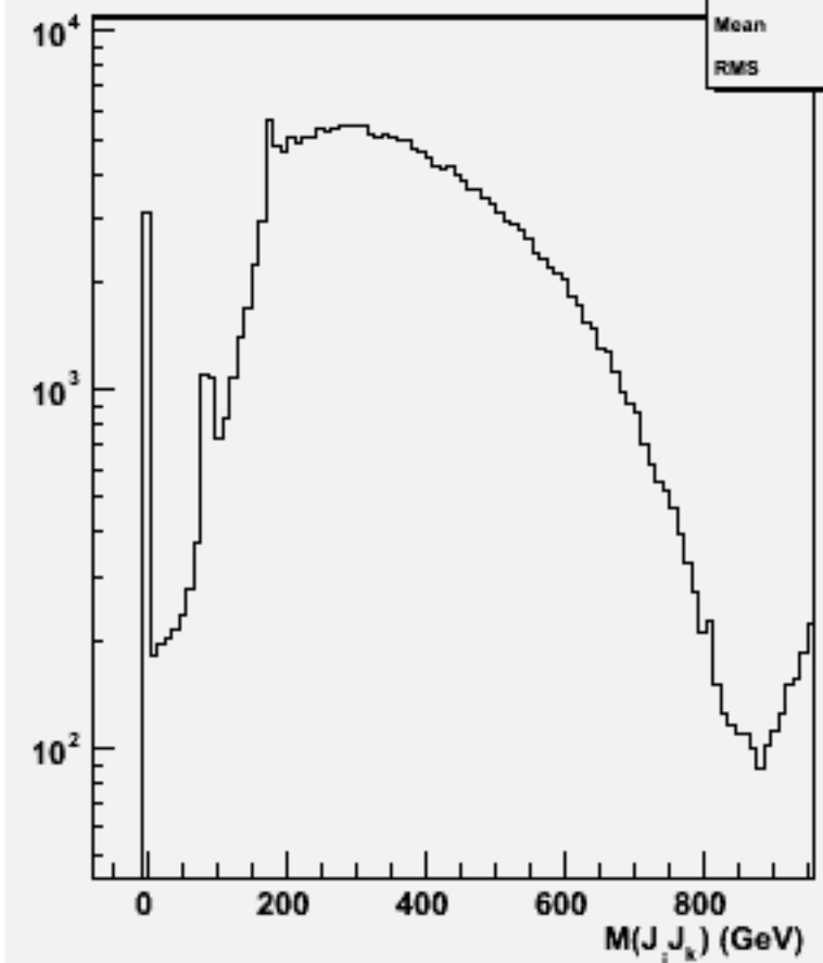
2jets mass(All comb)p106124 physsim-ttz-6q_zqq
