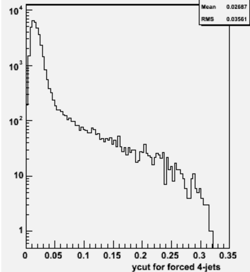
Ycut for 4-jets :p106119 physsim-tth-6q_hnonbb
