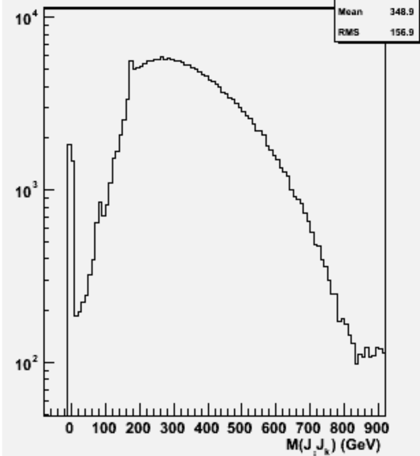
2jets mass(All comb)p106119 physsim-tth-6q_hnonbb
