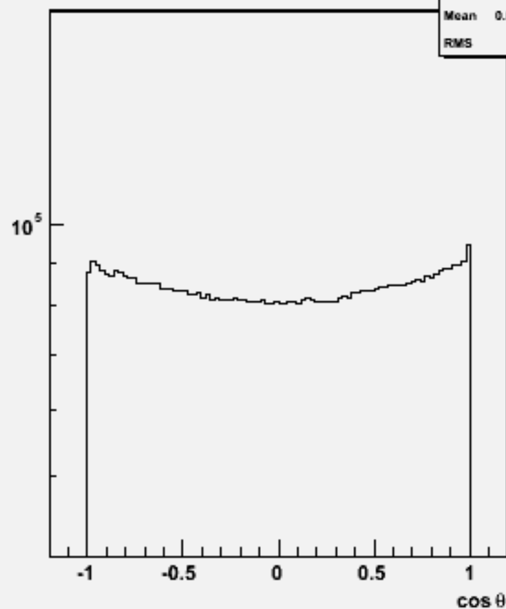
Particle cos \theta : p106119 physsim-tth-6q_hnonbb
