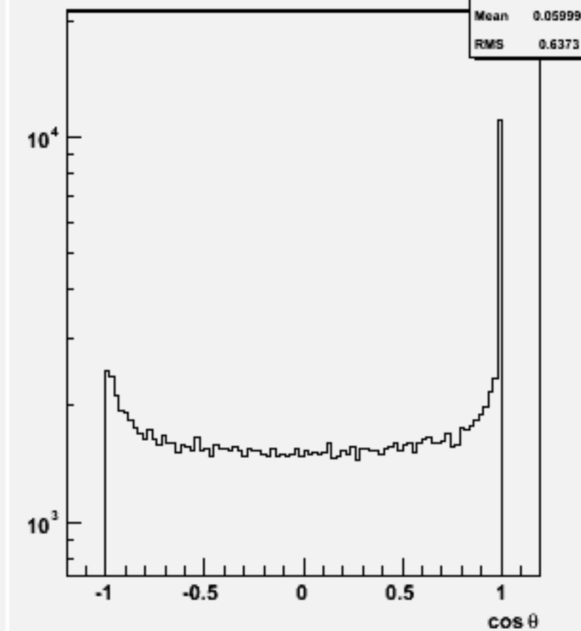
Jet cos \theta (All jets)p106119 physsim-tth-6q_hnonbb
