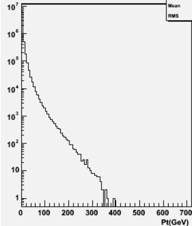
Particle Pt : p106119 physsim-tth-6q_hnonbb
