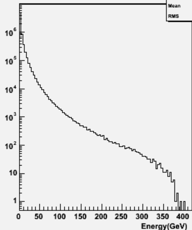
Particle Energy : p106119 physsim-tth-6q_hnonbb
