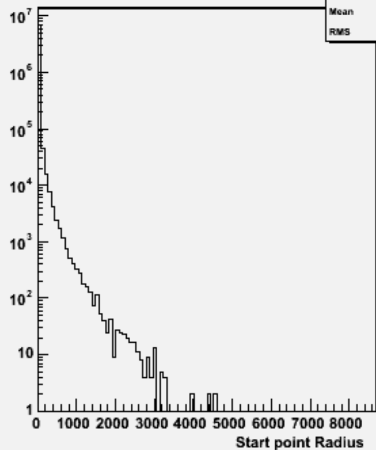
Start point R : p106119 physsim-tth-6q_hnonbb
