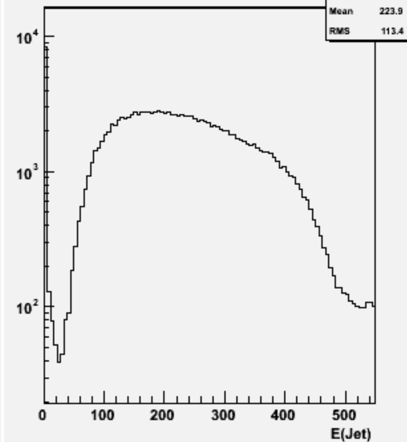
Jet energies(All jets)p106119 physsim-tth-6q_hnonbb
