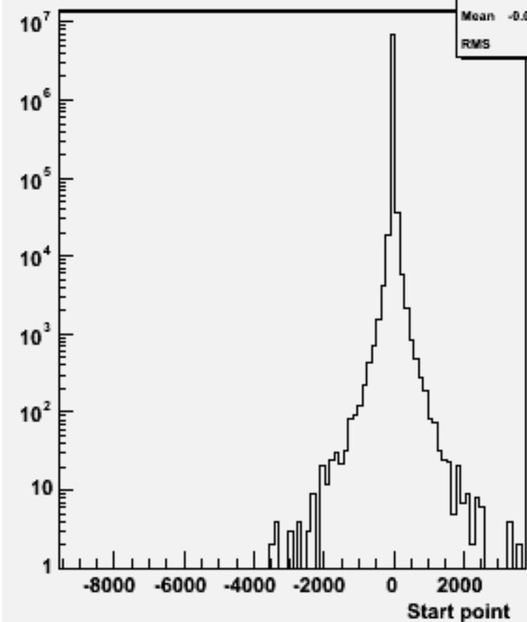
Start point Z : p106119 physsim-tth-6q_hnonbb
