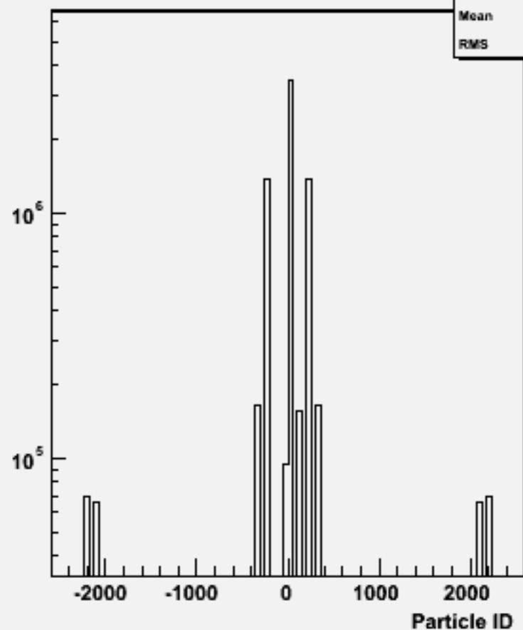
Particle ID : p106119 physsim-tth-6q_hnonbb
