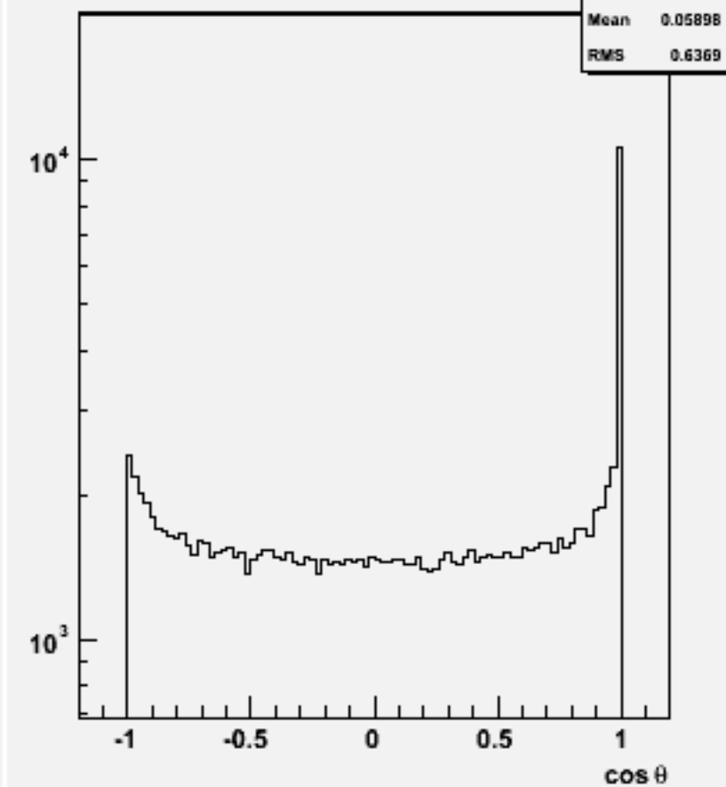
Jet cosθ (All jets)p106117 physsim-tth-6q_hbb
