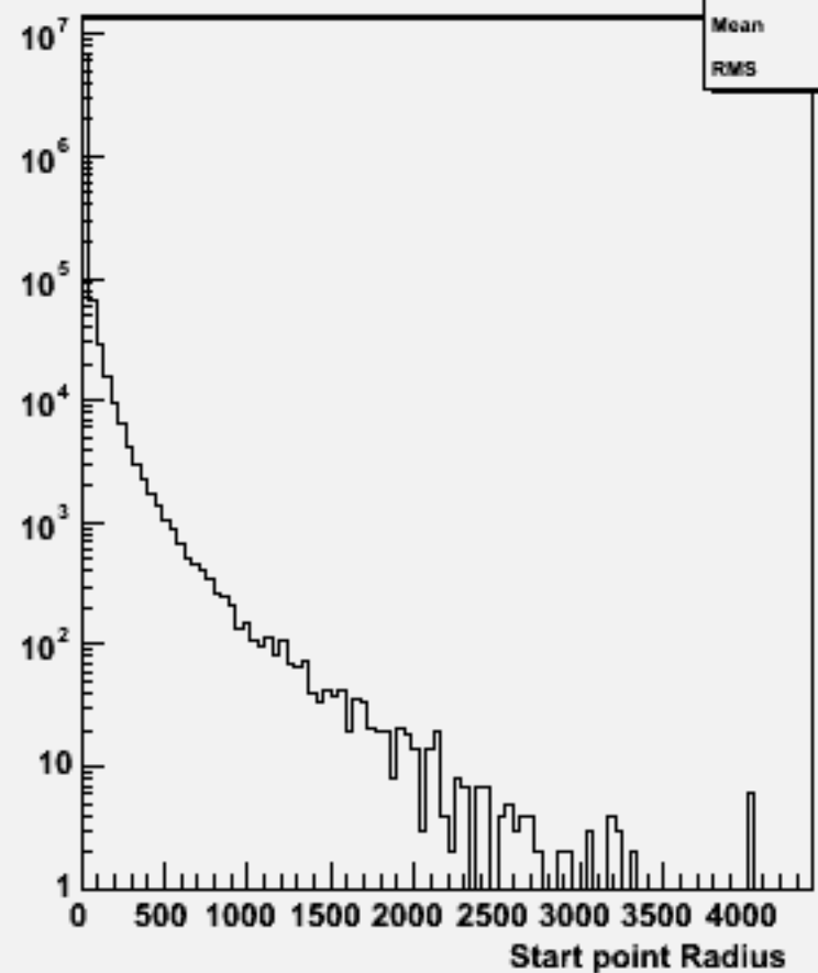
Start point R : p106117 physsim-tth-6q_hbb
