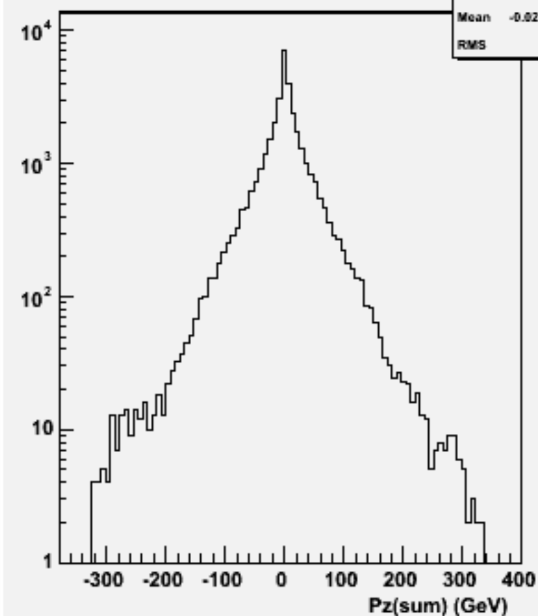
Pz Sum: p106117 physsim-tth-6q_hbb
