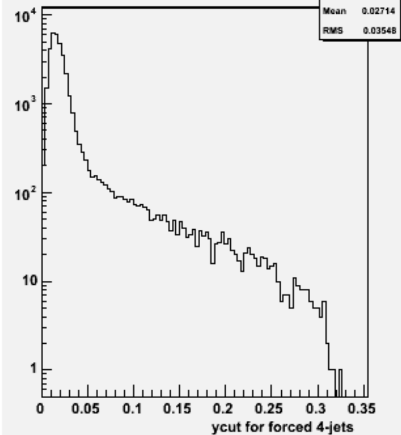
Ycut for 4-jets :p106117 physsim-tth-6q_hbb
