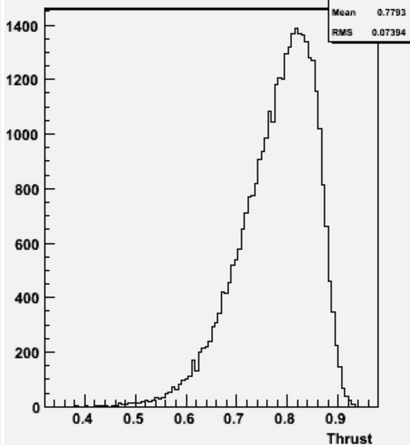
Thrust p106117 physsim-tth-6q_hbb
