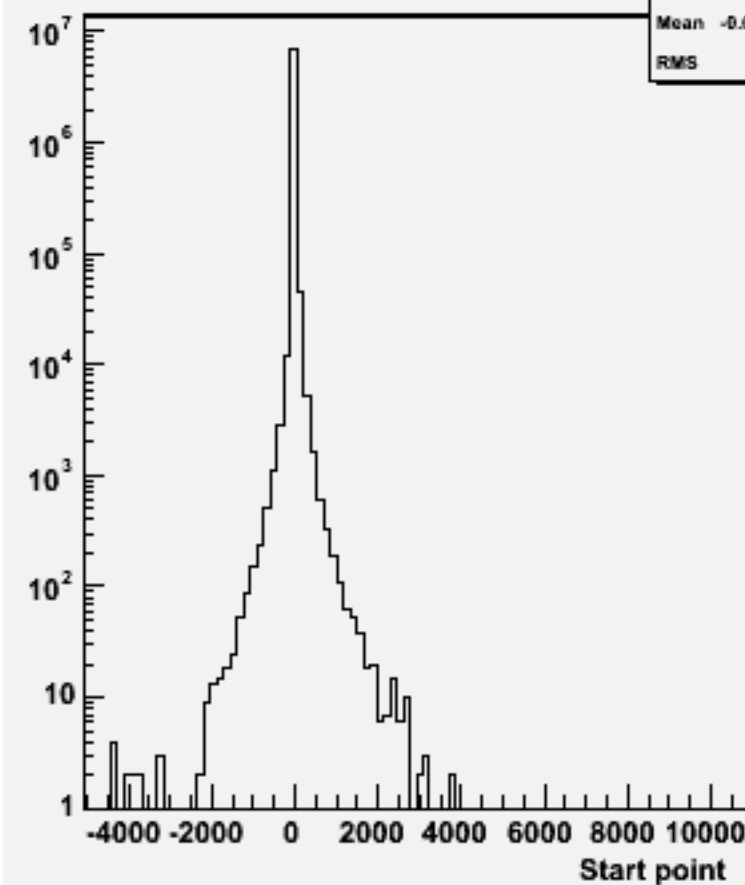
Start point Z : p106117 physsim-tth-6q_hbb
