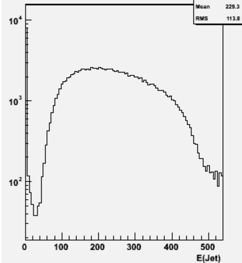
Jet energies(All jets)p106117 physsim-tth-6q_hbb
