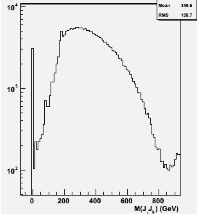
2jets mass(All comb)p106117 physsim-tth-6q_hbb
