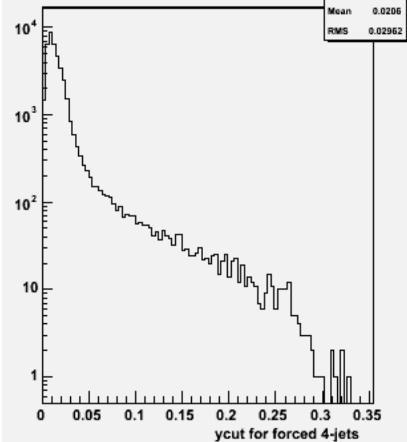
Ycut for 4-jets :p106114 physsim-ttbb-all_all
