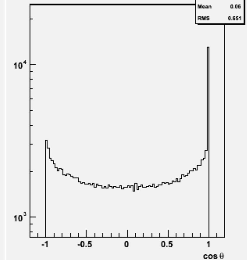
Jet cos \theta (All jets)p106114 physsim-ttbb-all_all
