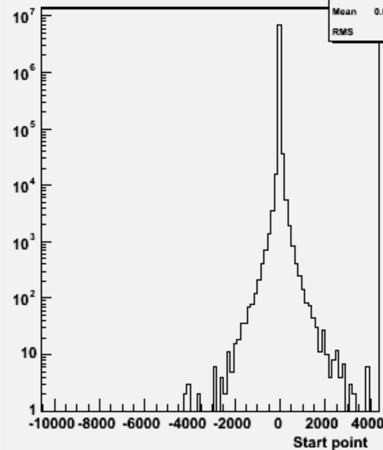
Start point Z : p106114 physsim-ttbb-all_all
