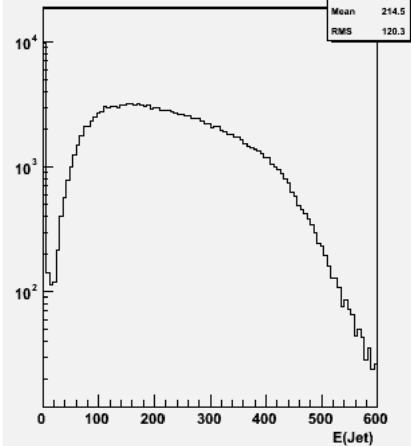
Jet energies(All jets)p106114 physsim-ttbb-all_all
