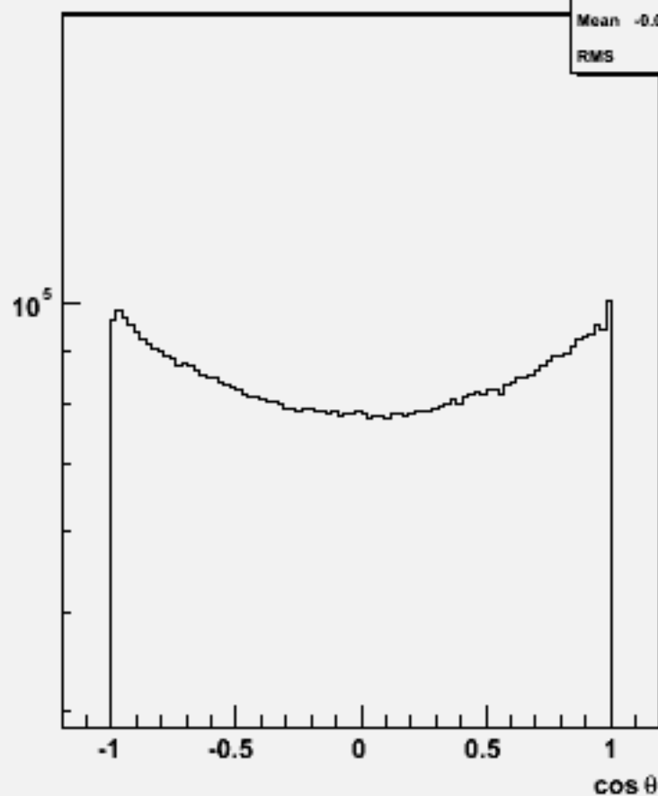
Particle cos \theta : p106114 physsim-ttbb-all_all
