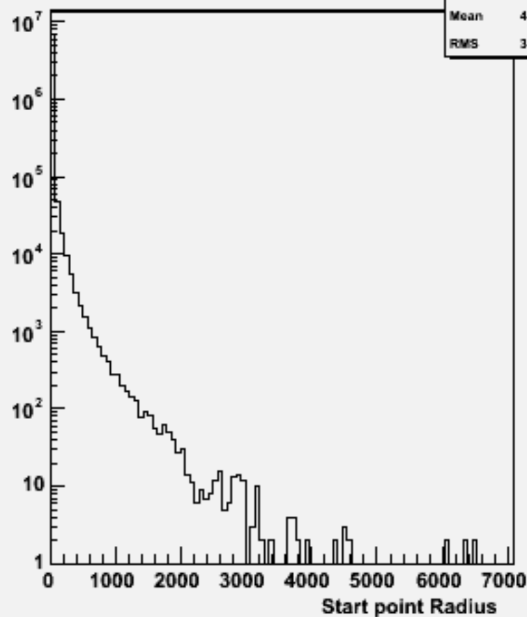
Start point R : p106114 physsim-ttbb-all_all
