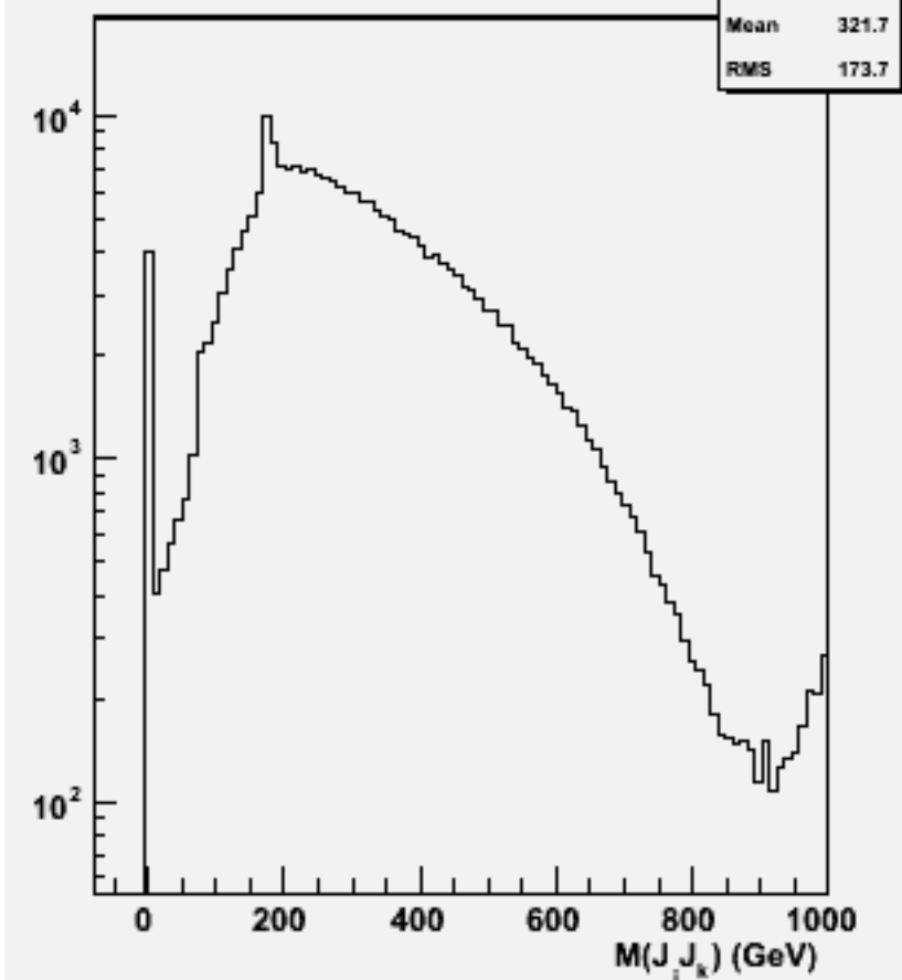
2jets mass(All comb)p106114 physsim-ttbb-all_all
