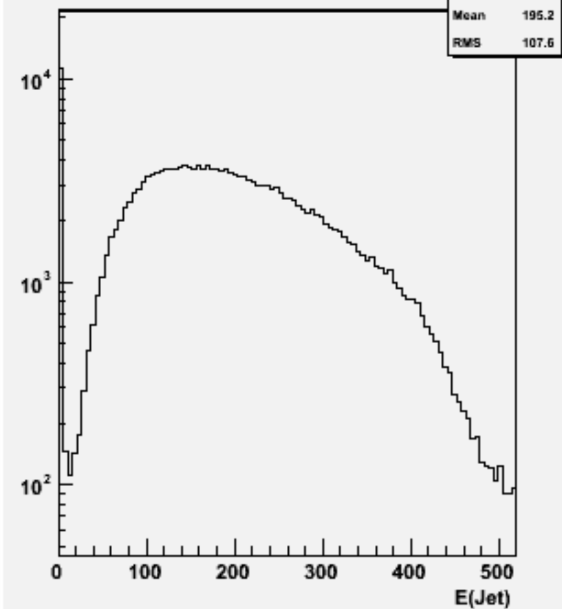
Jet energies(All jets)p106102 physsim-ttz-en4q_all
