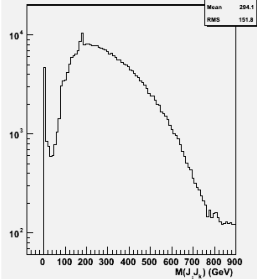
2jets mass(All comb)p106102 physsim-ttz-en4q_all
