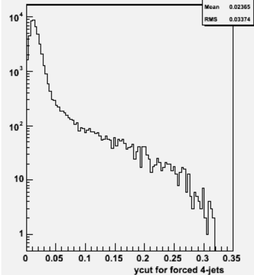
Ycut for 4-jets :p106102 physsim-ttz-en4q_all
