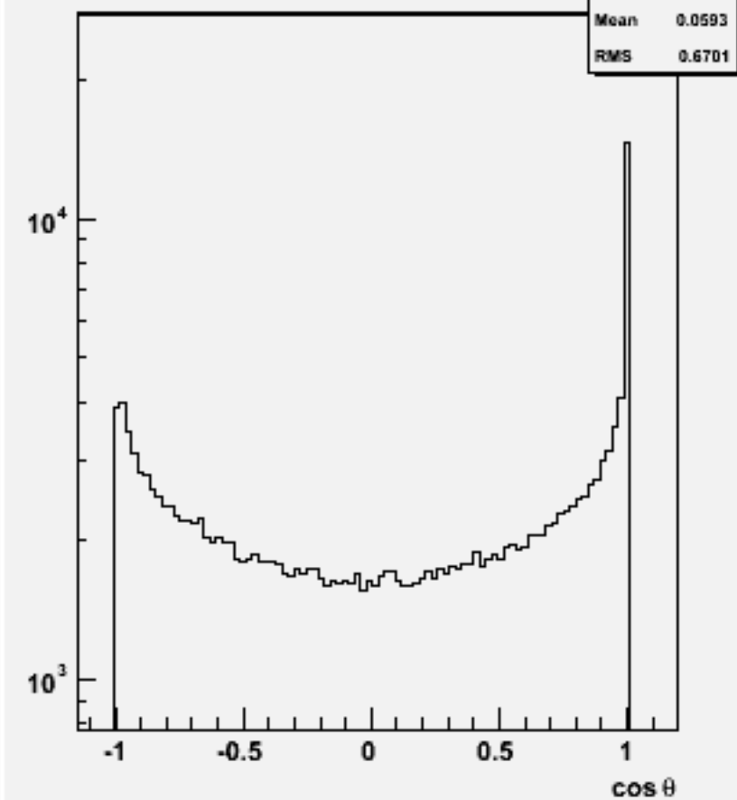
Jet cos \theta (All jets)p106102 physsim-ttz-en4q_all
