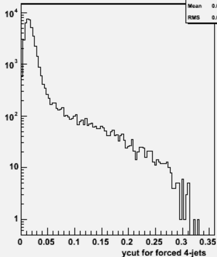
Ycut for 4-jets :p106101 physsim-tth-en4q_all
