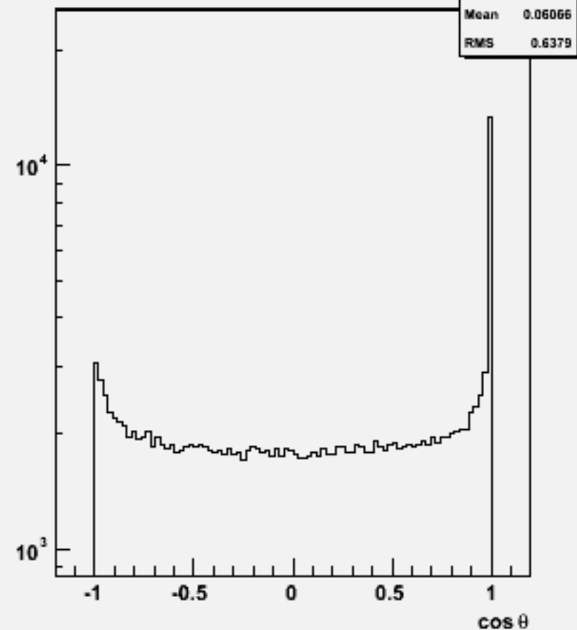
Jet cos \theta (All jets)p106101 physsim-tth-en4q_all
