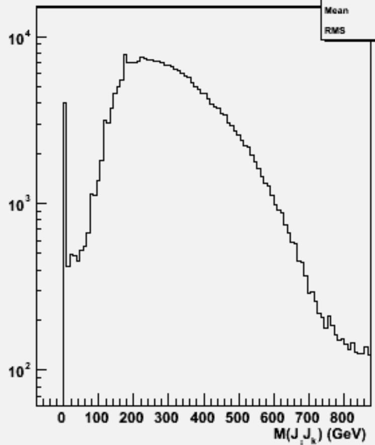
2jets mass(All comb)p106101 physsim-tth-en4q_all
