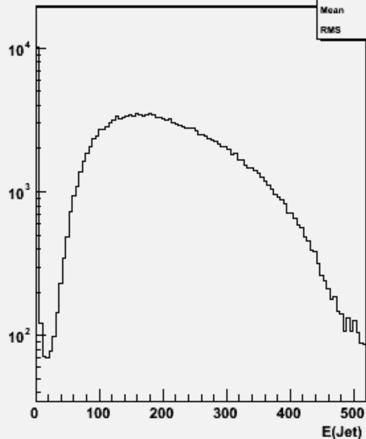
Jet energies(All jets)p106101 physsim-tth-en4q_all
