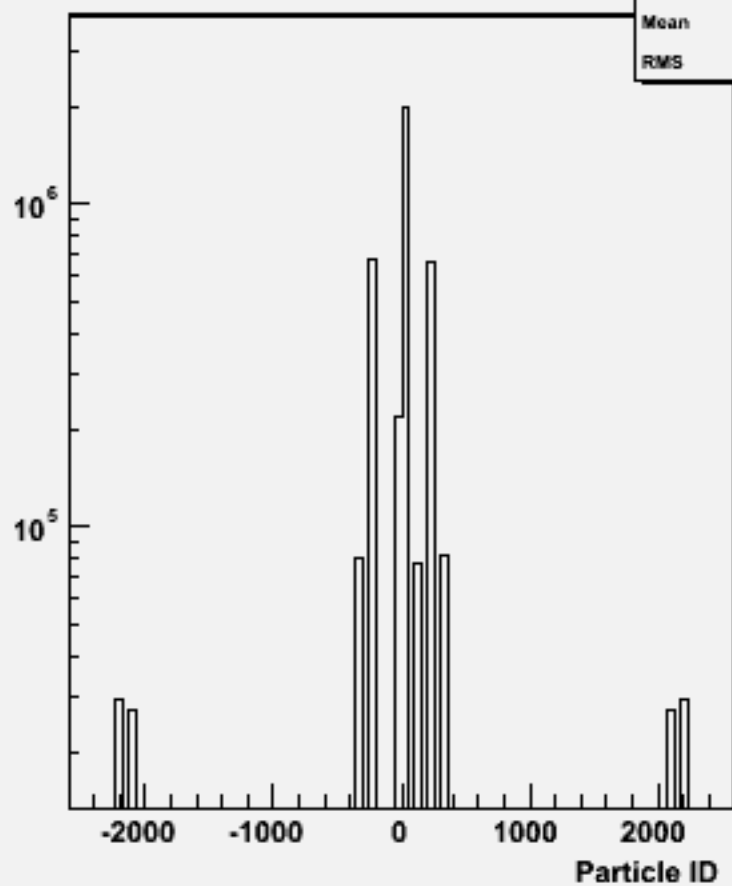
Particle ID : p106052 physsim-ttz-2l2nbb_znn
