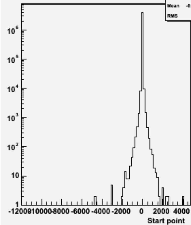
Start point Z : p106052 physsim-ttz-2l2nbb_znn
