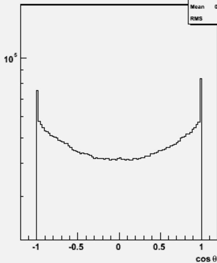
Particle cos \theta : p106052 physsim-ttz-2l2nbb_znn
