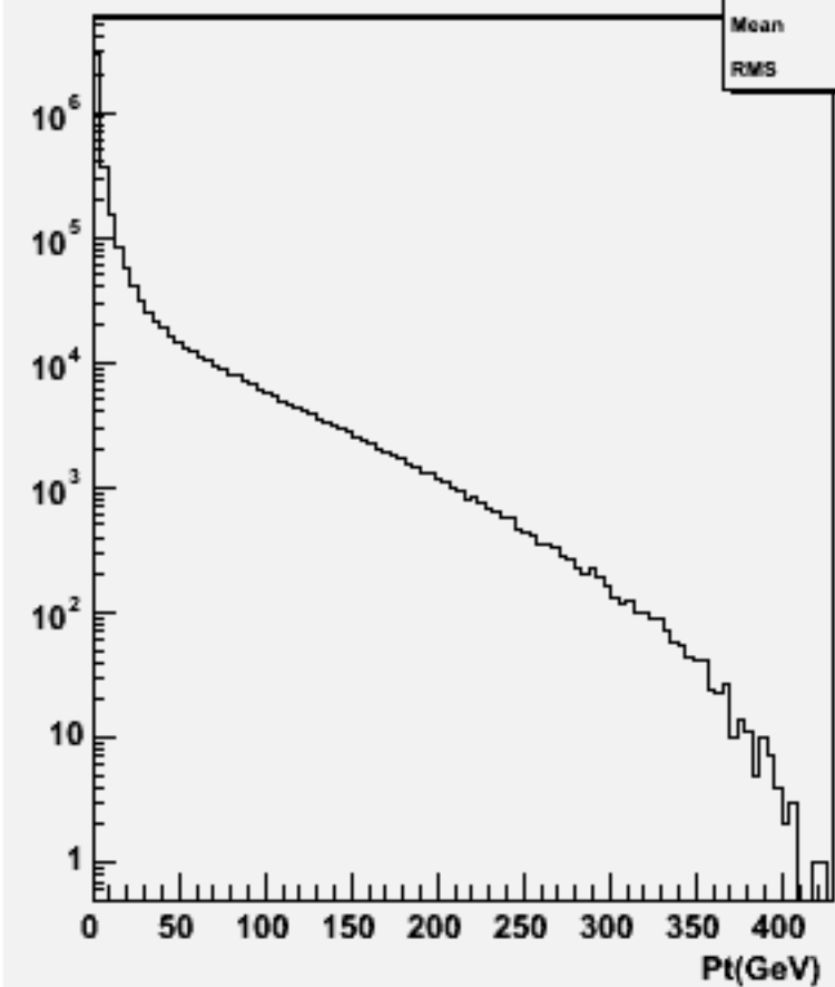
Particle Pt : p106052 physsim-ttz-2l2nbb_znn
