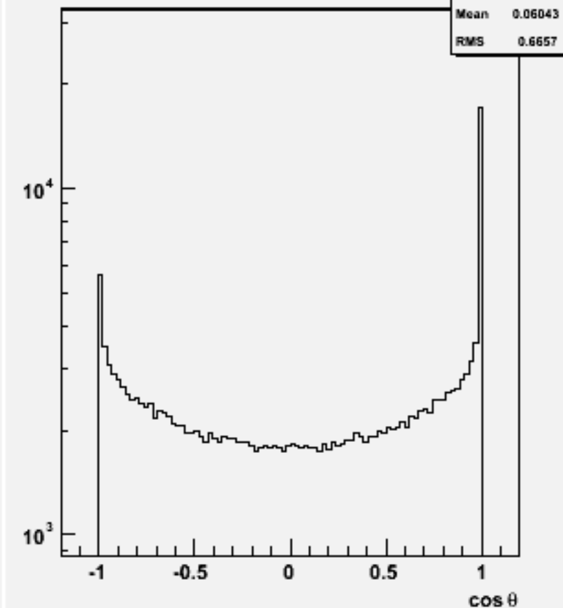
Jet cos \theta (All jets)p106052 physsim-ftz-2l2nbb_znn
