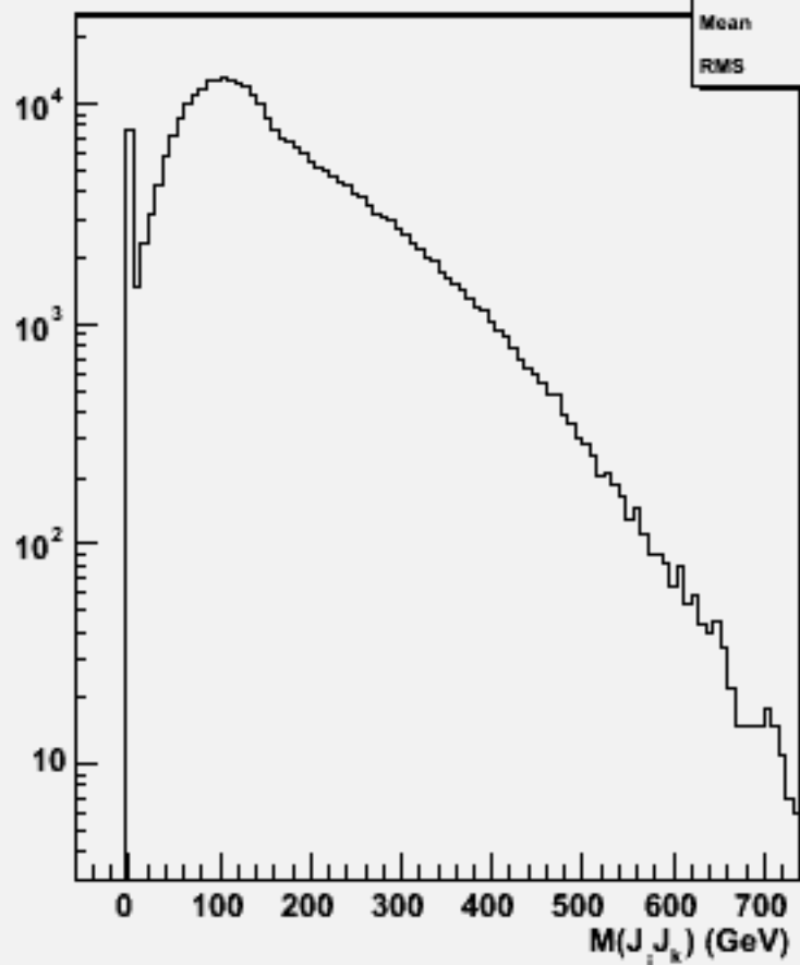
2jets mass(All comb)p106052 physsim-ftz-2l2nbb_znn
