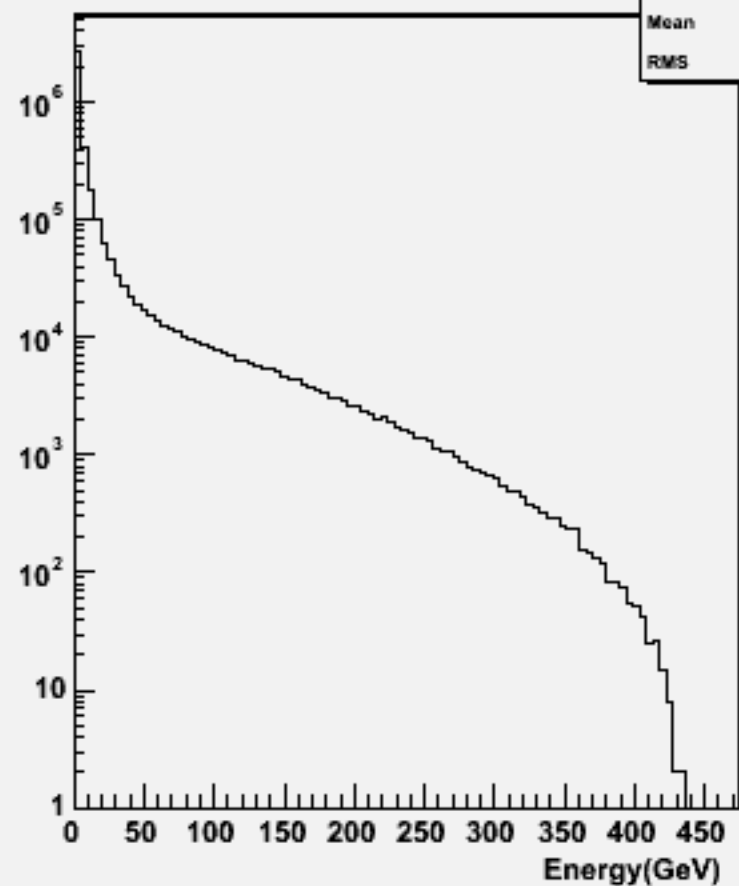
Particle Energy : p106052 physsim-ttz-2l2nbb_znn
