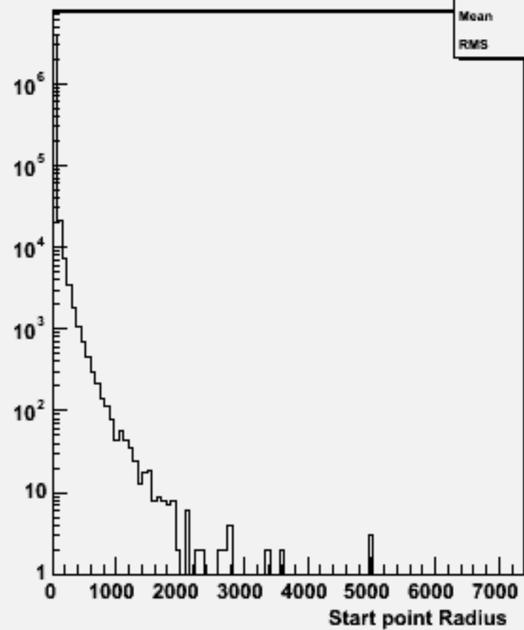
Start point R : p106052 physsim-ttz-2l2nbb_znn
