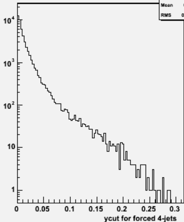
Ycut for 4-jets :p106052 physsim-ftz-2l2nbb_znn
