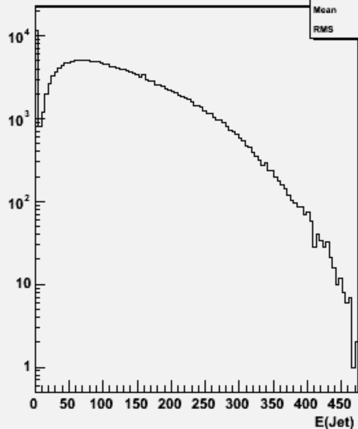
Jet energies(All jets)p106052 physsim-ftz-2l2nbb_znn
