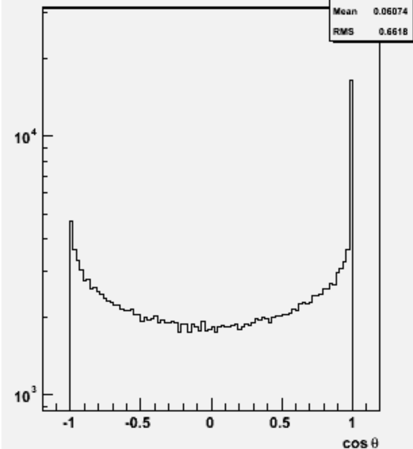
Jet cos \theta (All jets)p106040 physsim-ttz-ln4q_znn
