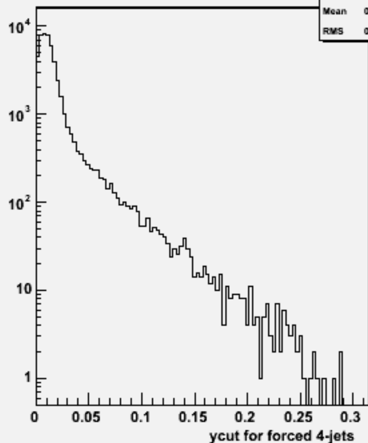
Ycut for 4-jets :p106040 physsim-ttz-ln4q_znn
