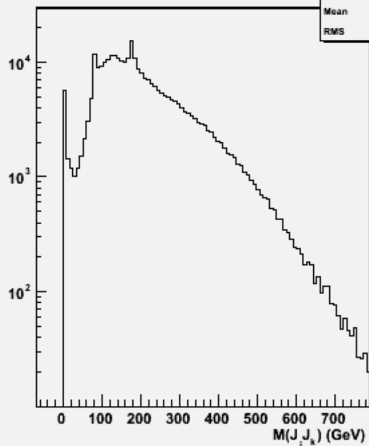
2jets mass(All comb)p106040 physsim-ttz-ln4q_znn
