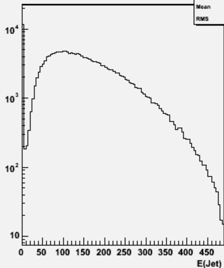
Jet energies(All jets)p106040 physsim-ttz-ln4q_znn
