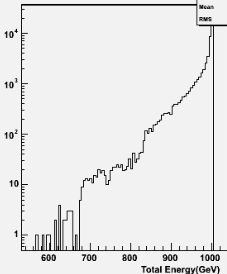
Total Energy (inc. \nu ): p106038 pyssim-ttz-ln4q_zll
