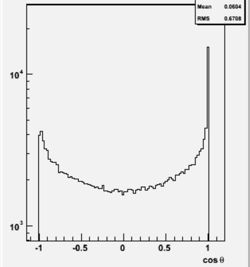
Jet cos(theta) (All jets)p106038 physsim-ttz-ln4q_zll
