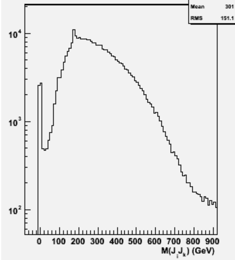
2jets mass(All comb)p106038 physsim-ttz-ln4q_zll
