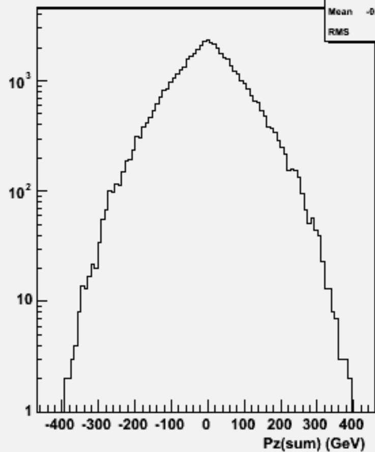
Pz Sum: p106038 pyssim-ttz-ln4q_zll
