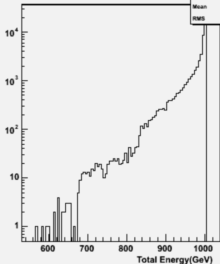
Total Energy (inc. \nu ): p106038 pyssim-ttz-ln4q_zll
