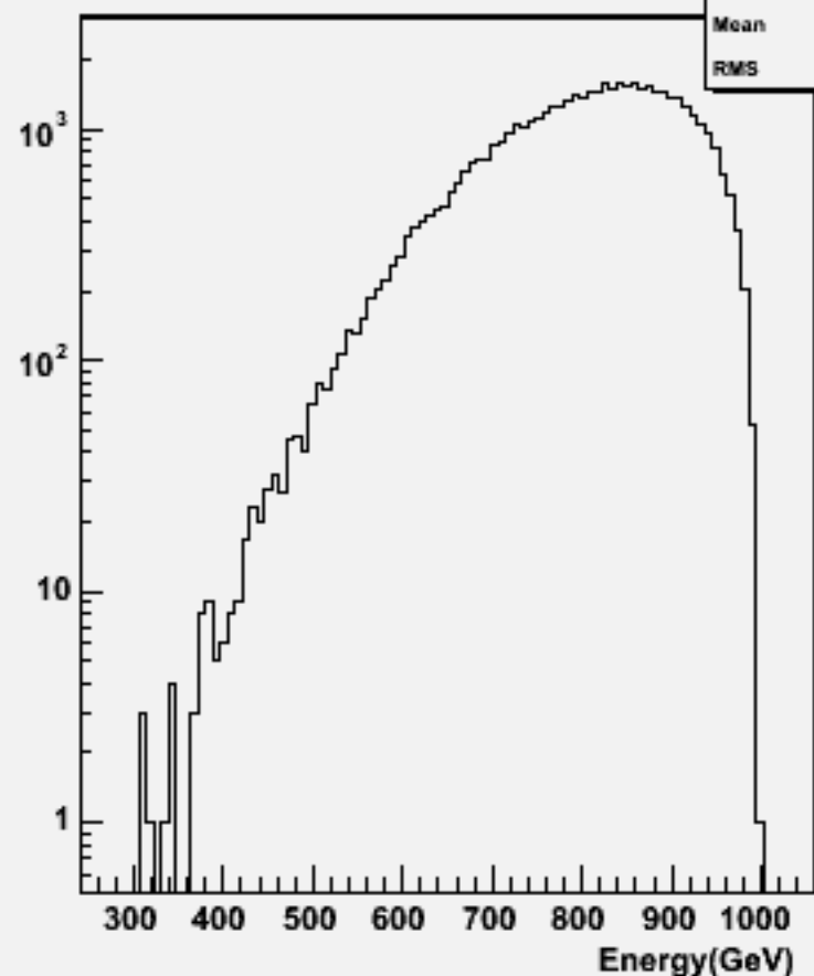
Total Energy (w/o \nu ): p106038 pyssim-ttz-ln4q_zll
