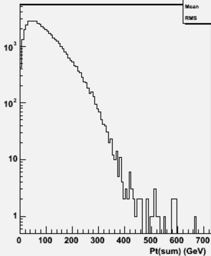
Pt Sum: p106038 pyssim-ttz-ln4q_zll
