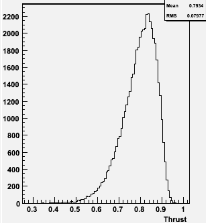
Thrust p106038 pyssim-ttz-ln4q_zll
