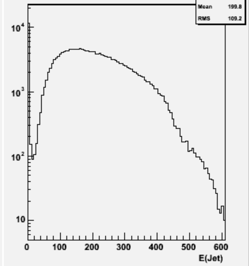
Jet energies(All jets)p106038 physsim-ttz-ln4q_zll
