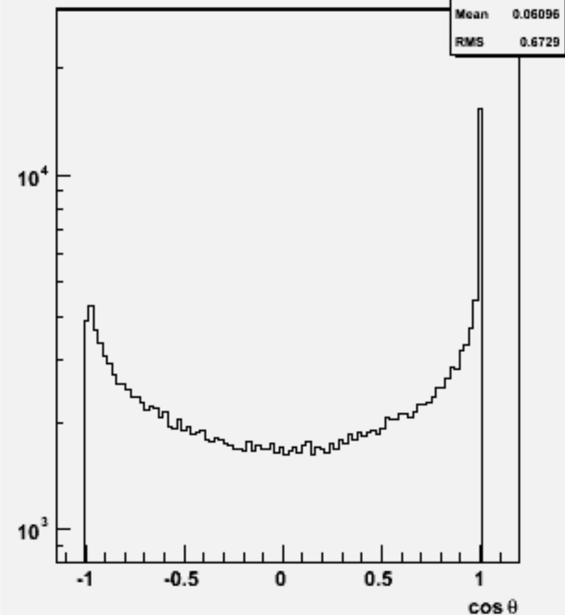
Jet cos \theta (All jets)p106035 physsim-ttz-ln4q_zqq
