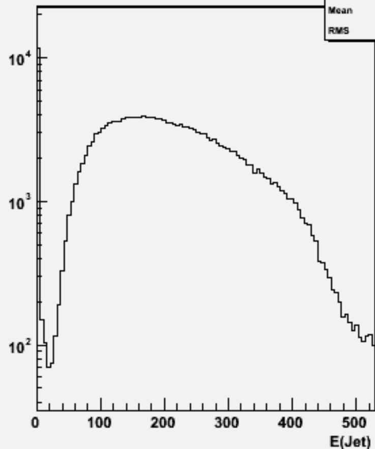
Jet energies(All jets)p106035 physsim-ttz-ln4q_zqq
