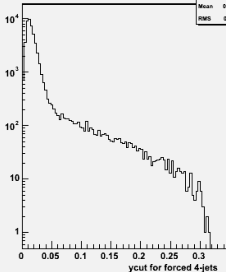
Ycut for 4-jets :p106035 physsim-ttz-ln4q_zqq
