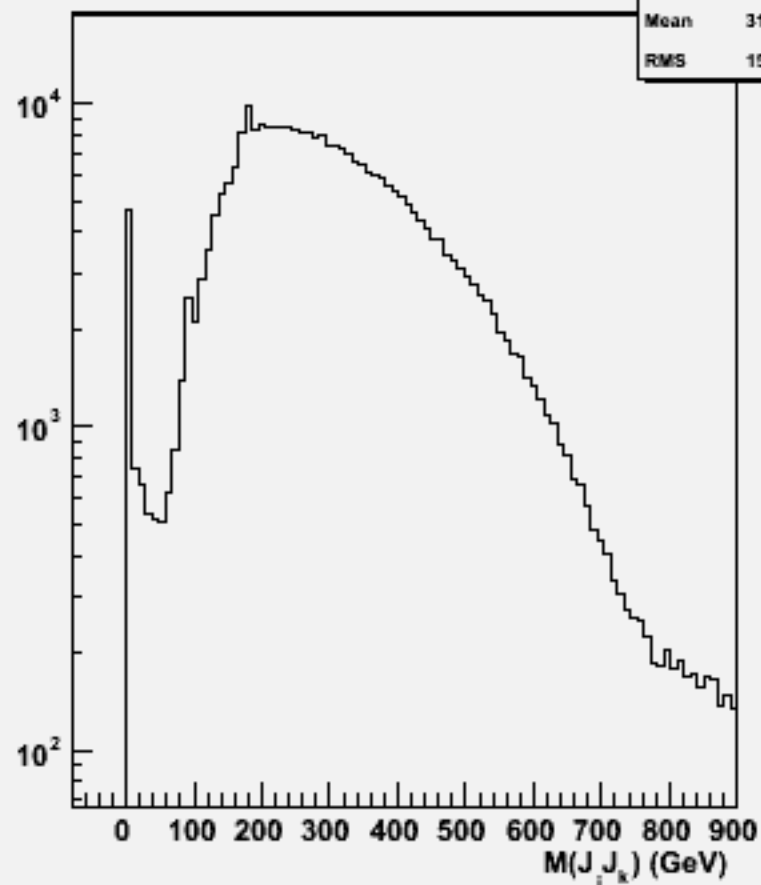
2jets mass(All comb)p106035 physsim-ttz-ln4q_zqq
