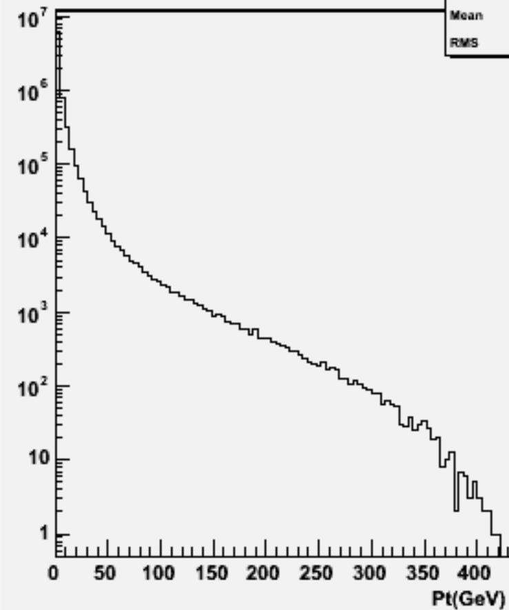
Particle Pt : p106027 physsim-ttz-6q_znn
