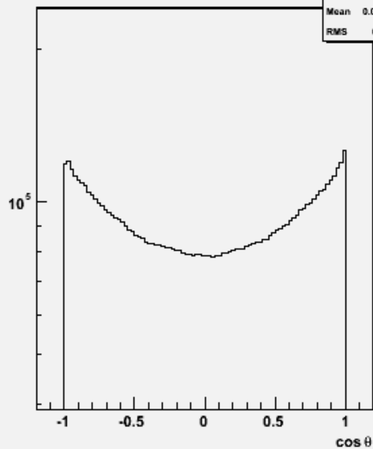
Particle cos \theta : p106027 physsim-ttz-6q_znn
