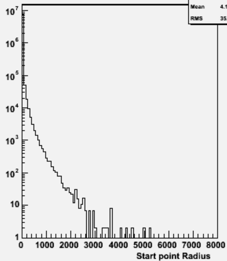
Start point R : p106027 physsim-ttz-6q_znn
