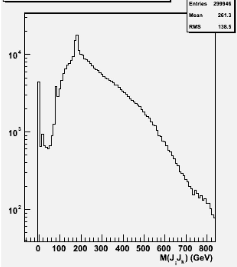
2jets mass(All comb)p106027 physsim-ttz-6q_znn
