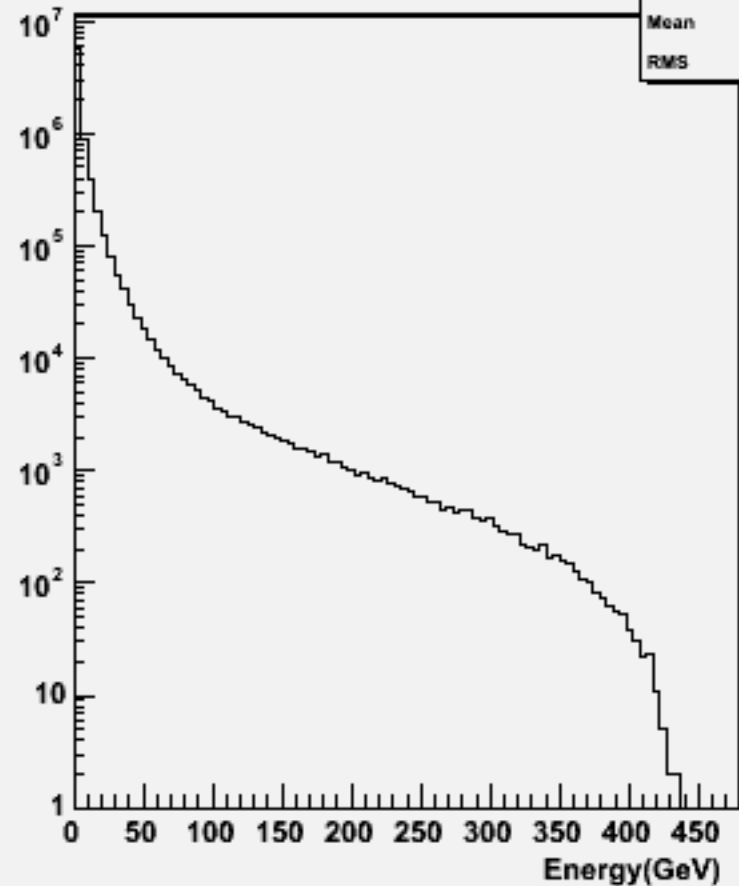
Particle Energy : p106027 physsim-ttz-6q_znn
