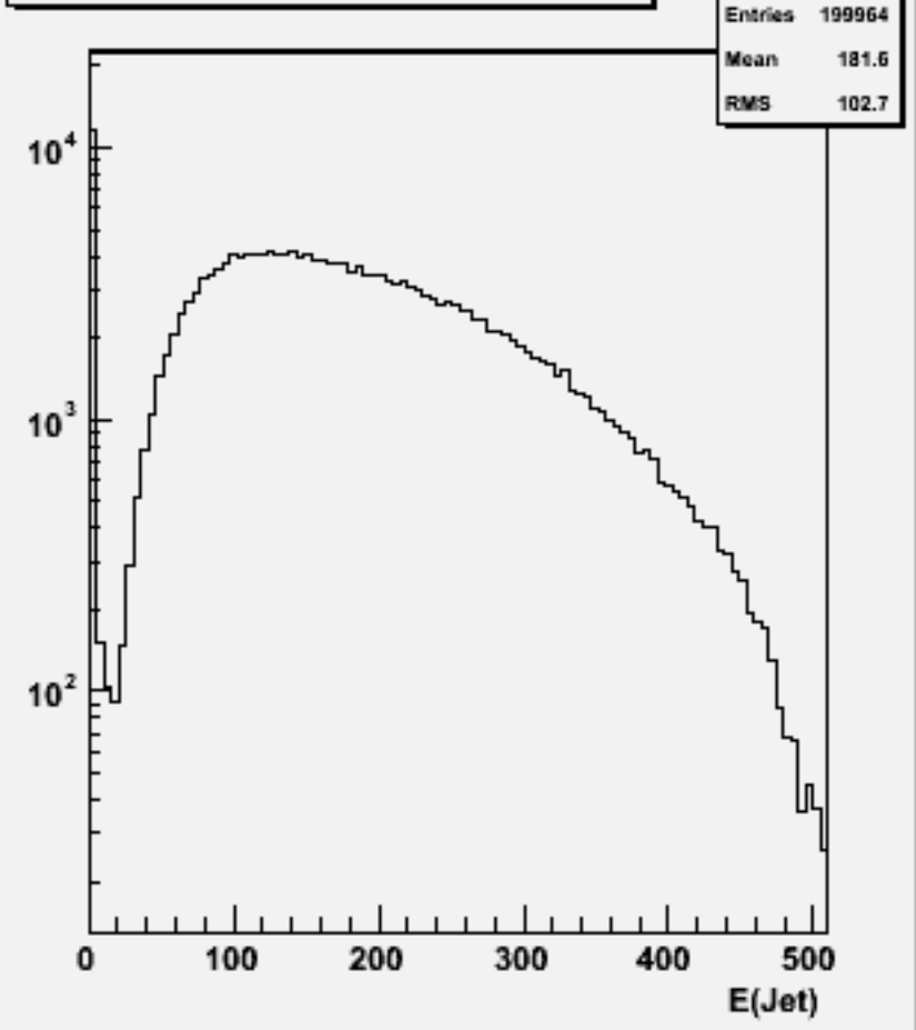
Jet energies(All jets)p106027 physsim-ttz-6q_znn
