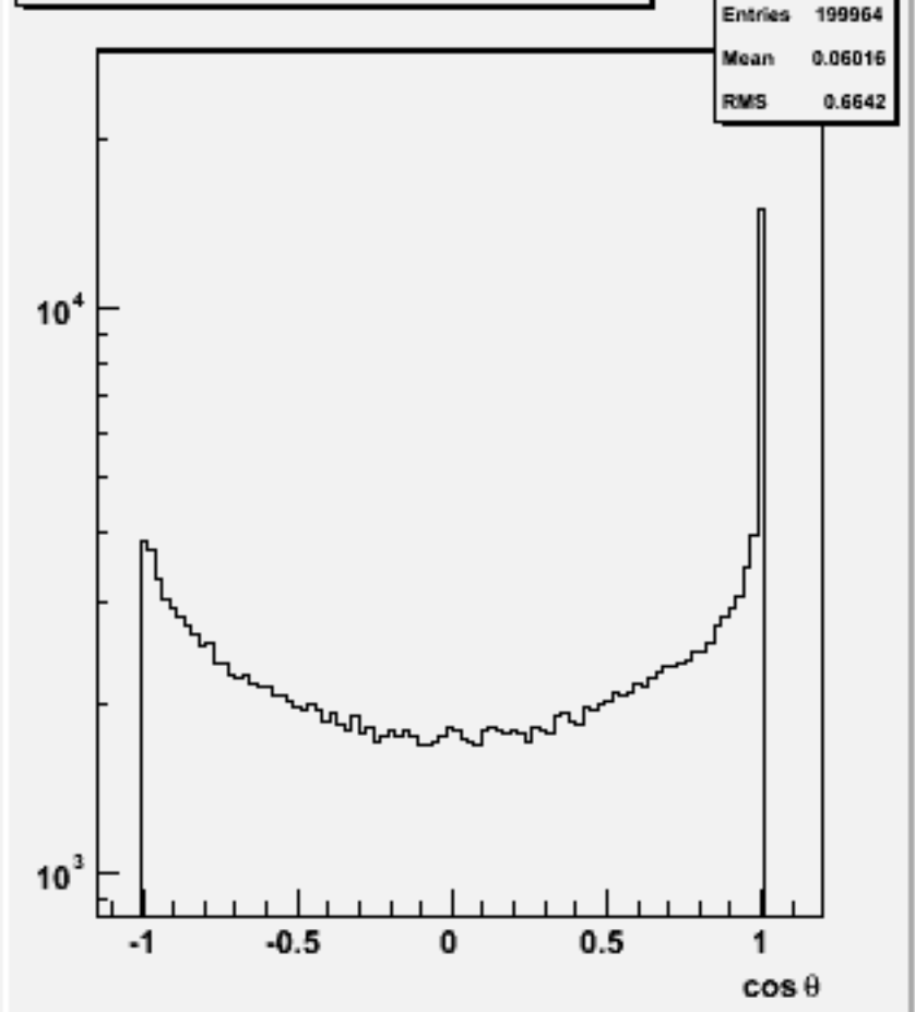
Jet cos \theta (All jets)p106027 physsim-ttz-6q_znn
