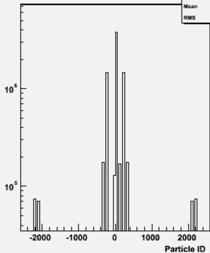
Particle ID : p106027 physsim-ttz-6q_znn
