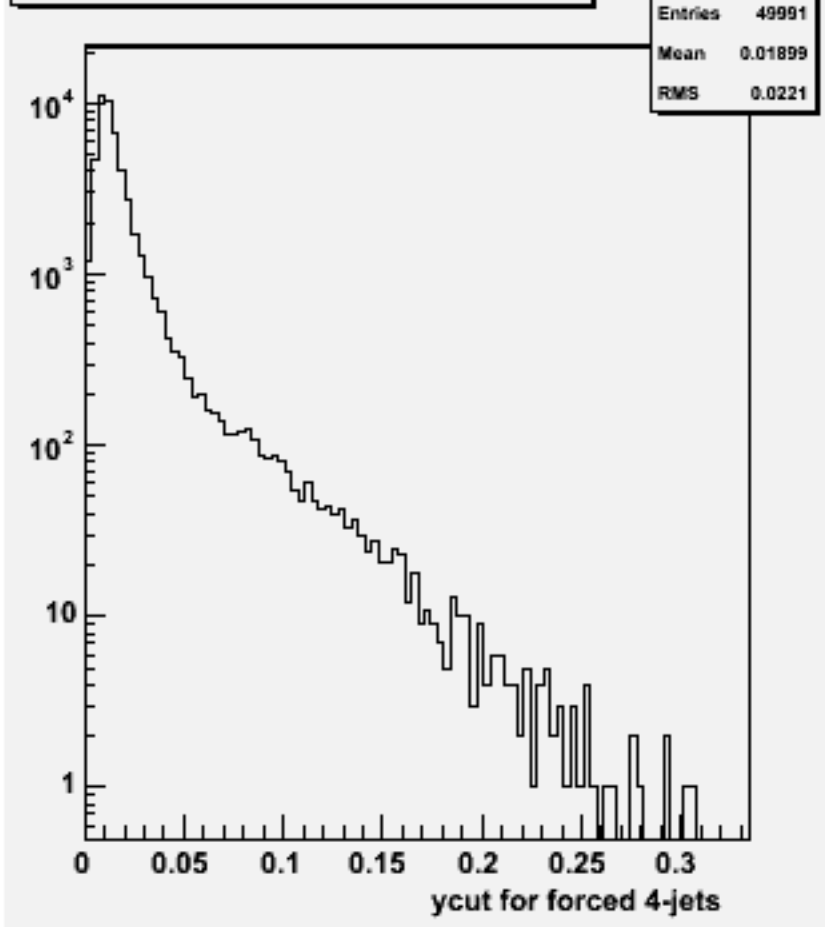
Ycut for 4-jets :p106027 physsim-ttz-6q_znn
