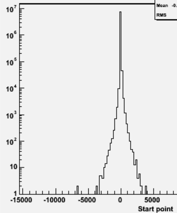
Start point Z : p106027 physsim-ttz-6q_znn
