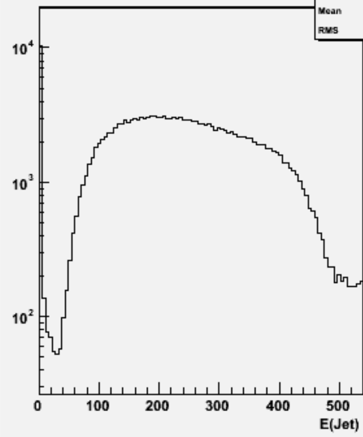
Jet energies(All jets)p106023 physsim-ttz-6q_zqq
