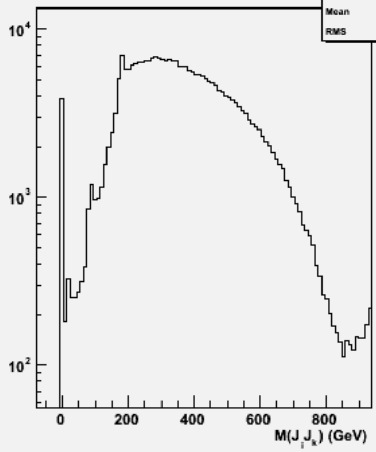
2jets mass(All comb)p106023 physsim-ttz-6q_zqq
