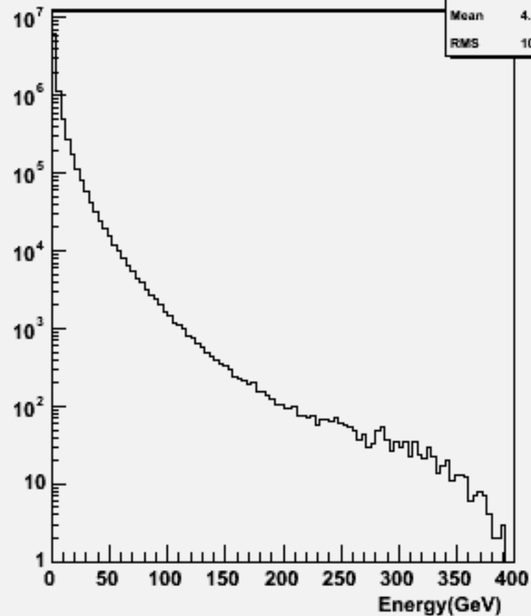
Particle Energy : p106023 physsim-ttz-6q_zqq
