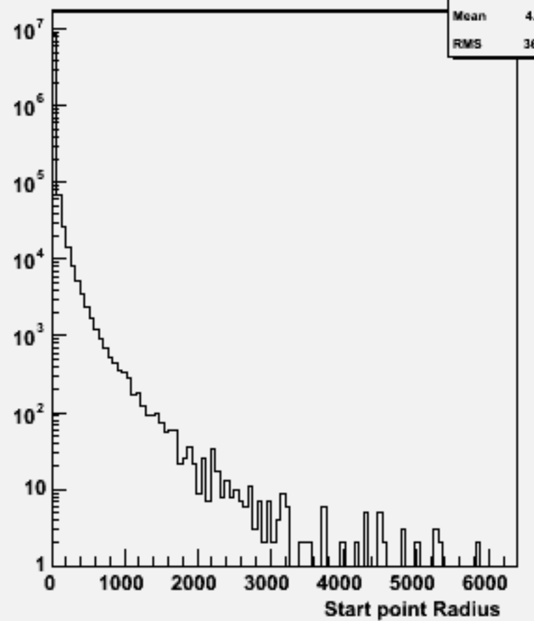
Start point R : p106023 physsim-ttz-6q_zqq
