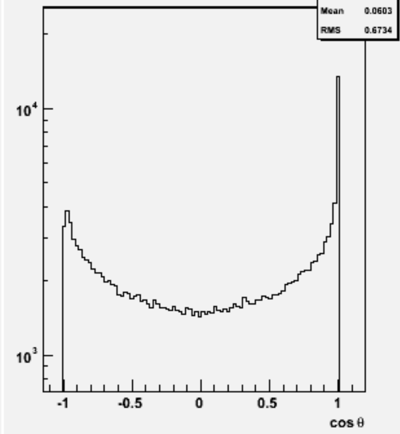
Jet cos \theta (All jets)p106023 physsim-ttz-6q_zqq
