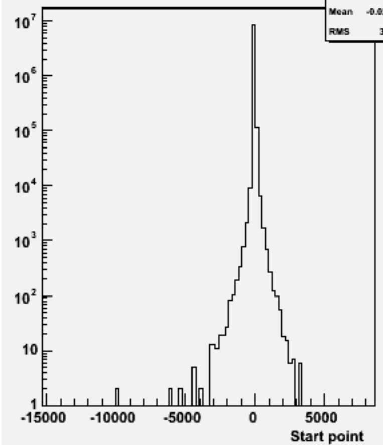
Start point Z : p106023 physsim-ttz-6q_zqq
