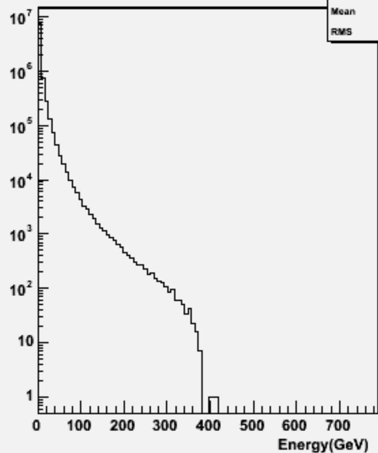
Particle Energy : p106019 physsim-tth-6q_hnonbb
