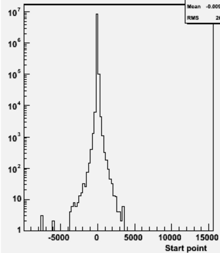
Start point Z : p106019 physsim-tth-6q_hnonbb
