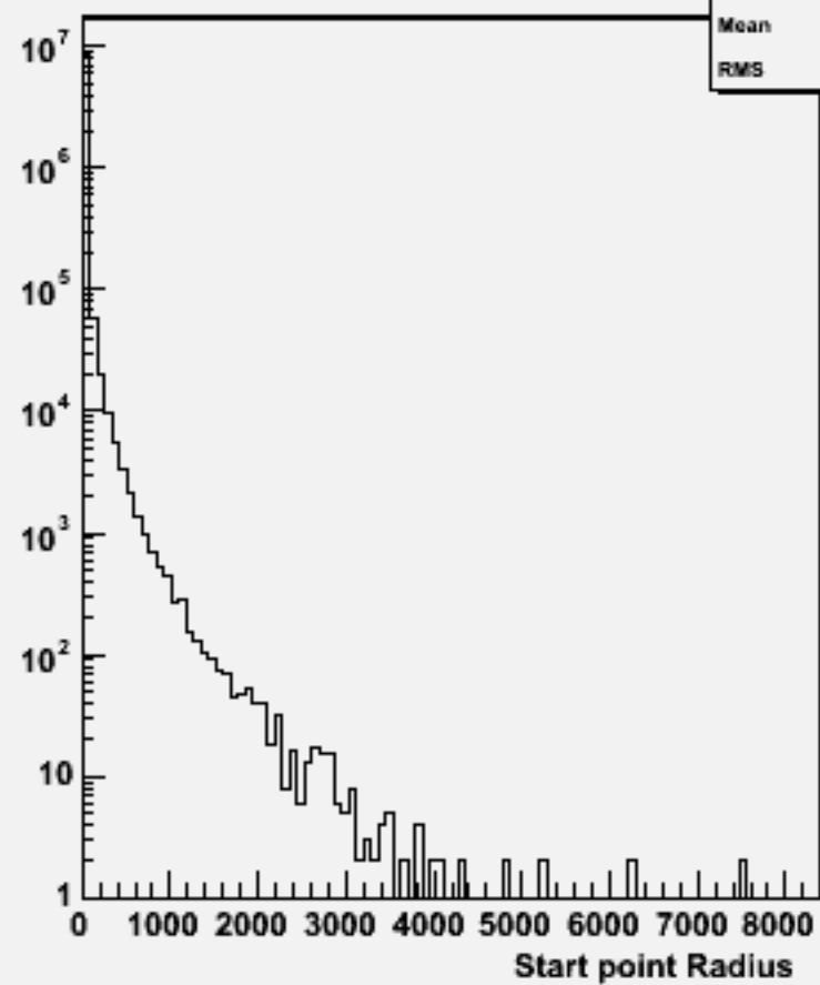
Start point R : p106019 physsim-tth-6q_hnonbb
