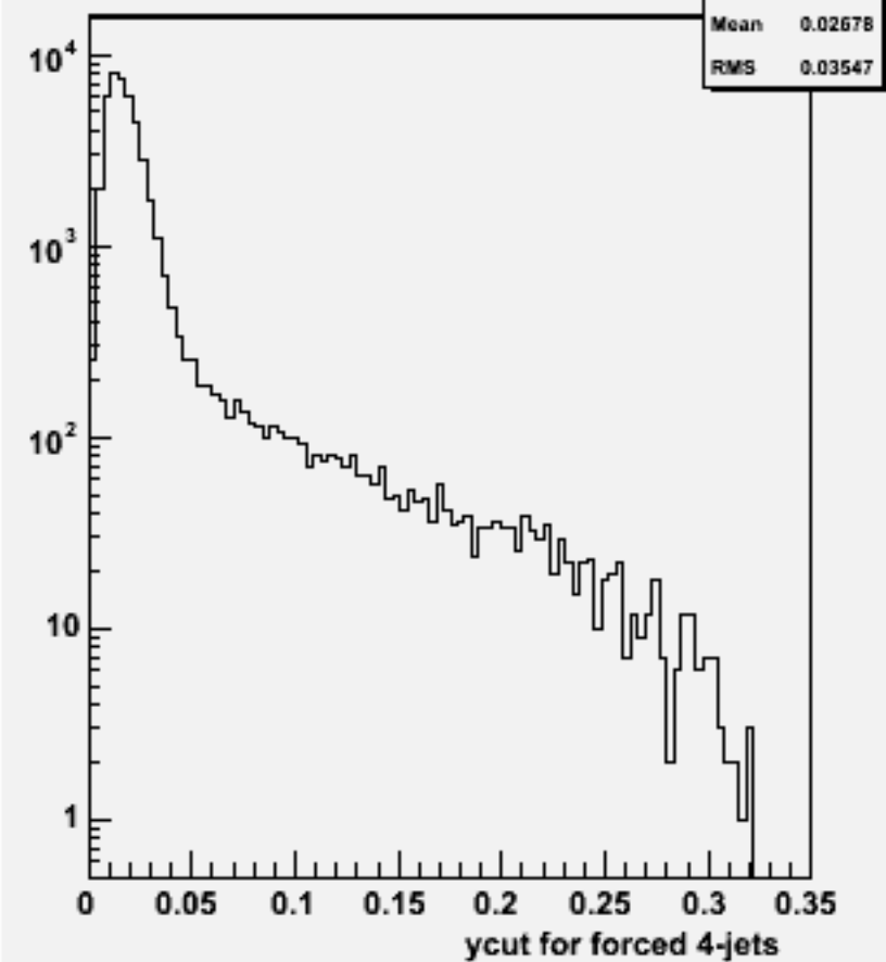
Ycut for 4-jets :p106019 physsim-tth-6q_hnonbb
