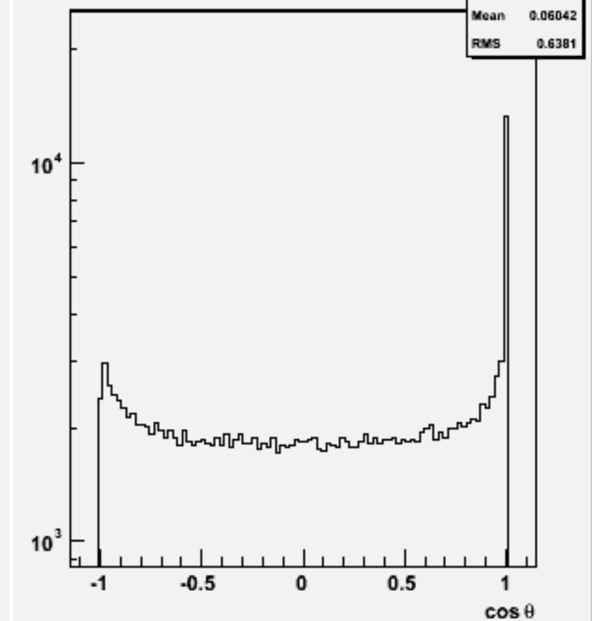
Jet cos \theta (All jets)p106019 physsim-tth-6q_hnonbb
