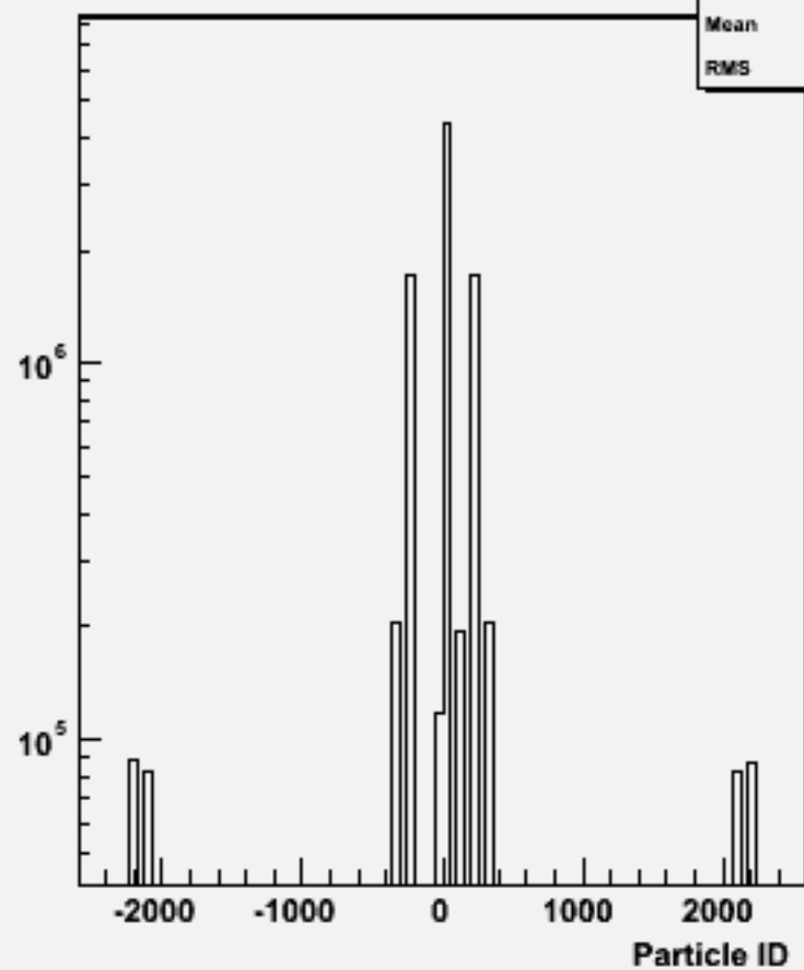
Particle ID : p106019 physsim-tth-6q_hnonbb
