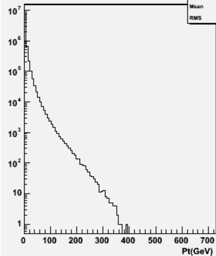
Particle Pt : p106019 physsim-tth-6q_hnonbb
