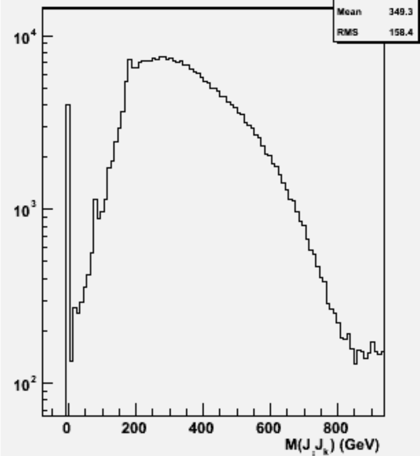
Zjets mass(All comb)p106019 physsim-tth-6q_hnonbb
