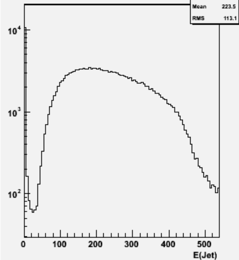
Jet energies(All jets)p106019 physsim-tth-6q_hnonbb
