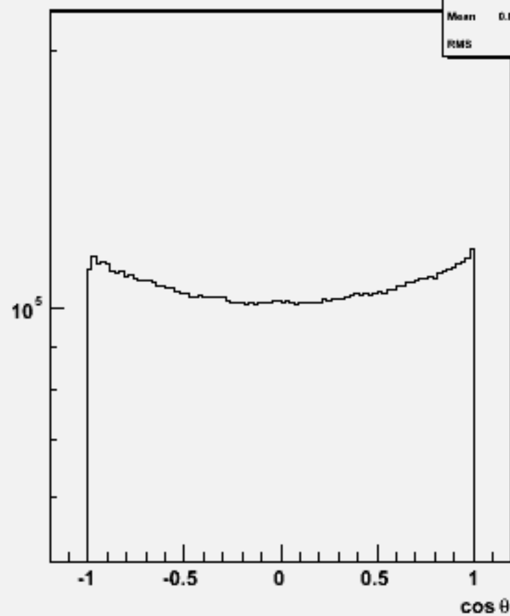
Particle cos \theta : p106019 physsim-tth-6q_hnonbb
