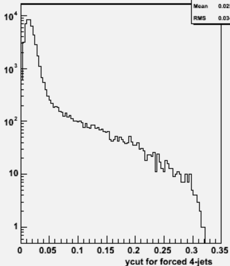
Ycut for 4-jets :p106001 physsim-tth-en4q_all
