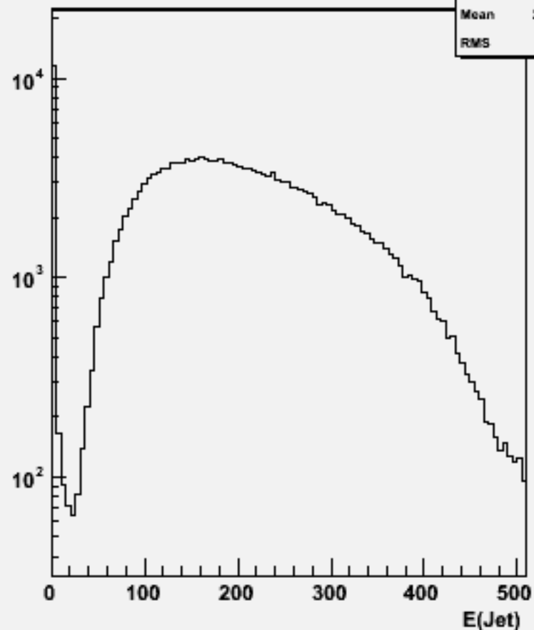
Jet energies(All jets)p106001 physsim-tth-en4q_all
