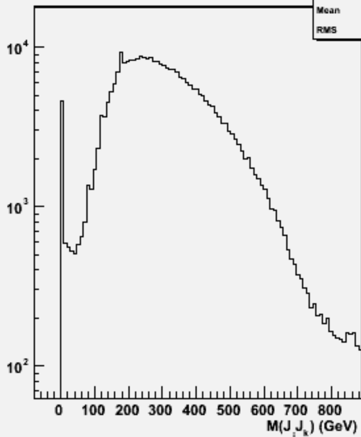
2jets mass(All comb)p106001 physsim-tth-en4q_all
