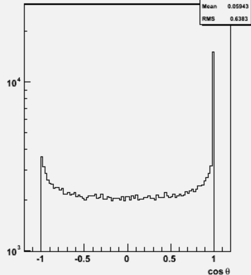
Jet cos \theta (All jets)p106001 physsim-tth-en4q_all
