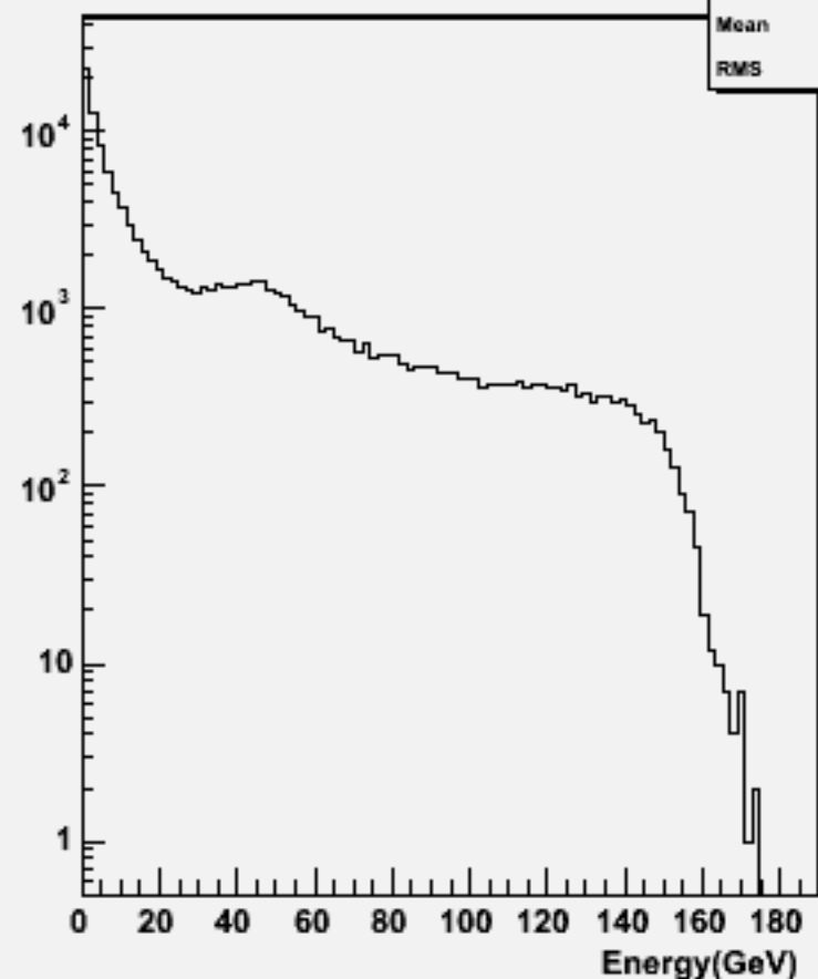
Start point R : w104088 aa_n1n1e3e3_o
