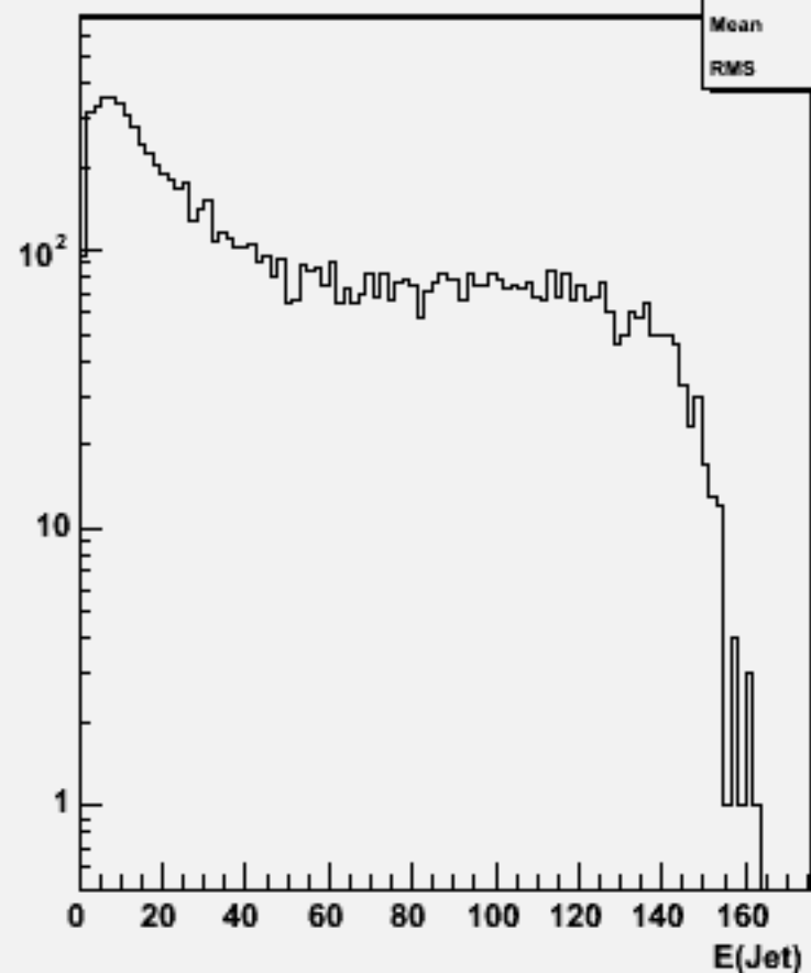
Jet energies(All jets)w104088 aa_n1n1e3e3_o
