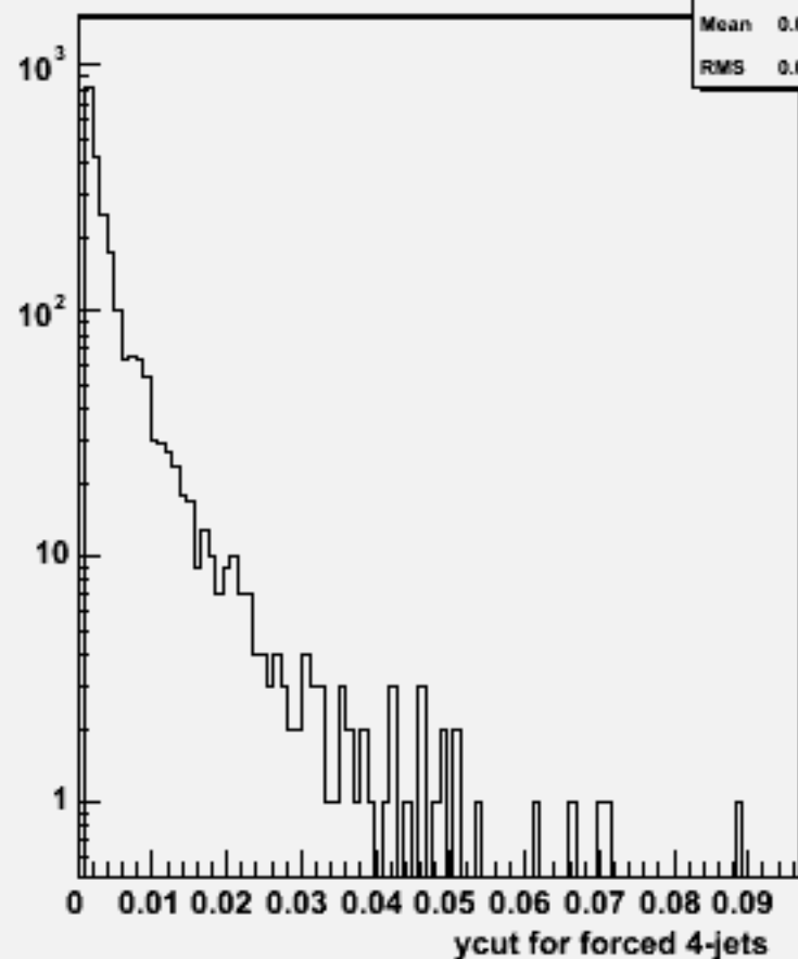
Ycut for 4-jets :w104088 aa_n1n1e3e3_o
