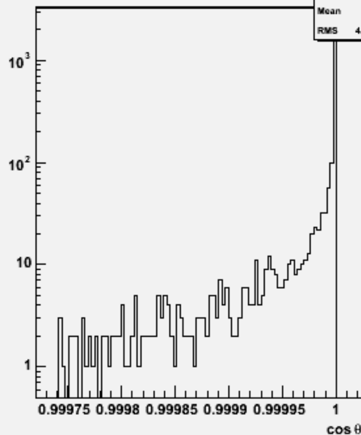
Jet cosθ (All jets)w104088 aa_n1n1e3e3_o
