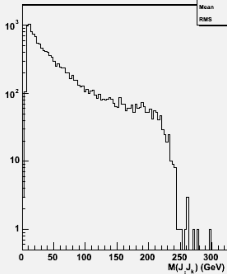
2jets mass(All comb)w104088 aa_n1n1e3e3_o
