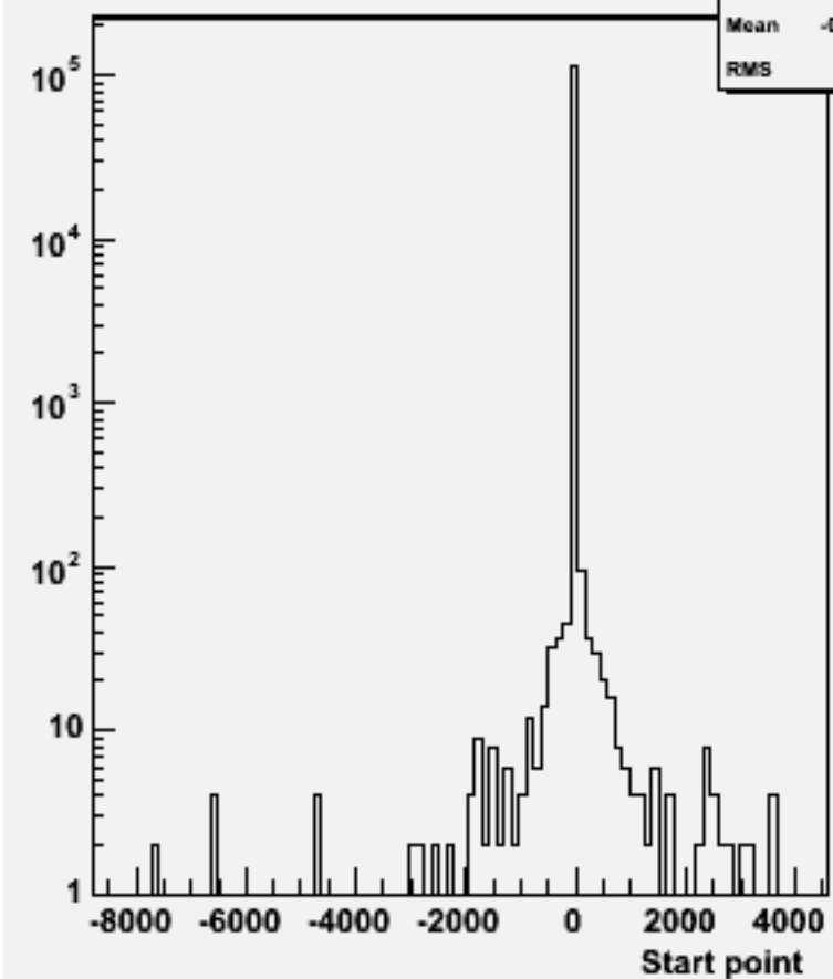
Start point Z : w104088 aa_n1n1e3e3_o
