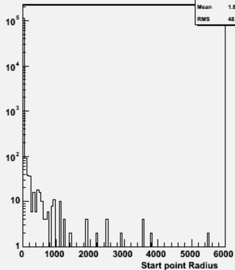
Start point R : w104088 aa_n1n1e3e3_o
