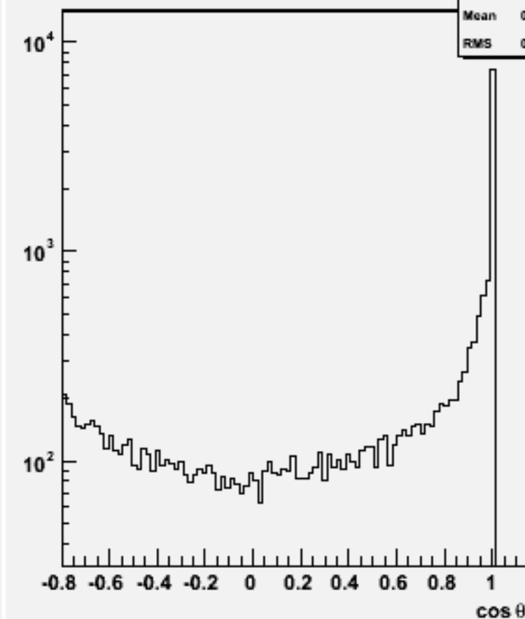
Jet cos \theta (All jets)w104056 aa_n2n2uu_o
