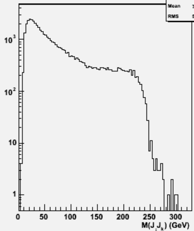
2jets mass(All comb)w104056 aa_n2n2uu_o
