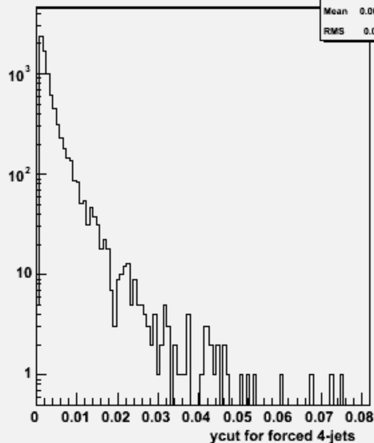
Ycut for 4-jets :w104056 aa_n2n2uu_o
