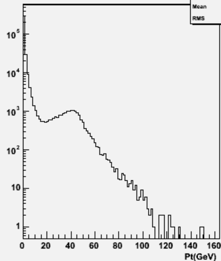
Particle Pt : w104052 aa_n1n1cc_o
