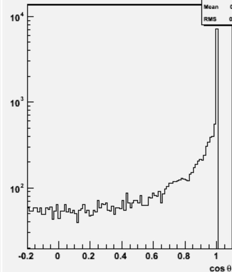
Jet cos \theta (All jets)w104052 aa_n1n1cc_o
