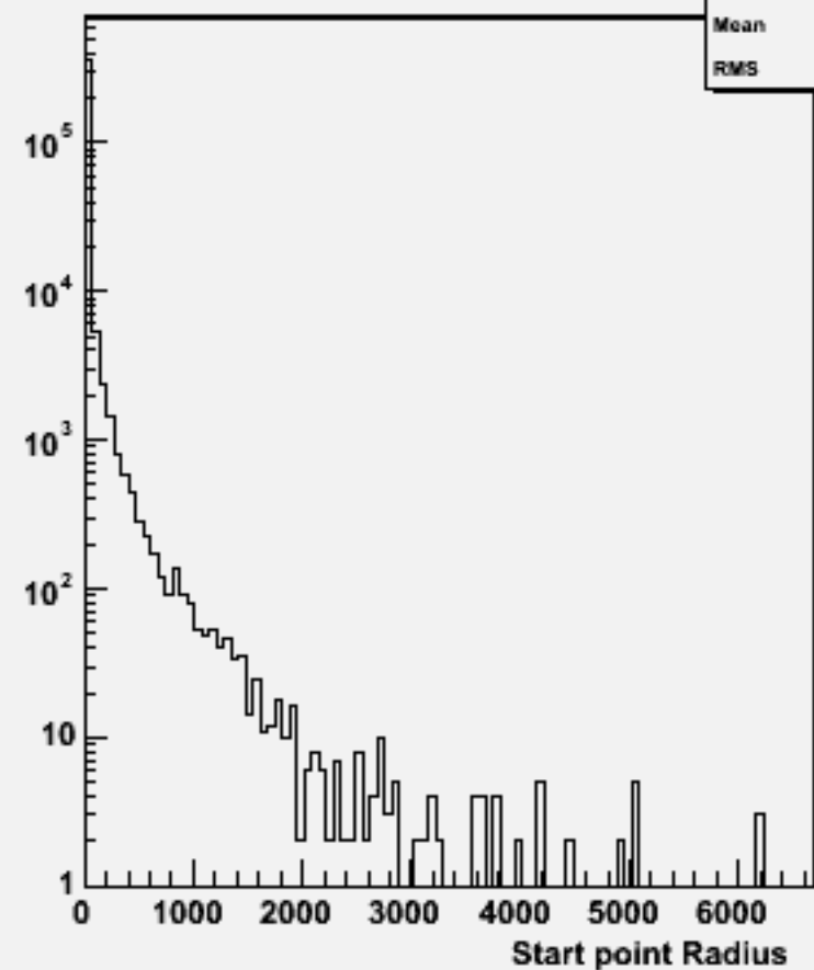
Start point R : w104052 aa_n1n1cc_o
