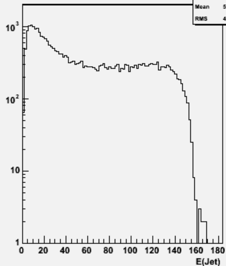
Jet energies(All jets)w104052 aa_n1n1cc_o
