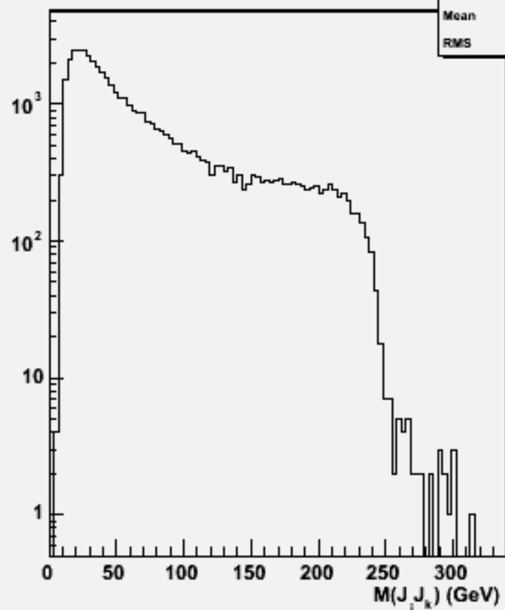
2jets mass(All comb)w104052 aa_n1n1cc_o
