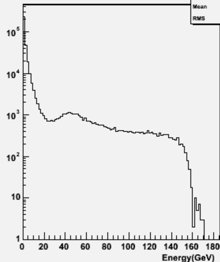
Particle Energy : w104052 aa_n1n1cc_o
