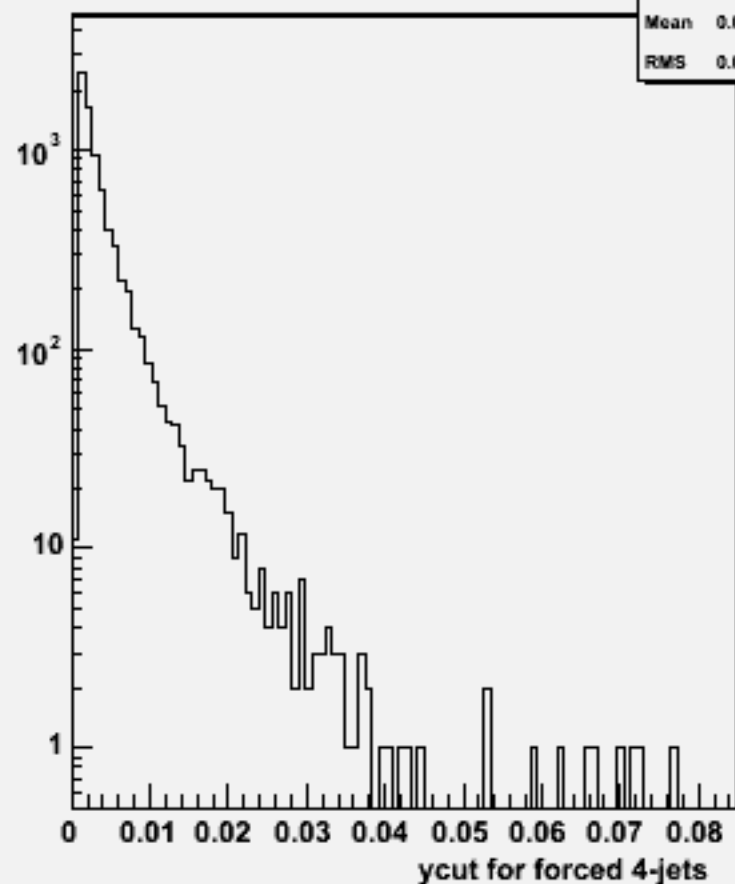
Ycut for 4-jets :w104052 aa_n1n1cc_o
