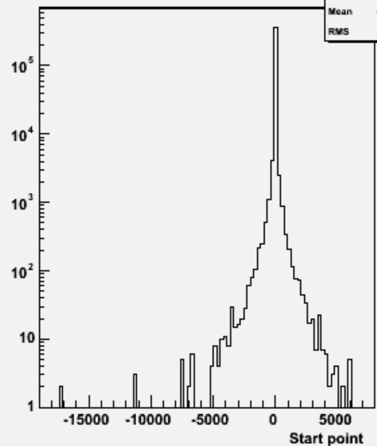
Start point Z : w104052 aa_n1n1cc_o
