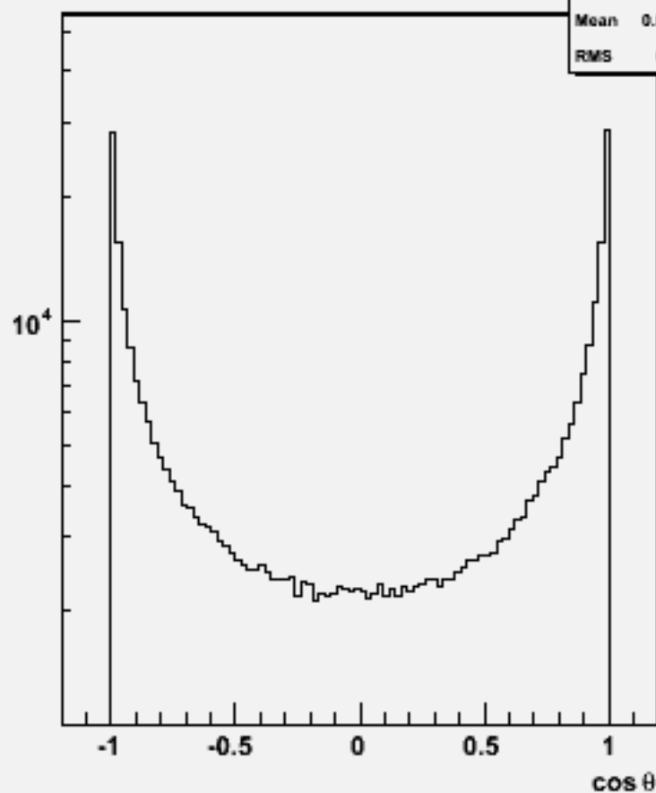
Particle cos \theta : w104052 aa_n1n1cc_o
