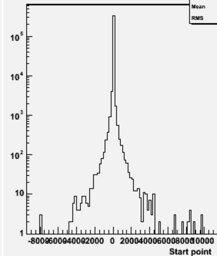
Start point Z : w104048 aa_n1n1uu_o
