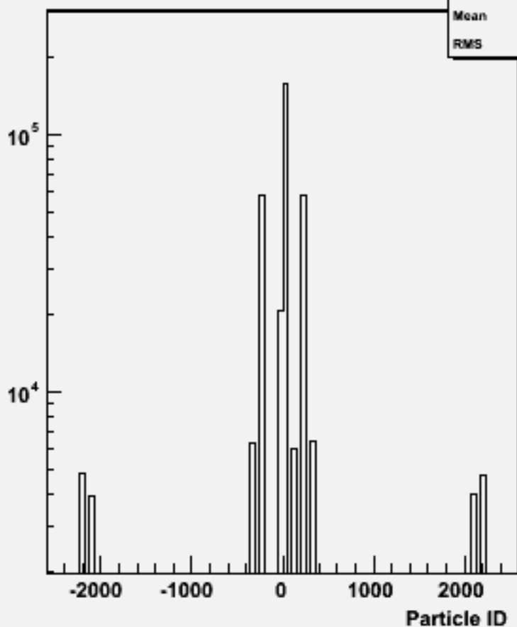
Particle ID : w104048 aa_n1n1uu_o
