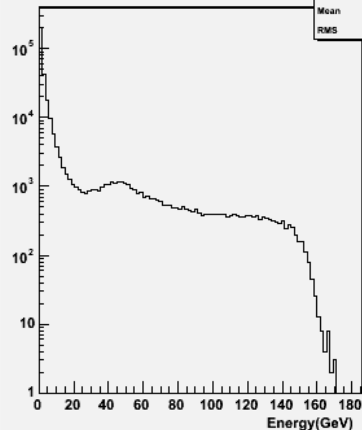
Particle Energy : w104048 aa_n1n1uu_o
