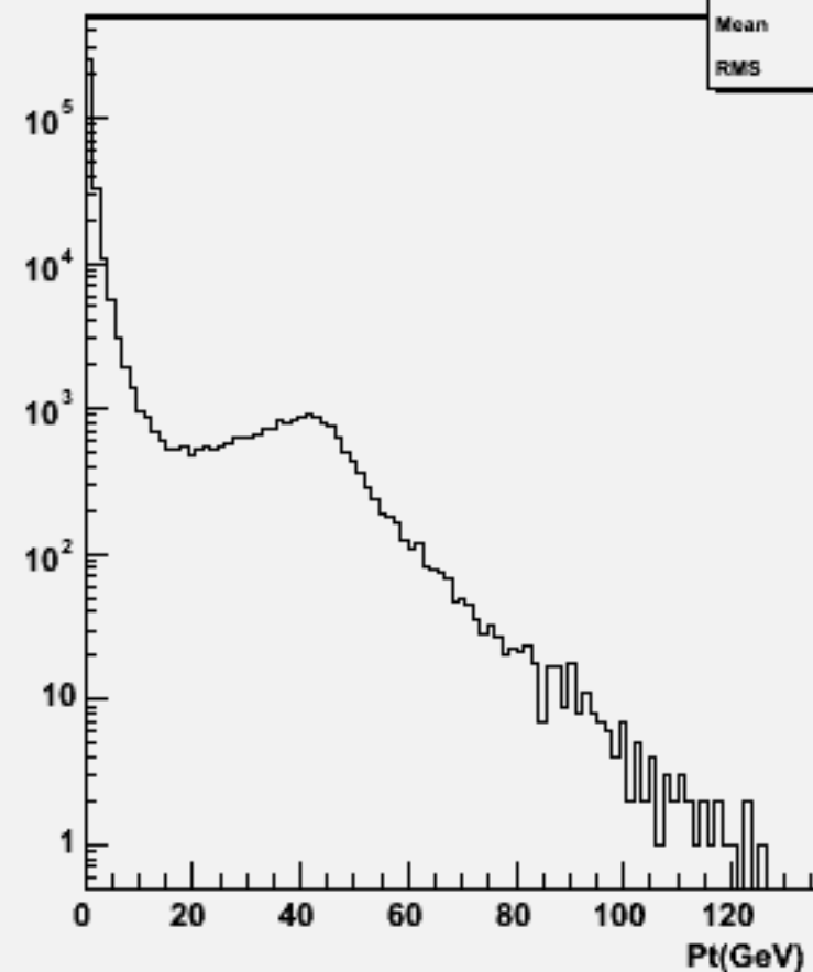
Particle Pt : w104048 aa_n1n1uu_o
