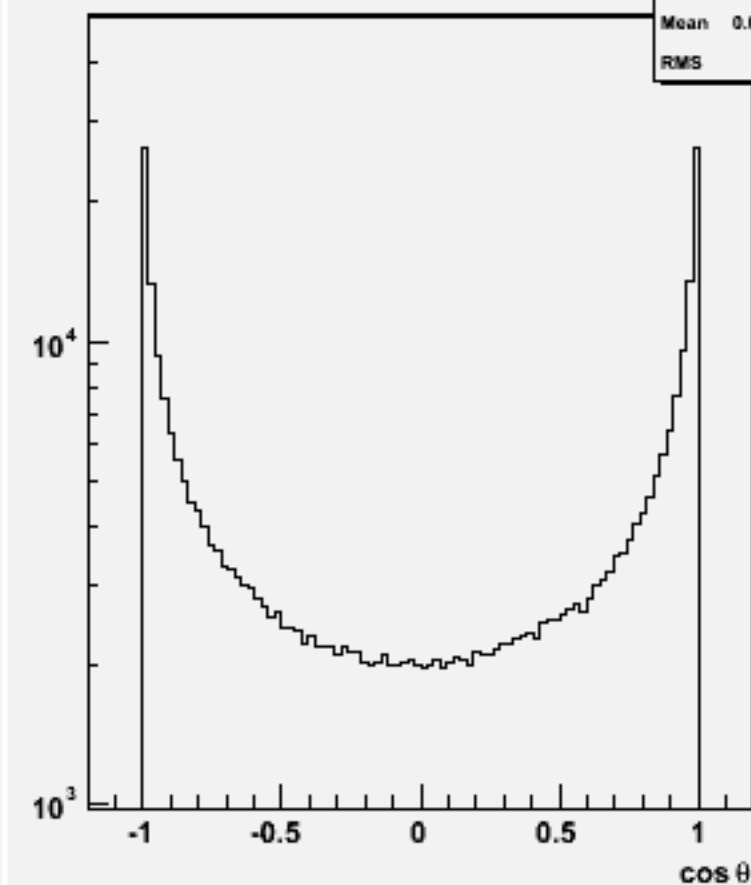
Particle cos \theta : w104048 aa_n1n1uu_o
