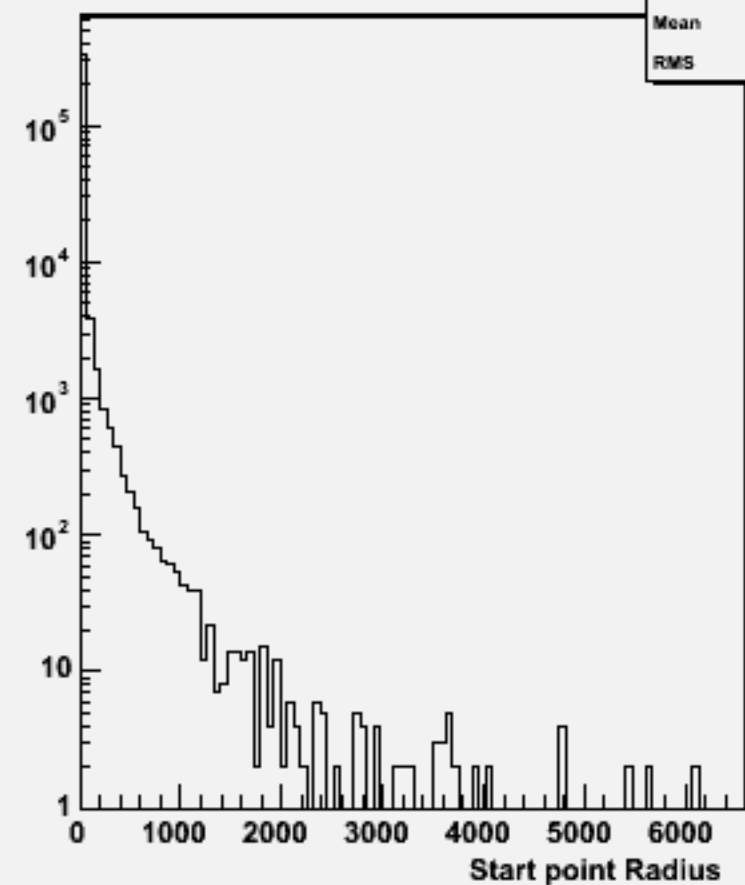
Start point R : w104048 aa_n1n1uu_o
