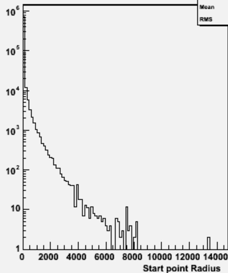
Start point R : w104046 aa_cssc_o
