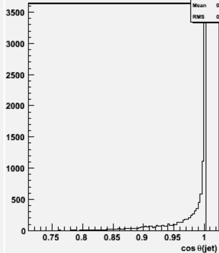
cos \theta for 2-jets :w104046 aa_cssc_o
