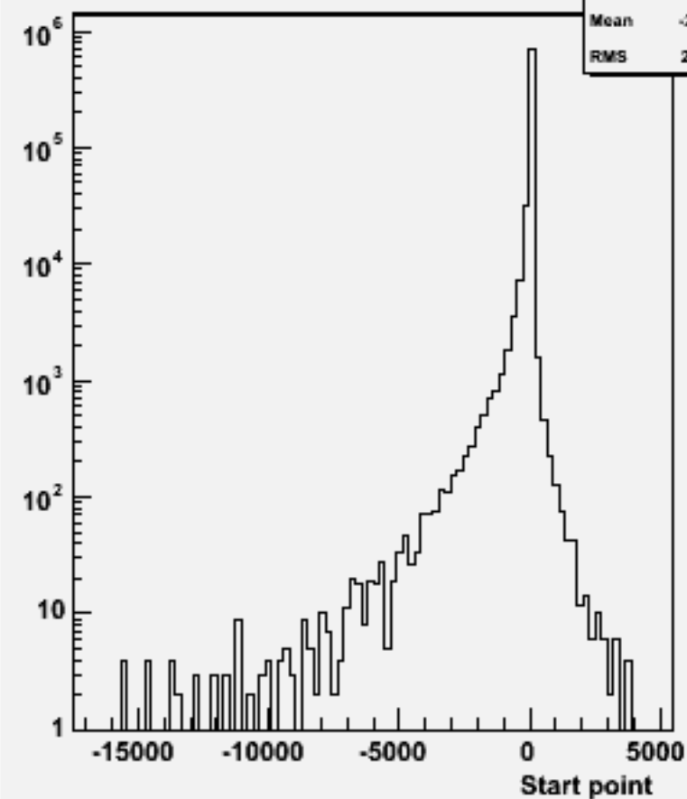
Start point Z : w104046 aa_cssc_o
