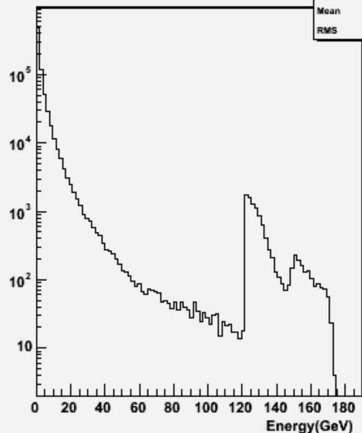
Particle Energy : w104046 aa_cssc_o
