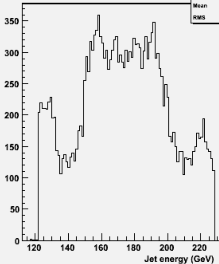
energy for 2-jets :w104046 aa_cssc_o
