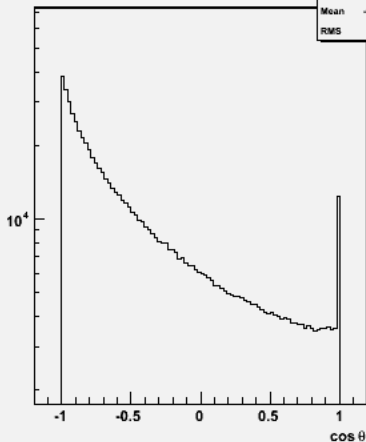
Particle cosθ : w104046 aa_cssc_o
