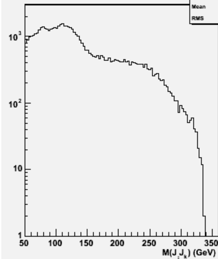
2jets mass(All comb)w104045 aa_cssc_o
