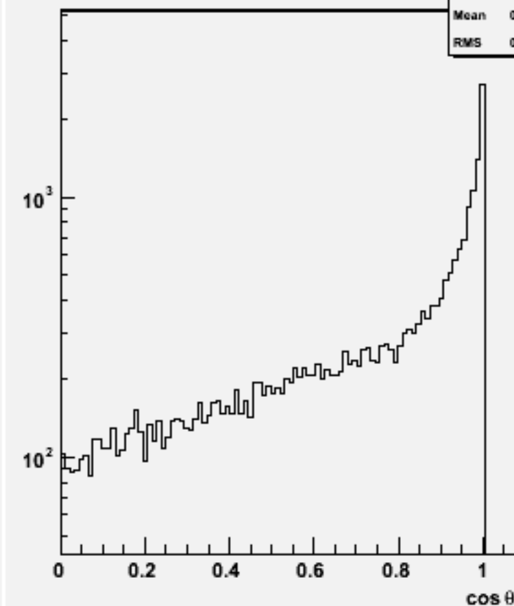
Jet cos \theta (All jets)w104045 aa_cssc_o
