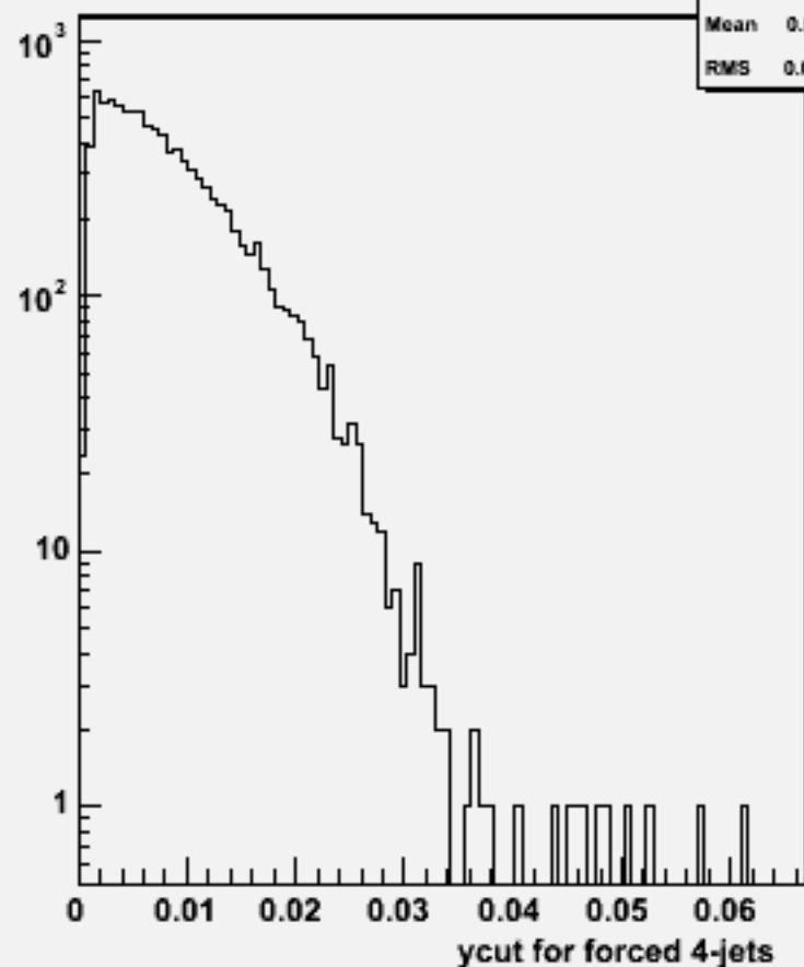
Ycut for 4-jets :w104045 aa_cssc_o
