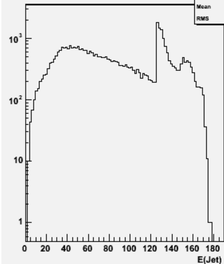
Jet energies(All jets)w104045 aa_cssc_o
