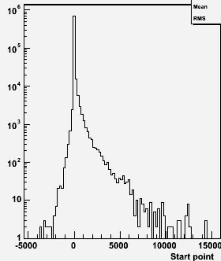
Start point Z : w104045 aa_cssc_o
