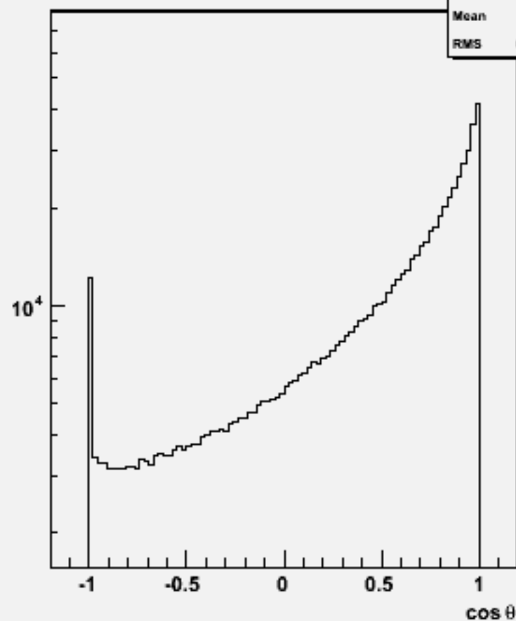
Particle cosθ : w104045 aa_cssc_o
