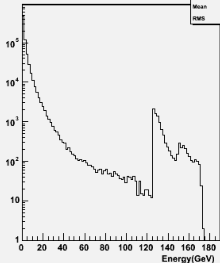
Particle Energy : w104045 aa_cssc_o
