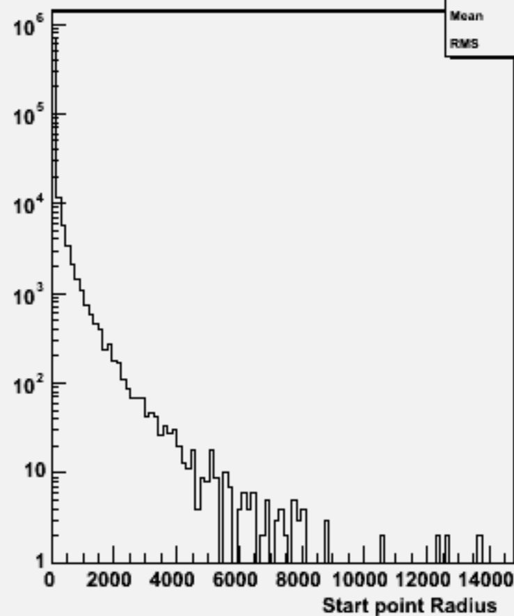
Start point R : w104045 aa_cssc_o
