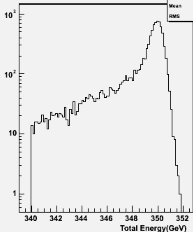
Total Energy (inc. \nu ): w104040 aa_csdu_o
