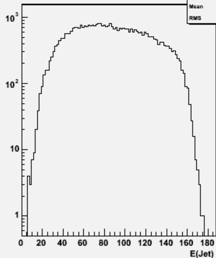
Jet energies(All jets)w104040 aa_csdu_o
