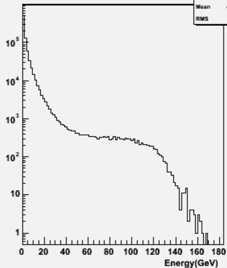
Particle Energy : w104040 aa_csdu_o
