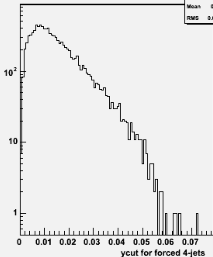
Ycut for 4-jets :w104040 aa_csdu_o
