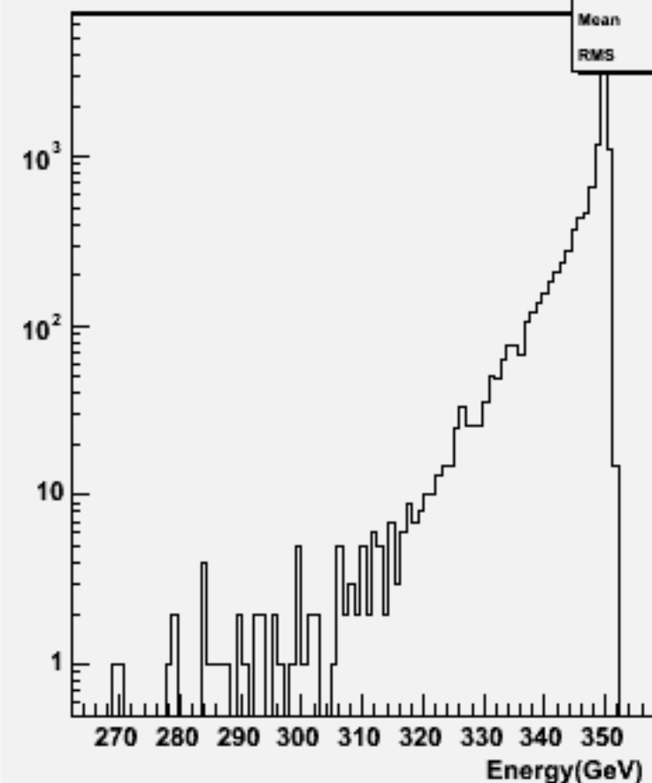
Total Energy (w/o \nu ): w104040 aa_csdu_o
