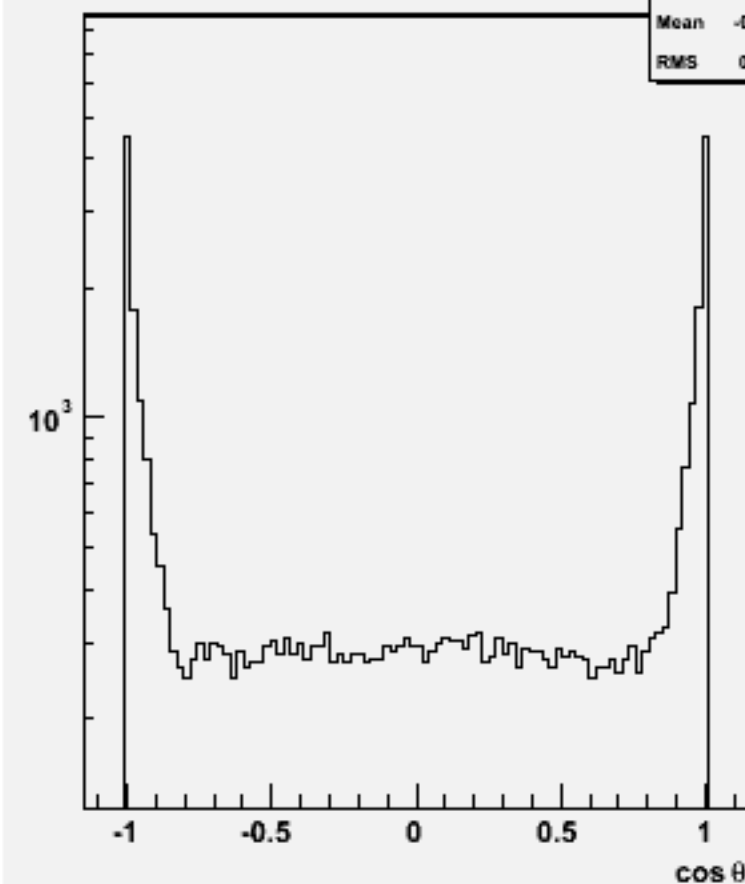
Jet cos \theta (All jets)w104040 aa_csdu_o
