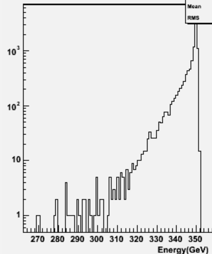
Total Energy (w/o \nu ): w104040 aa_csdu_o
