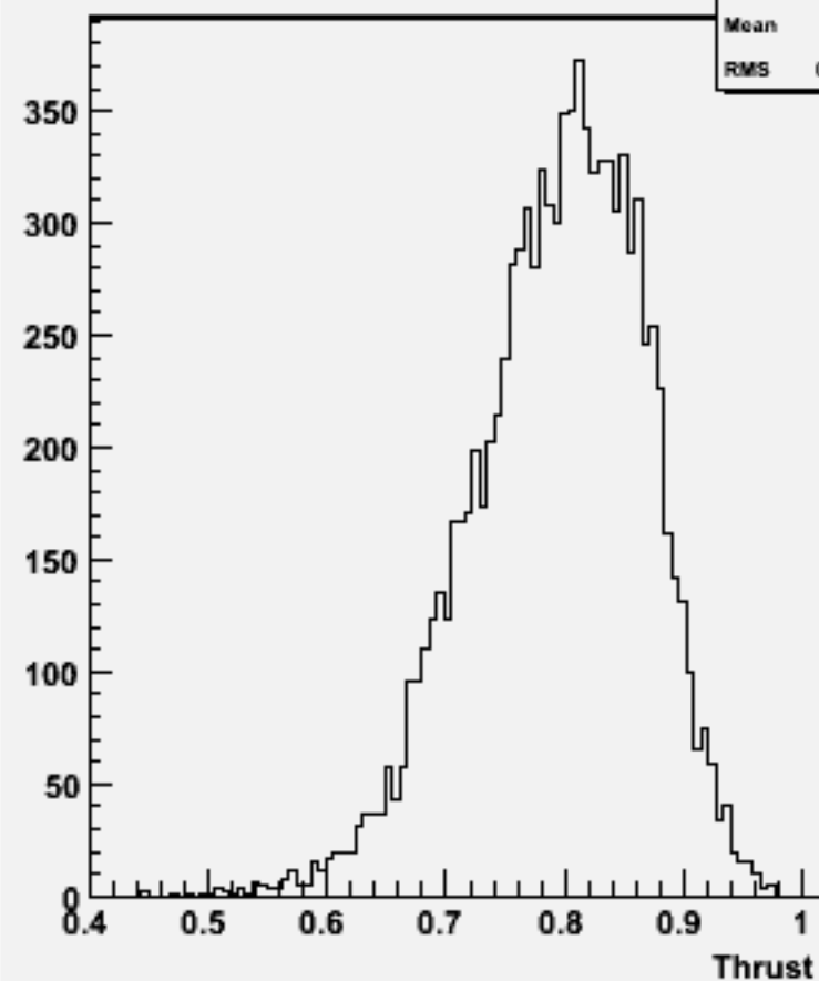
Thrust w104040 aa_csdu_o
