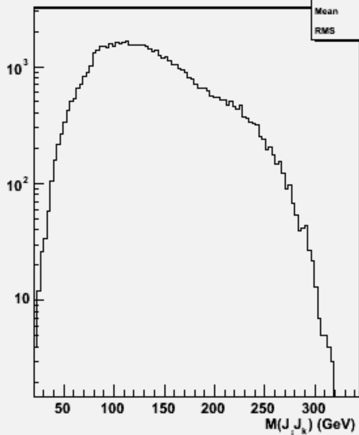
2jets mass(All comb)w104040 aa_csdu_o
