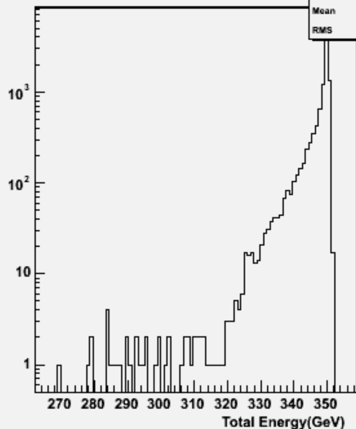
Total Energy (inc. \nu ): w104040 aa_csdu_o
