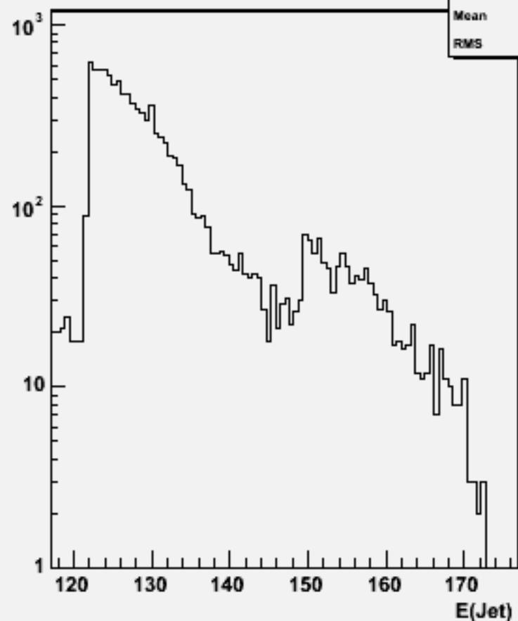
Jet energies(All jets)w104038 aa_cse3n3_o
