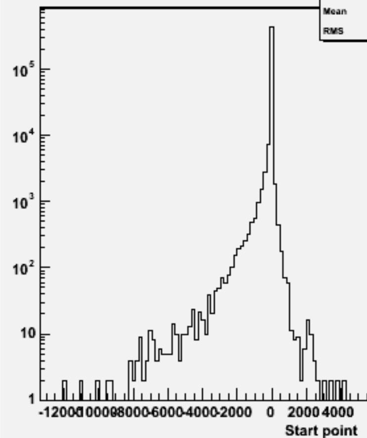
Start point Z : w104038 aa_cse3n3_o
