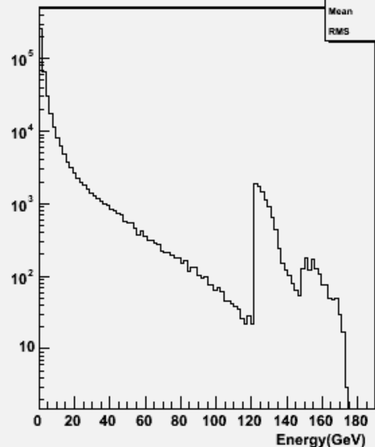
Particle Energy : w104038 aa_cse3n3_o
