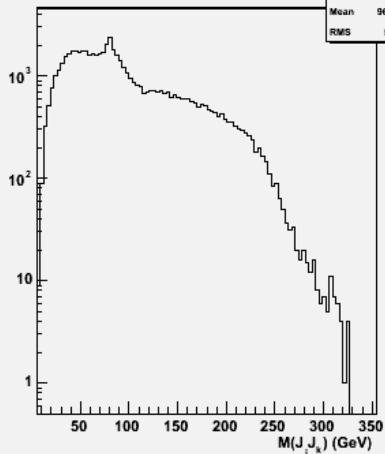
2jets mass(All comb)w104038 aa_cse3n3_o
