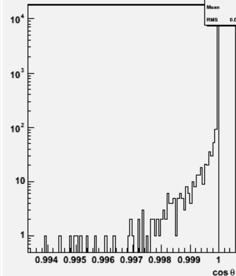
Jet cos \theta (All jets)w104038 aa_cse3n3_o
