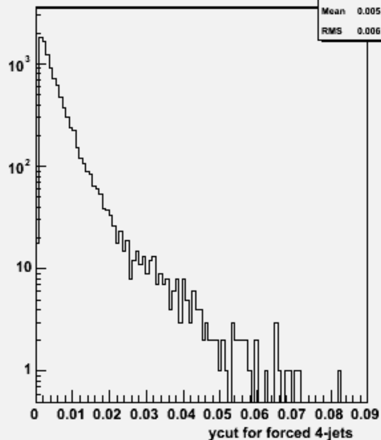
Ycut for 4-jets :w104038 aa_cse3n3_o
