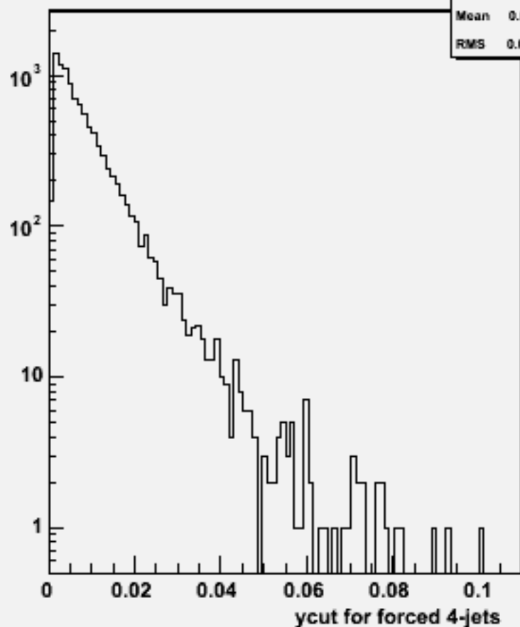
Ycut for 4-jets :w104036 aa_cse3n3_o
