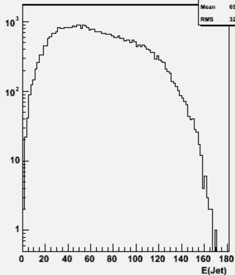
Jet energies(All jets)w104036 aa_cse3n3_o
