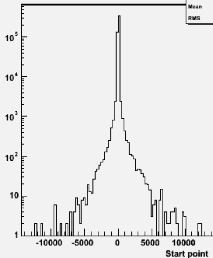
Start point Z : w104036 aa_cse3n3_o
