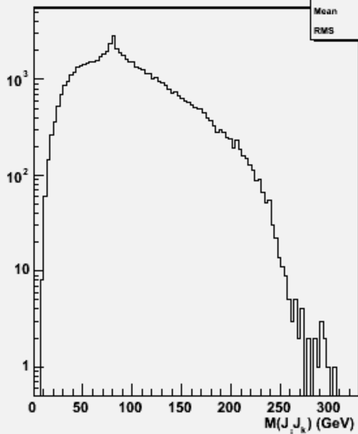
2jets mass(All comb)w104036 aa_cse3n3_o
