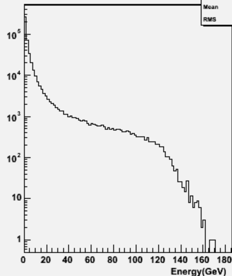
Particle Energy : w104036 aa_cse3n3_o
