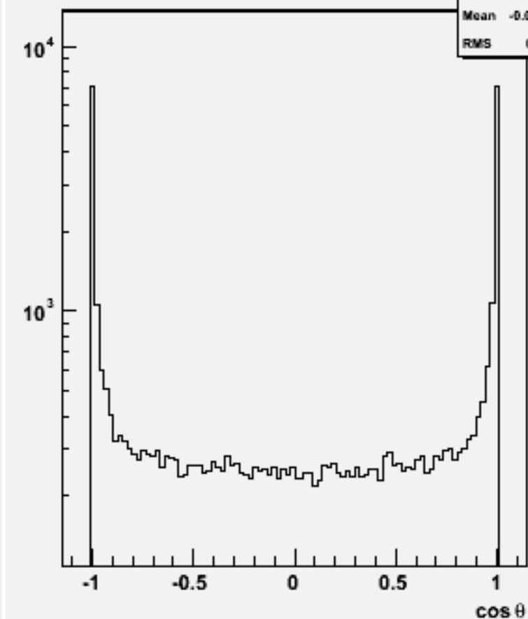
Jet cos \theta (All jets)w104036 aa_cse3n3_o
