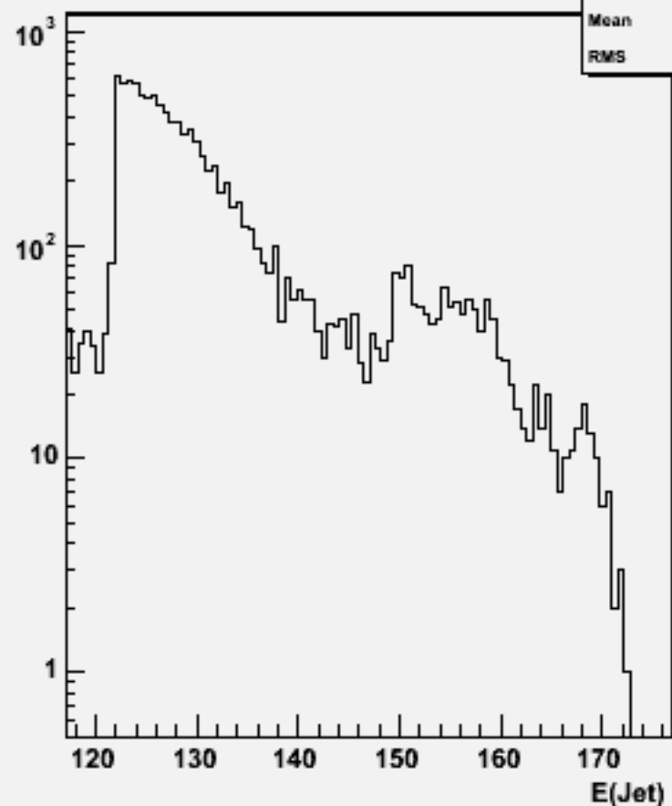
Jet energies(All jets)w104034 aa_cse2n2_o
