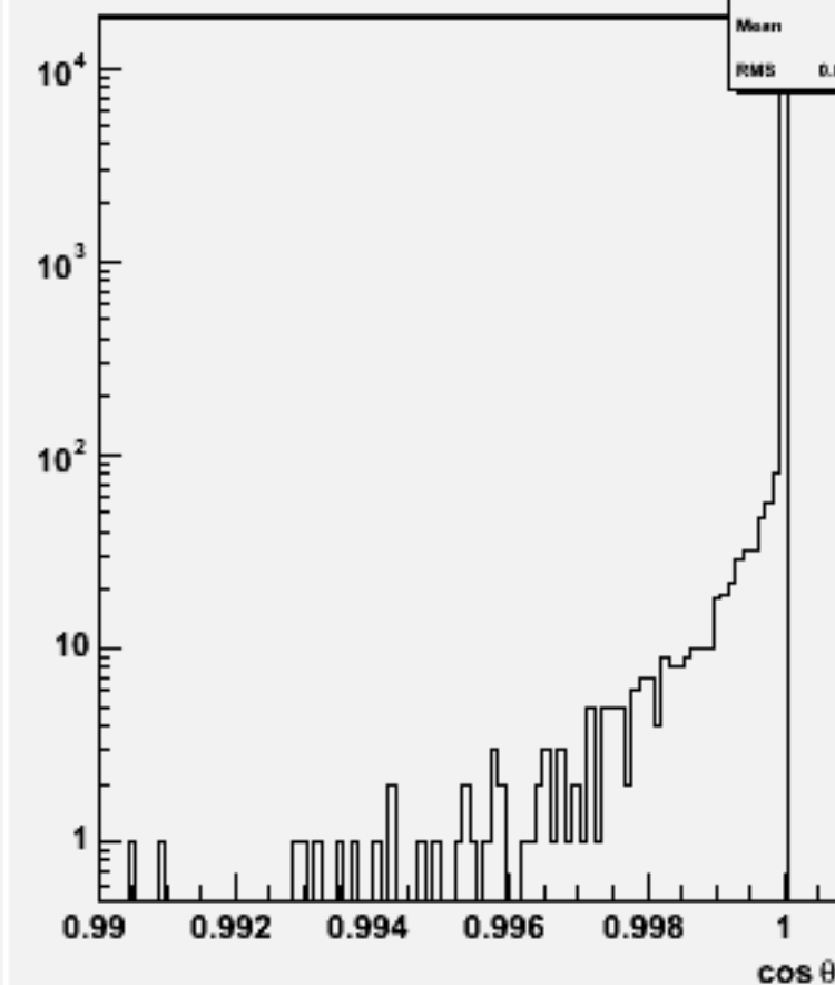
Jet cos \theta (All jets)w104034 aa_cse2n2_o
