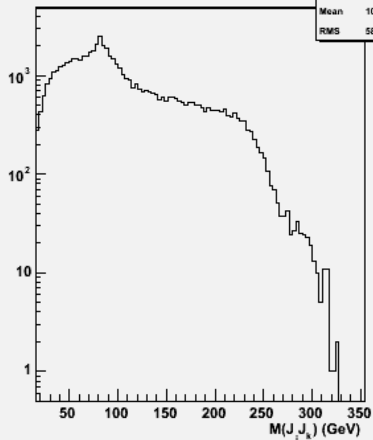
2jets mass(All comb)w104034 aa_cse2n2_o
