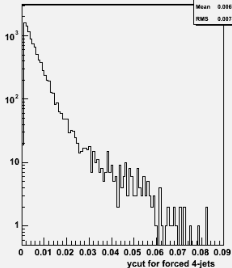
Ycut for 4-jets :w104034 aa_cse2n2_o
