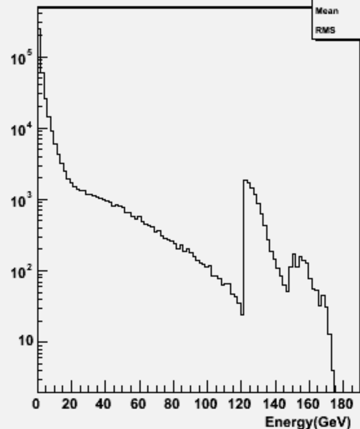
Particle Energy : w104034 aa_cse2n2_o
