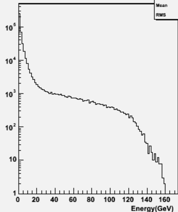
Particle Energy : w104032 aa_cse2n2_o
