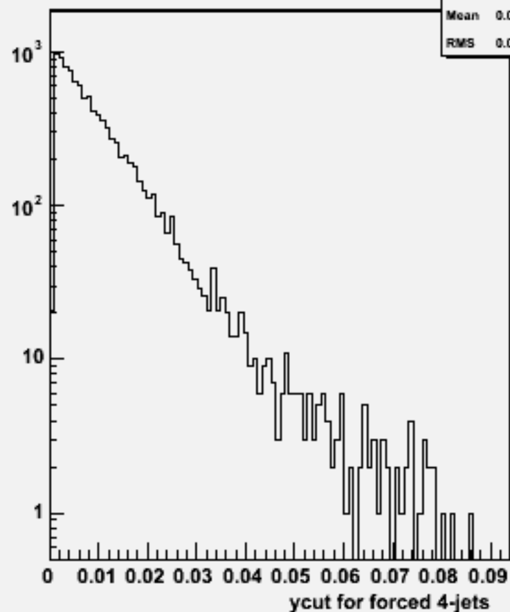
Ycut for 4-jets :w104032 aa_cse2n2_o
