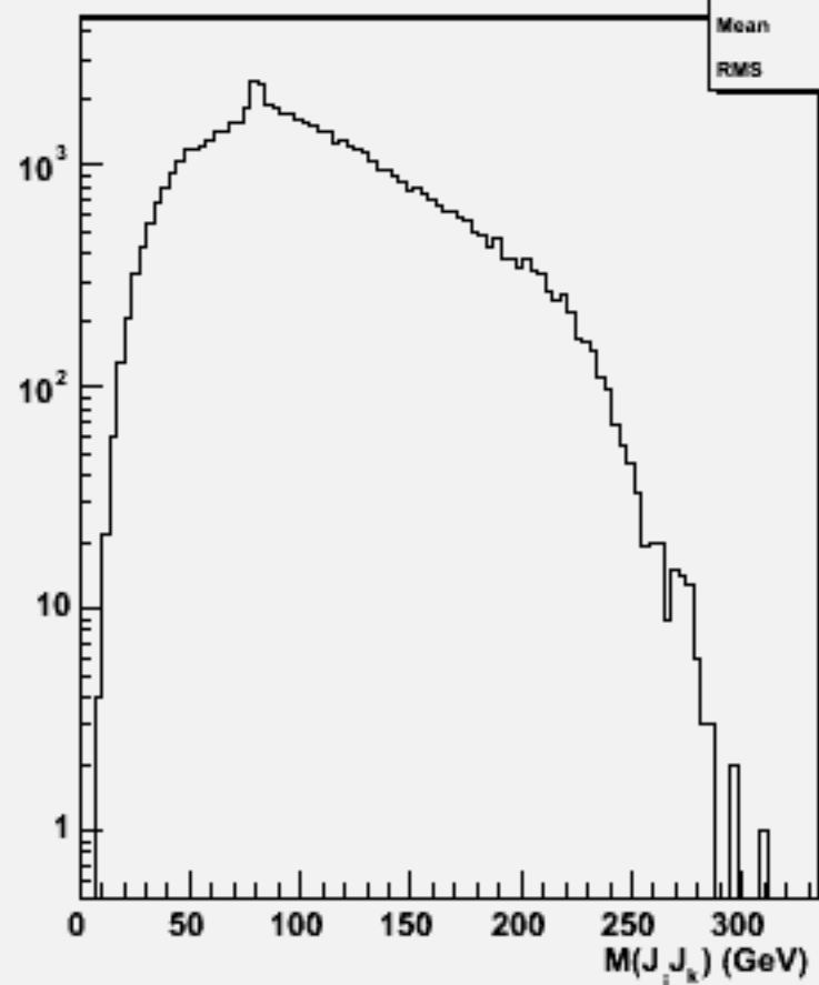
2jets mass(All comb)w104032 aa_cse2n2_o
