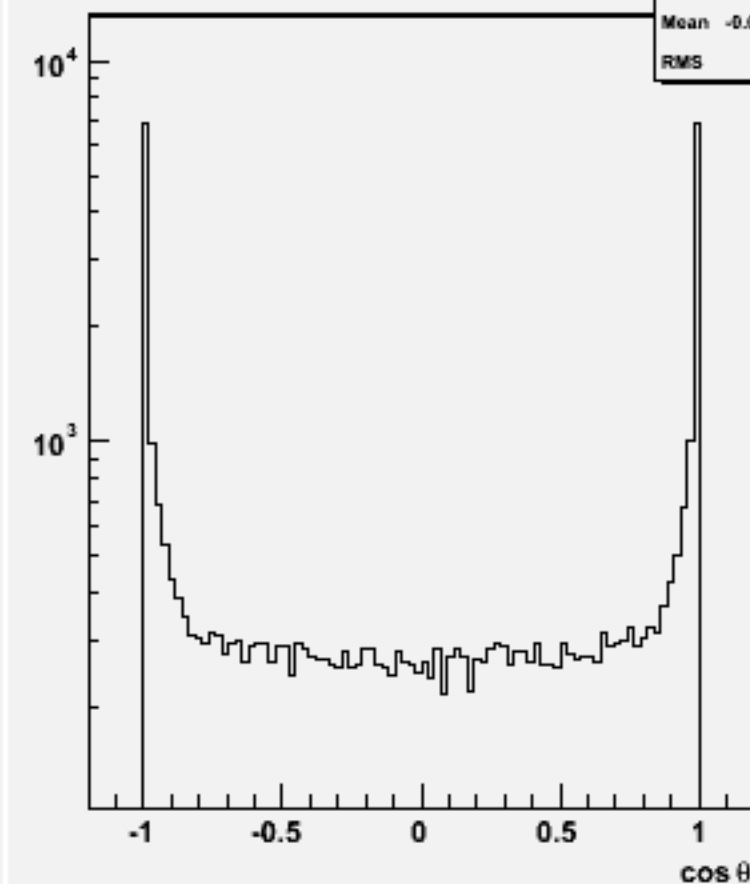
Jet cos \theta (All jets)w104032 aa_cse2n2_o
