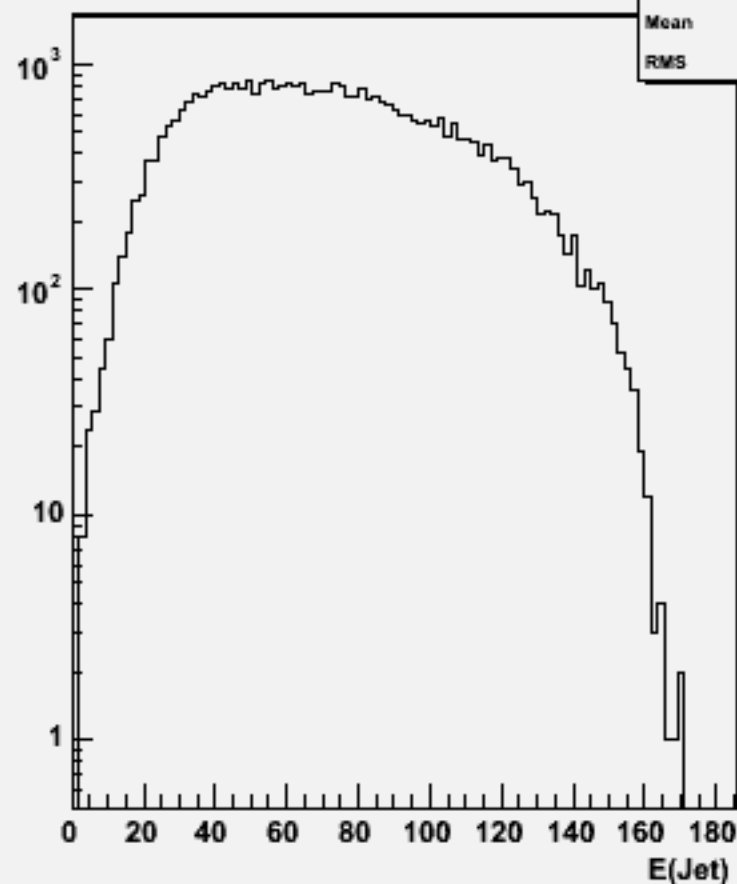
Jet energies(All jets)w104032 aa_cse2n2_o
