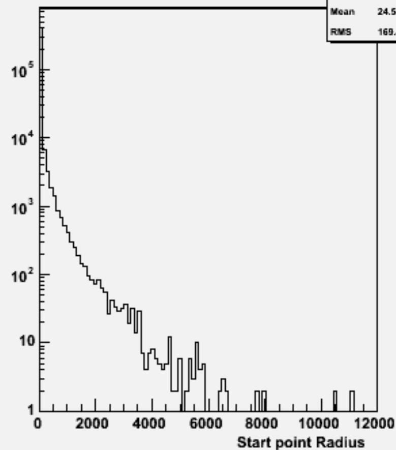
Start point R : w104030 aa_cse1n1_o
