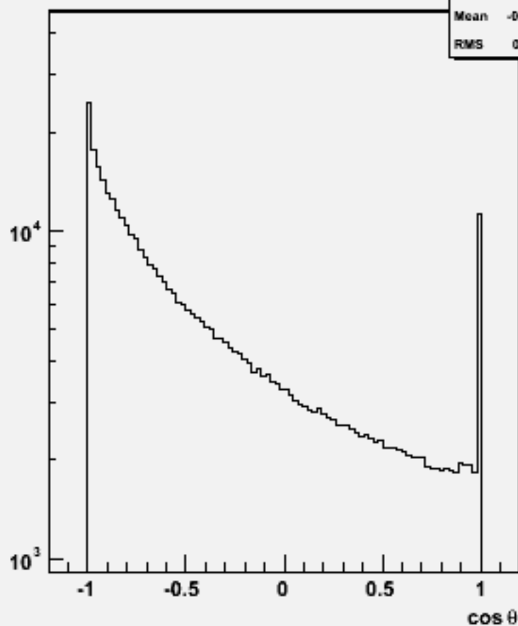
Particle cos \theta : w104030 aa_cse1n1_o
