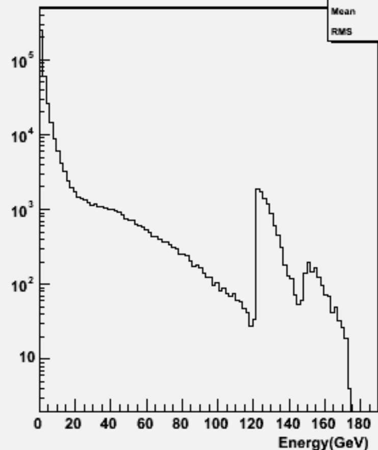
Particle Energy : w104030 aa_cse1n1_o
