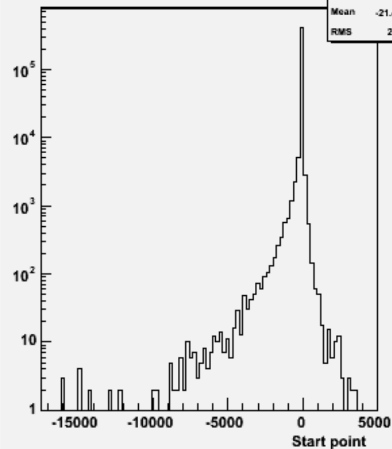
Start point Z : w104030 aa_cse1n1_o
