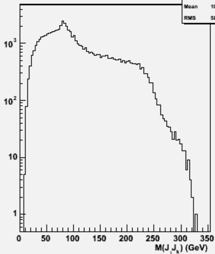
2jets mass(All comb)w104030 aa_cse1n1_o
