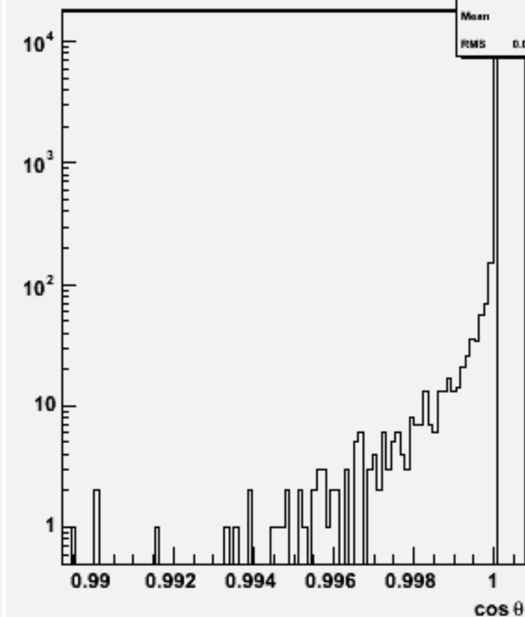
Jet cos \theta (All jets)w104030 aa_cse1n1_o
