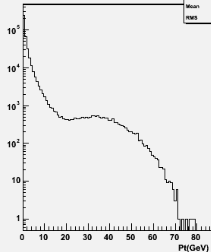
Particle Pt : w104030 aa_cse1n1_o
