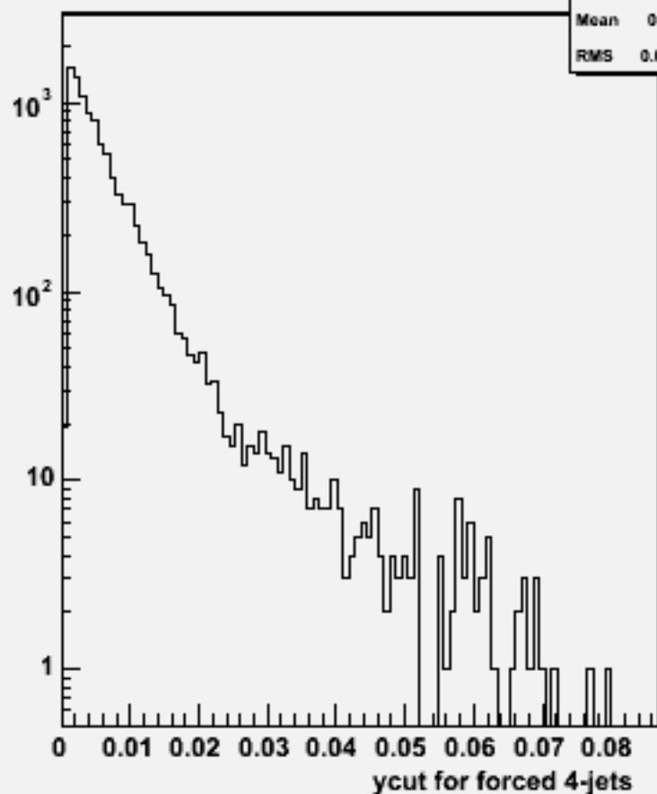
Ycut for 4-jets :w104030 aa_cse1n1_o
