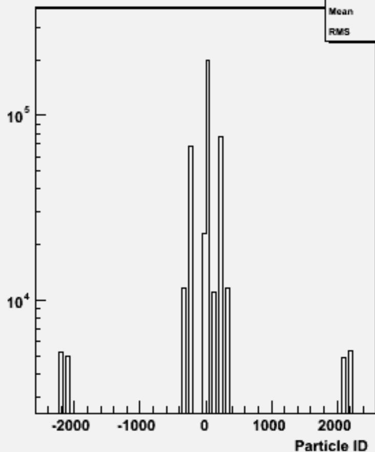
Particle ID : w104030 aa_cse1n1_o
