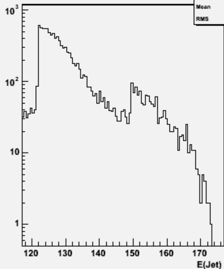
Jet energies(All jets)w104030 aa_cse1n1_o
