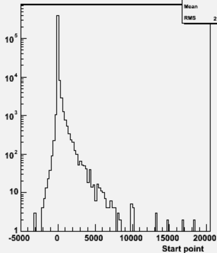
Start point Z : w104029 aa_cse1n1_o
