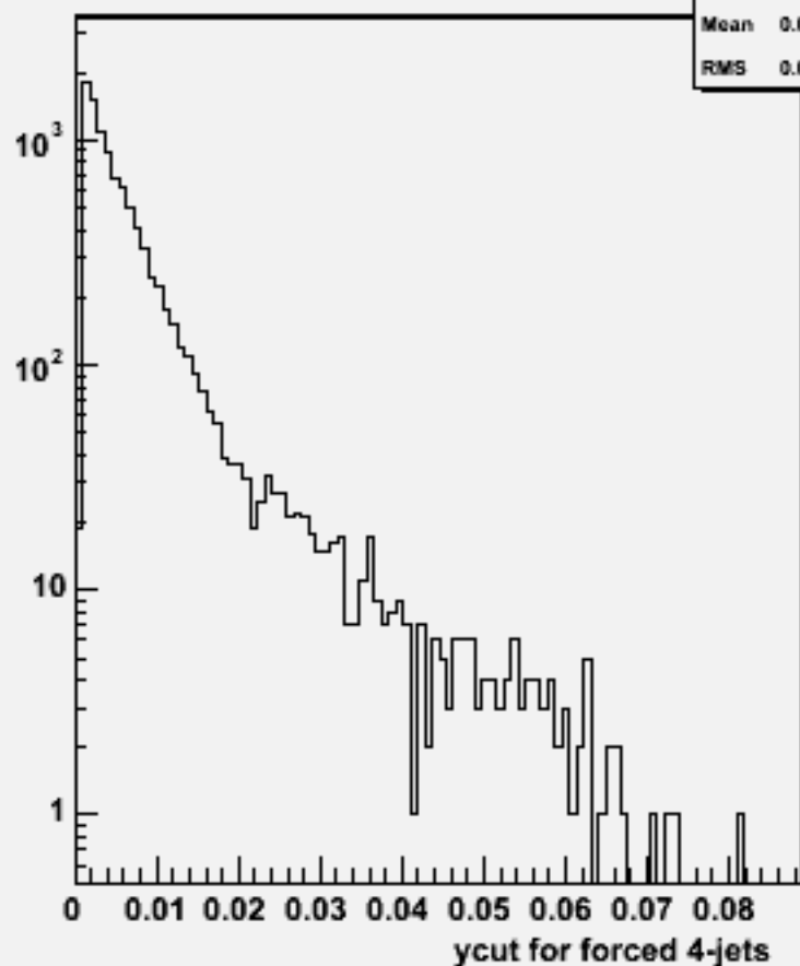
Ycut for 4-jets :w104029 aa_cse1n1_o
