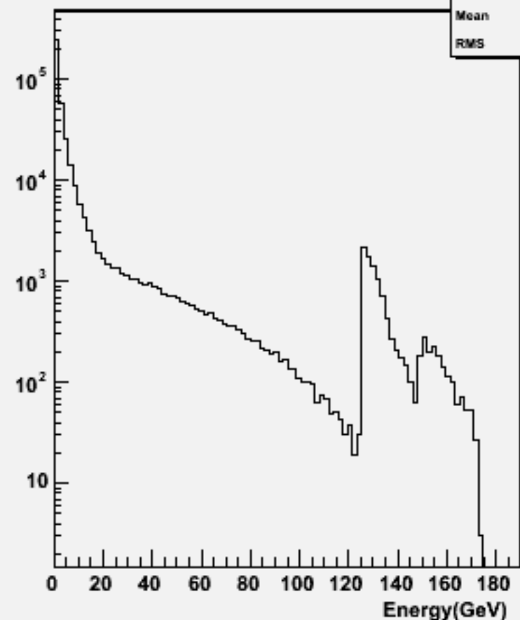
Particle Energy : w104029 aa_cse1n1_o
