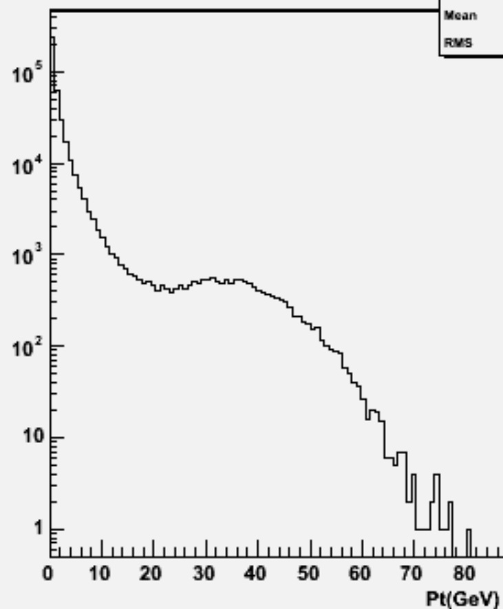
Particle Pt : w104029 aa_cse1n1_o
