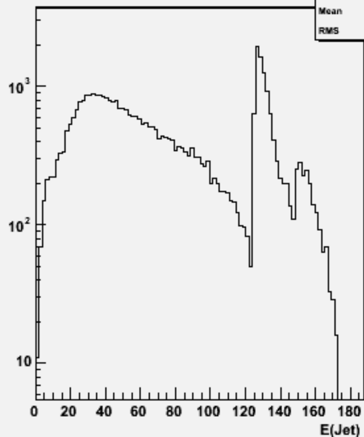
Jet energies(All jets)w104029 aa_cse1n1_o
