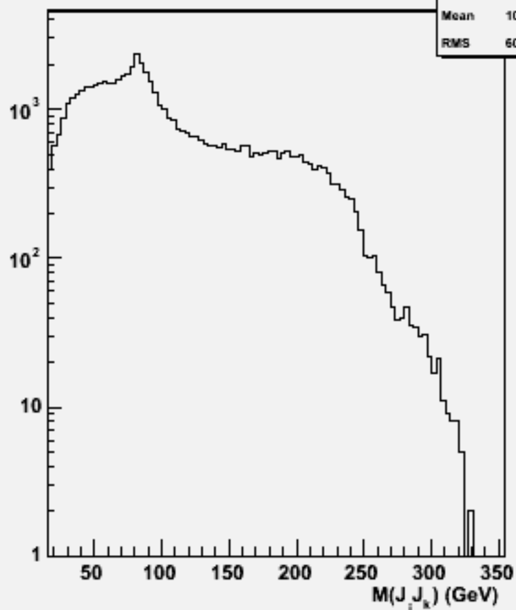
2jets mass(All comb)w104029 aa_cse1n1_o
