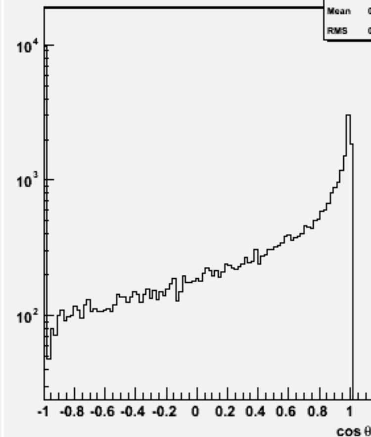
Jet cos \theta (All jets)w104029 aa_cse1n1_o
