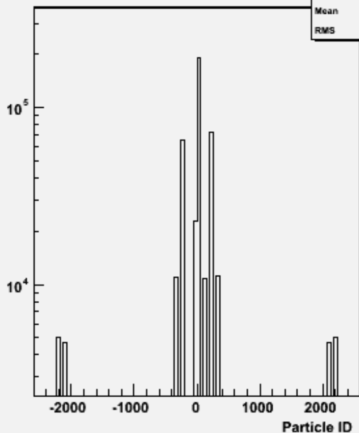
Particle ID : w104029 aa_cse1n1_o
