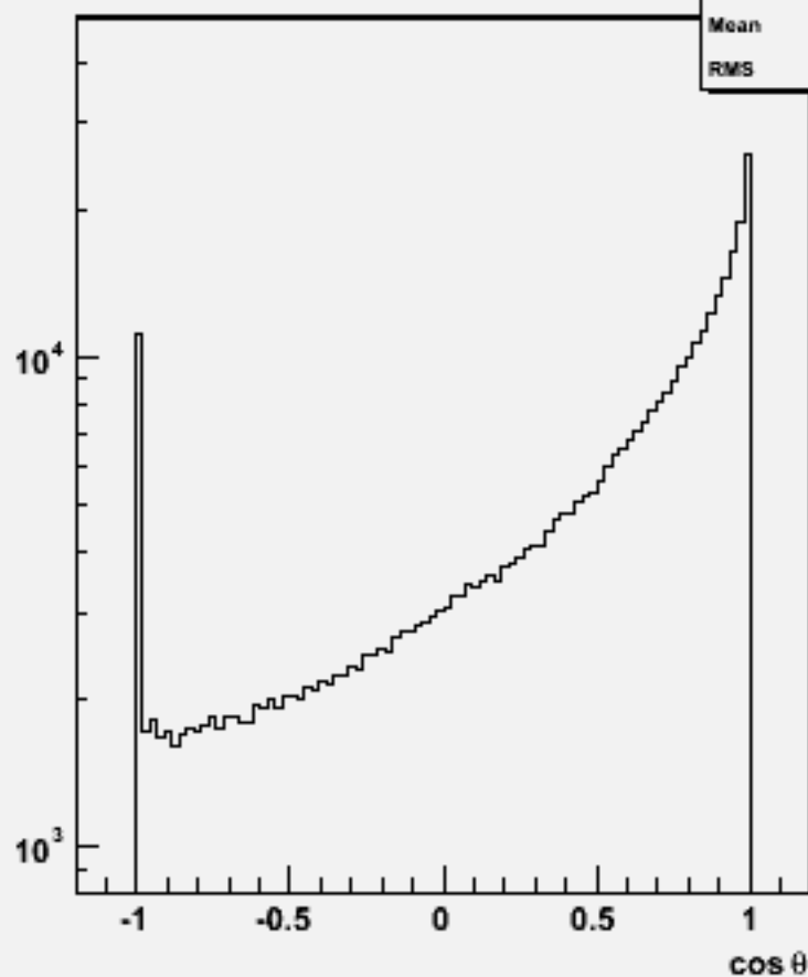
Particle cos \theta : w104029 aa_cse1n1_o
