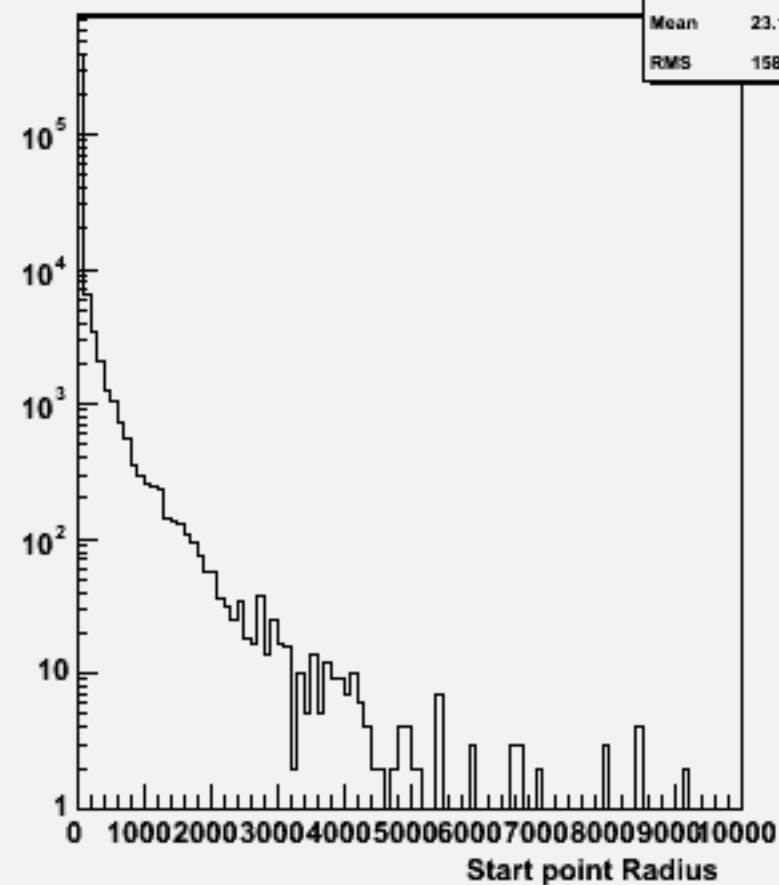
Start point R : w104029 aa_cse1n1_o
