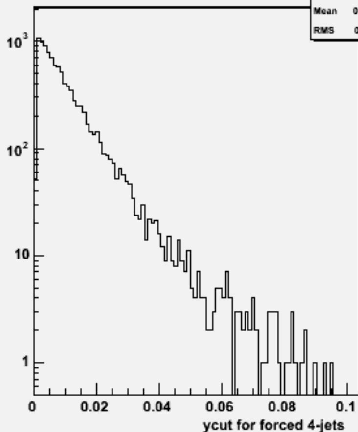
Ycut for 4-jets :w104028 aa_cse1n1_o
