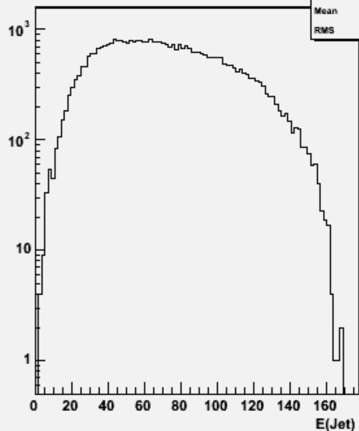
Jet energies(All jets)w104028 aa_cse1n1_o
