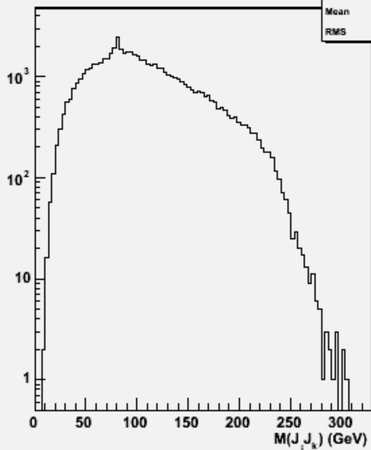
2jets mass(All comb)w104028 aa_cse1n1_o
