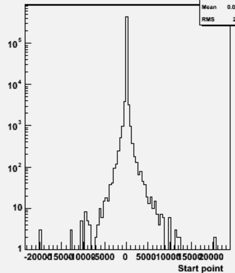
Start point Z : w104028 aa_cse1n1_o
