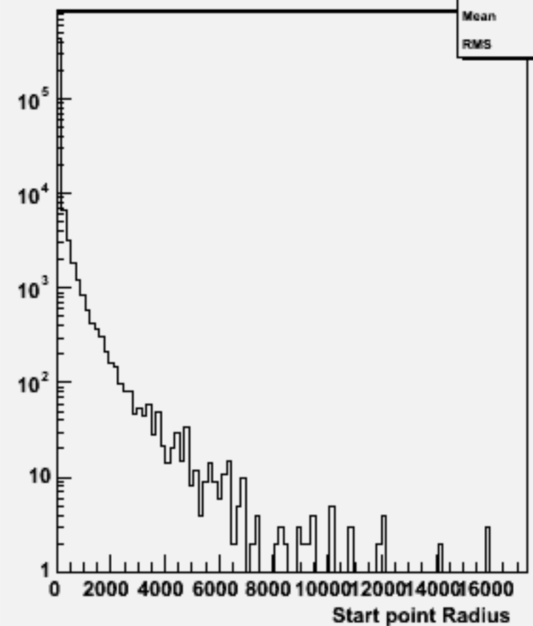
Start point R : w104028 aa_cse1n1_o
