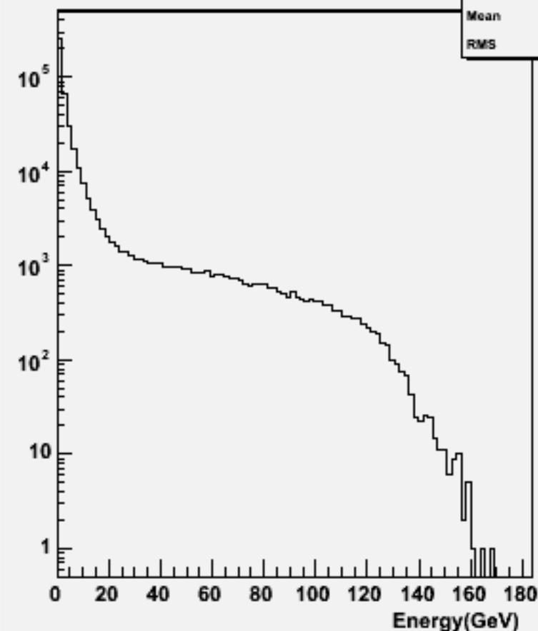
Particle Energy : w104028 aa_cse1n1_o
