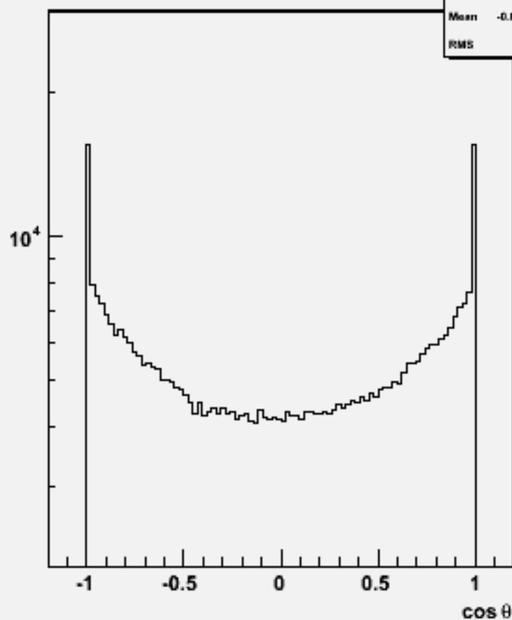
Particle cos \theta : w104028 aa_cse1n1_o
