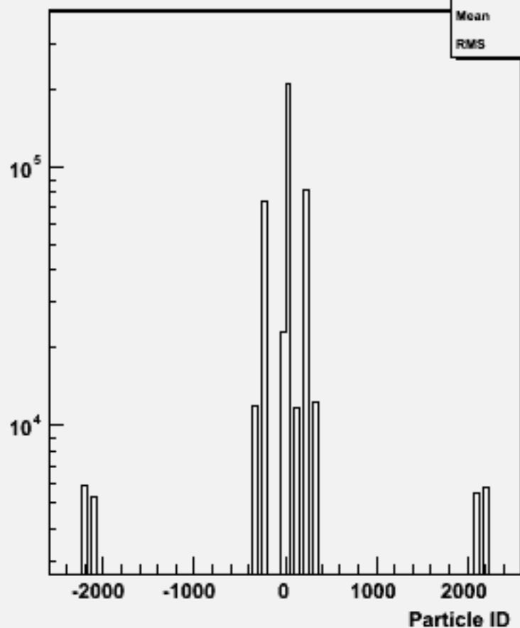
Particle ID : w104028 aa_cse1n1_o
