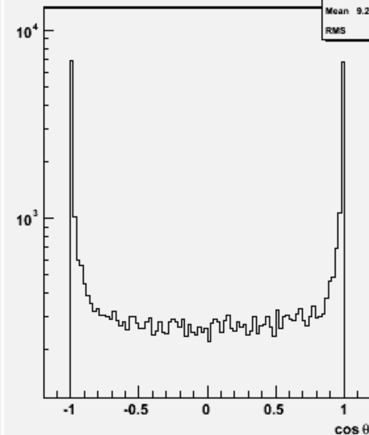
Jet cos \theta (All jets)w104028 aa_cse1n1_o
