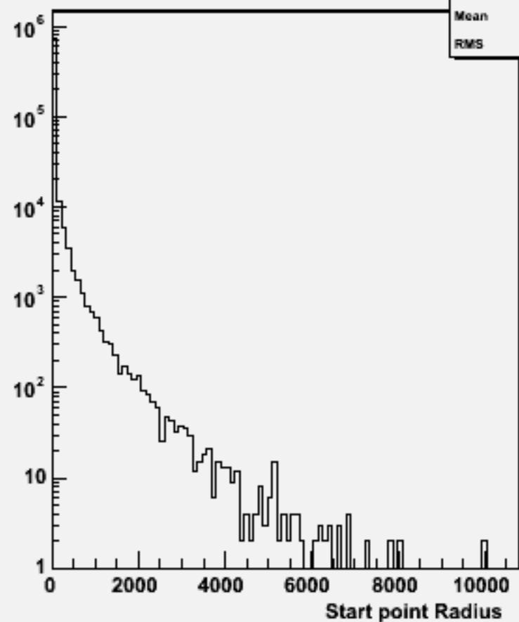
Start point R : w104026 aa_udsc_o
