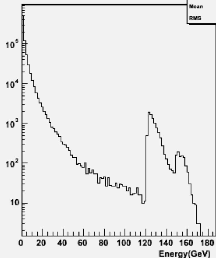
Particle Energy : w104026 aa_udsc_o
