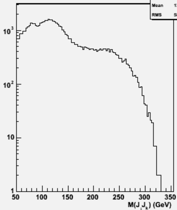
2jets mass(All comb)w104026 aa_udsc_o
