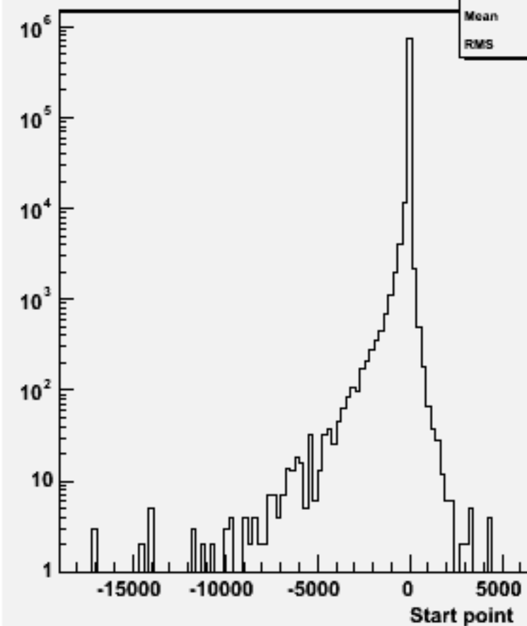
Start point Z : w104026 aa_udsc_o
