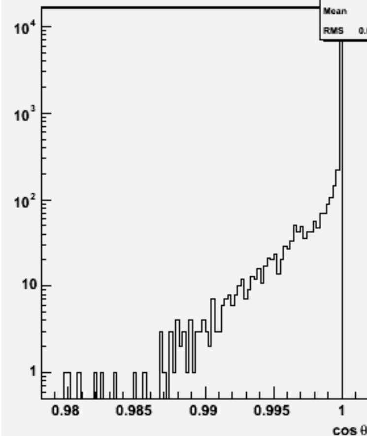
Jet cos \theta (All jets)w104026 aa_udsc_o
