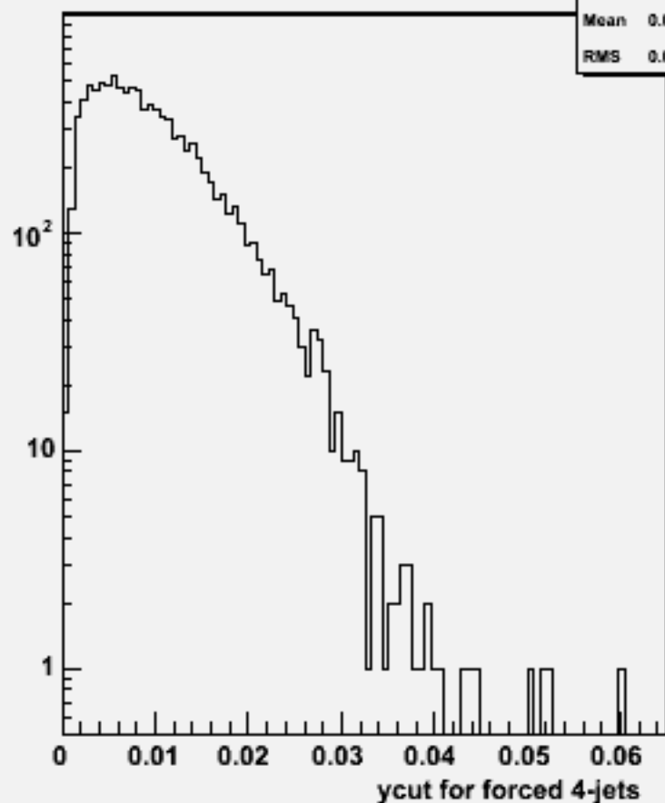
Ycut for 4-jets :w104026 aa_udsc_o
