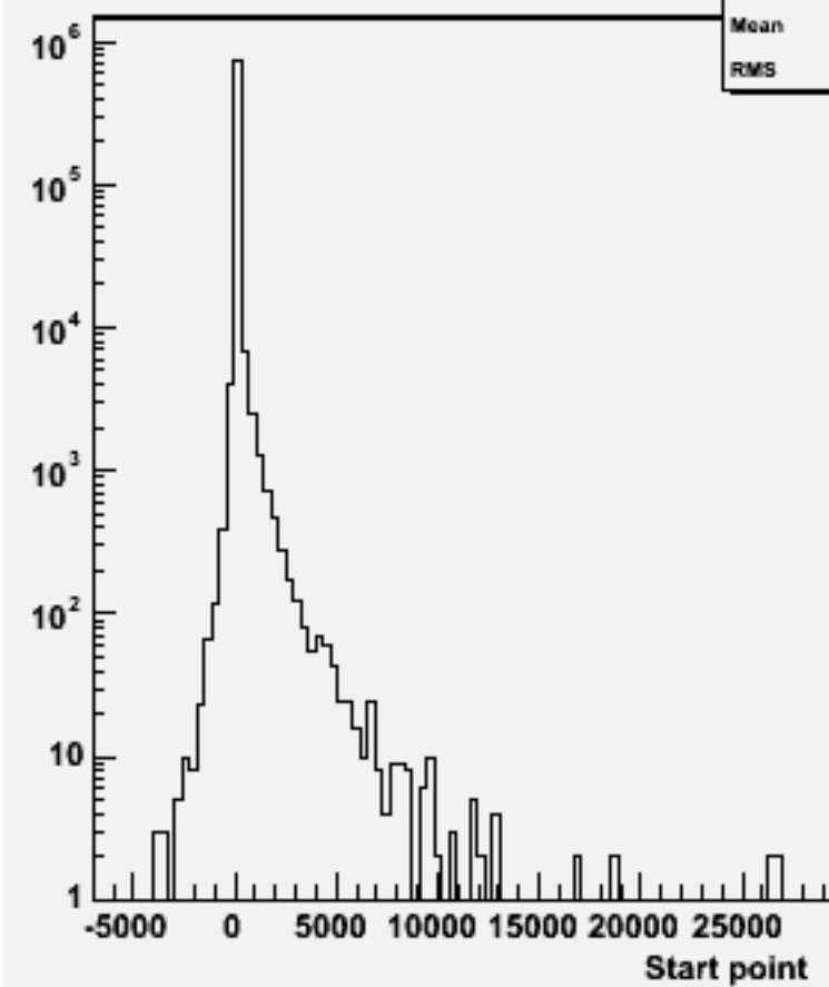
Start point Z : w104025 aa_udsc_o
