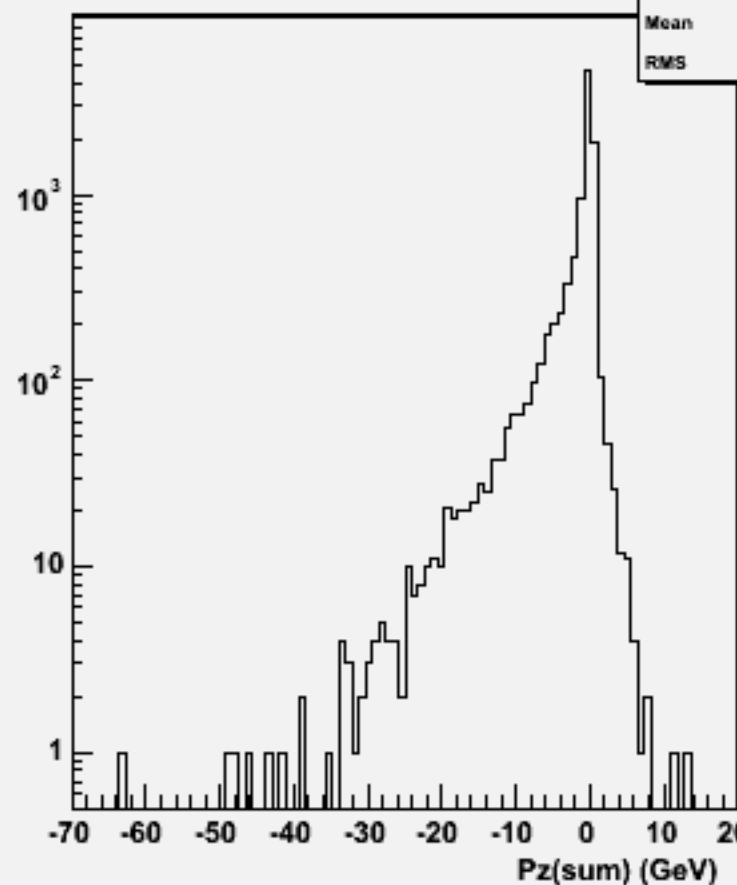
Pz Sum: w104025 aa_udsc_o
