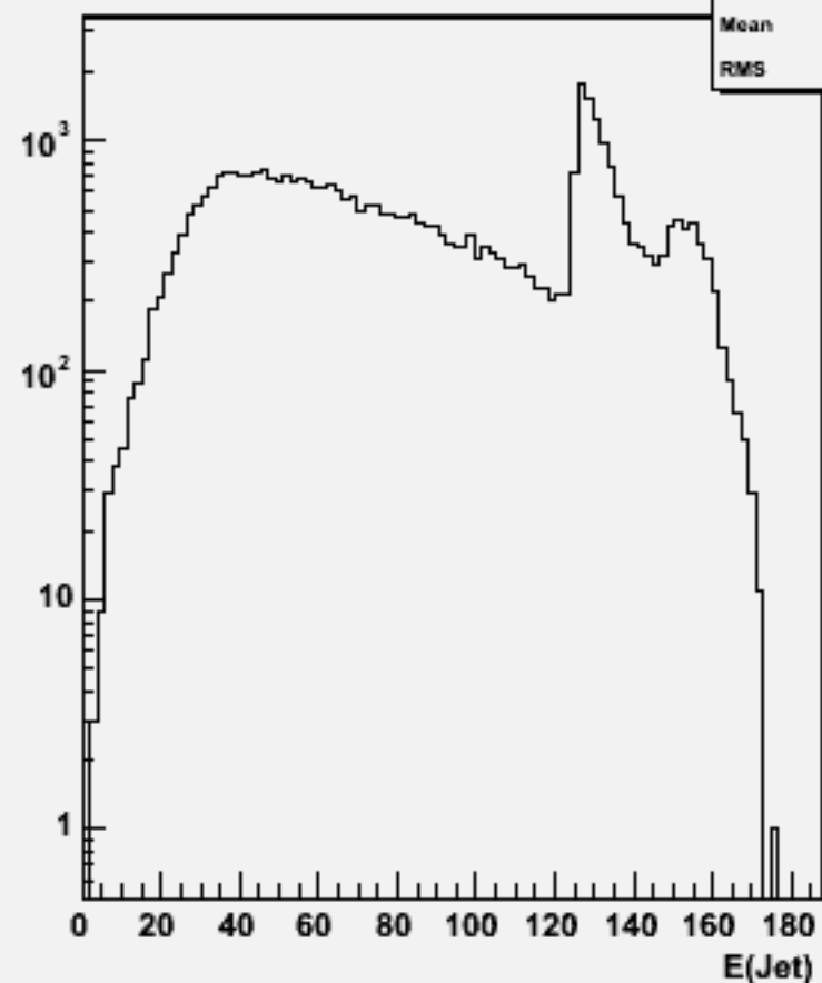
Jet energies(All jets)w104025 aa_udsc_o
