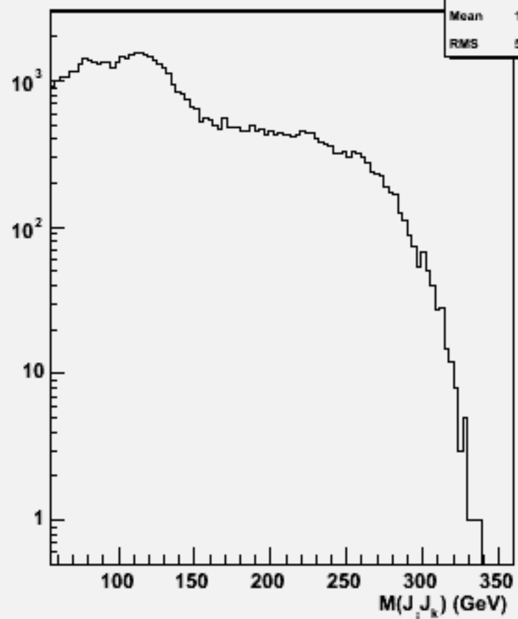
2jets mass(All comb)w104025 aa_udsc_o
