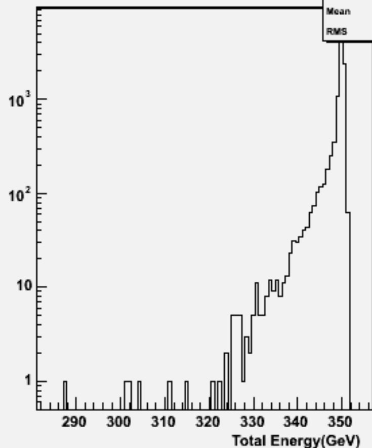
Total Energy (inc. \nu ): w104025 aa_udsc_o
