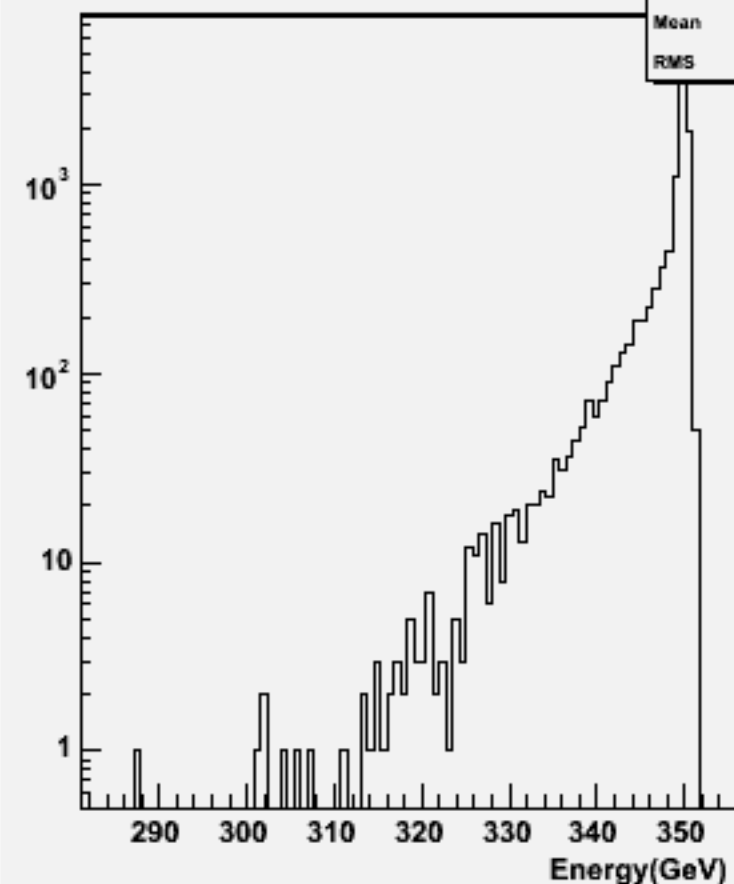
Total Energy (w/o \nu ): w104025 aa_udsc_o
