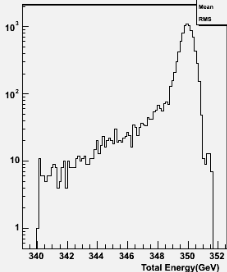
Total Energy (inc. \nu ): w104025 aa_udsc_o
