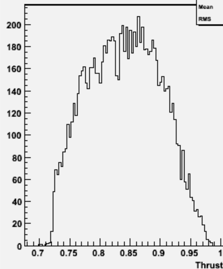
Thrust w104025 aa_udsc_o
