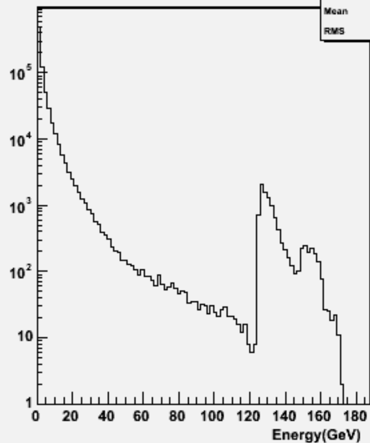
Particle Energy : w104025 aa_udsc_o
