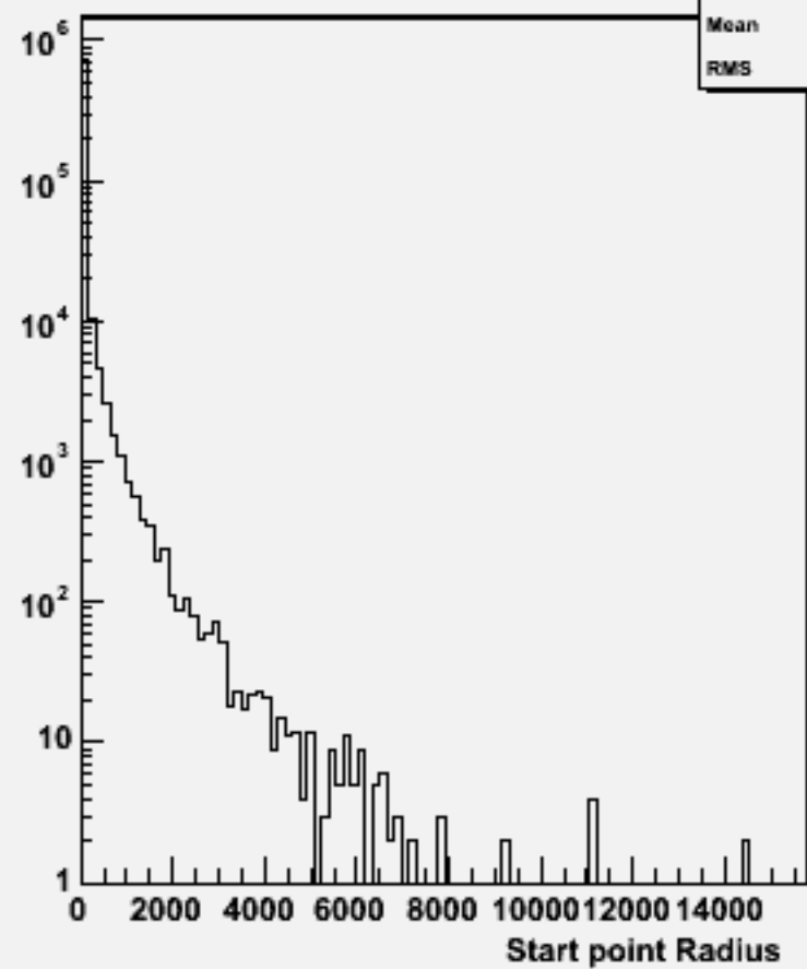
Start point R : w104025 aa_udsc_o
