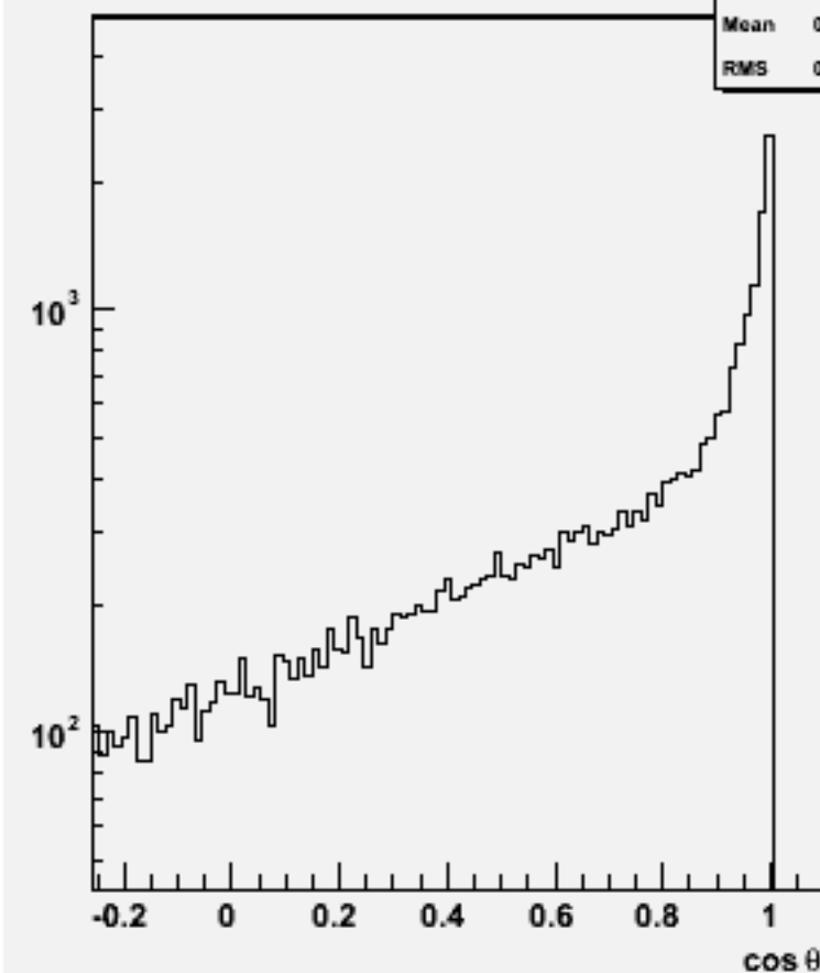
Jet cos \theta (All jets)w104025 aa_udsc_o
