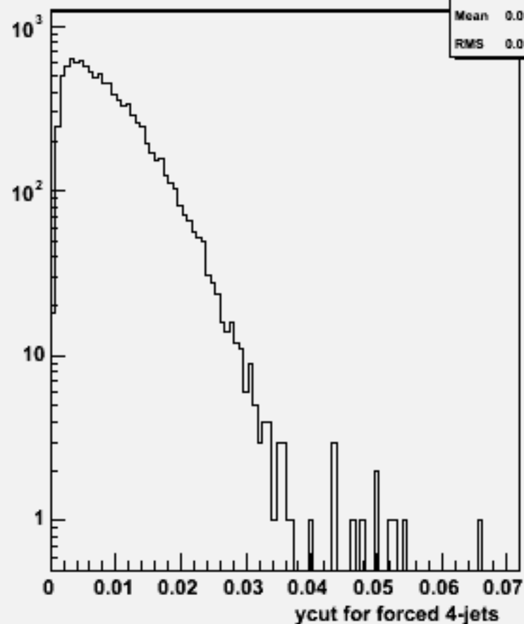
Ycut for 4-jets :w104025 aa_udsc_o
