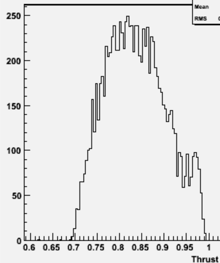
Thrust w104022 aa_uddu_o
