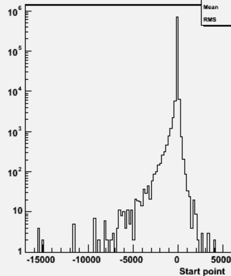
Start point Z : w104022 aa_uddu_o
