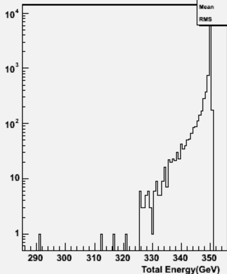
Total Energy (inc. \nu ): w104022 aa_uddu_o
