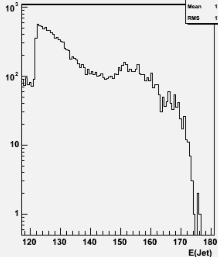
Jet energies(All jets)w104022 aa_uddu_o
