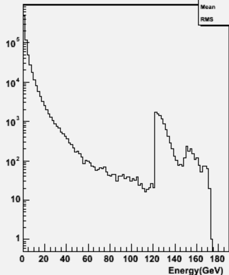
Particle Energy : w104022 aa_uddu_o
