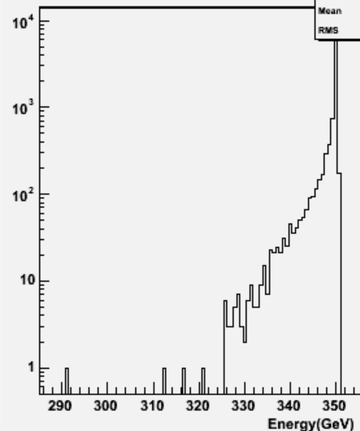
Total Energy (w/o \nu ): w104022 aa_uddu_o
