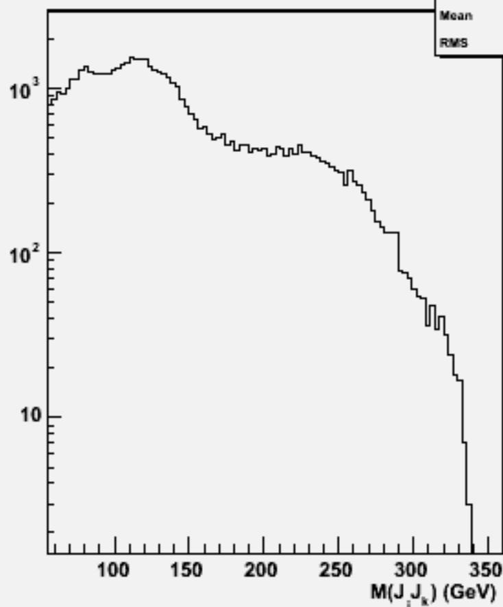
2jets mass(All comb)w104022 aa_uddu_o
