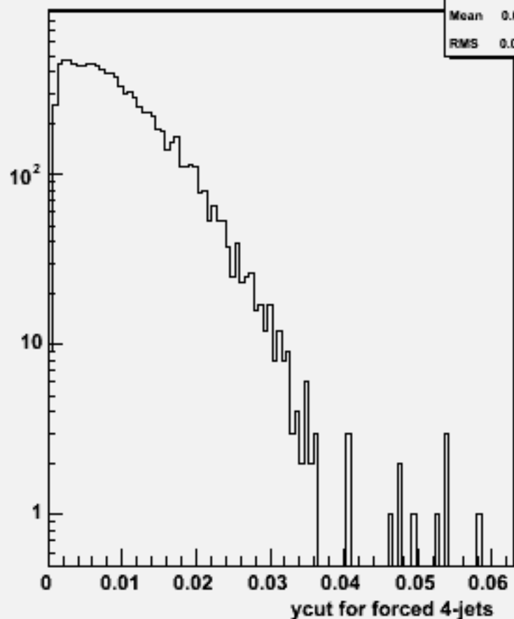
Ycut for 4-jets :w104022 aa_uddu_o
