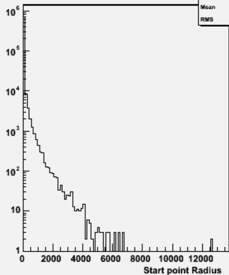
Start point R : w104022 aa_uddu_o
