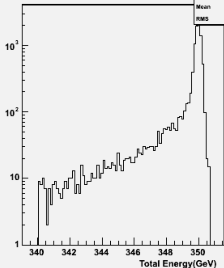
Total Energy (inc. \nu ): w104022 aa_uddu_o
