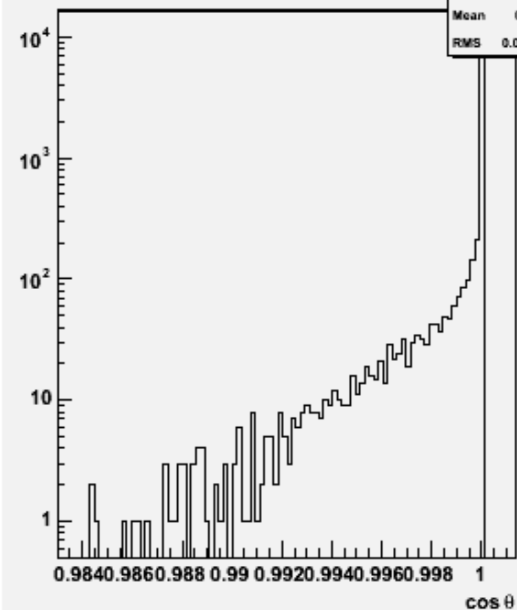
Jet cos \theta (All jets)w104022 aa_uddu_o
