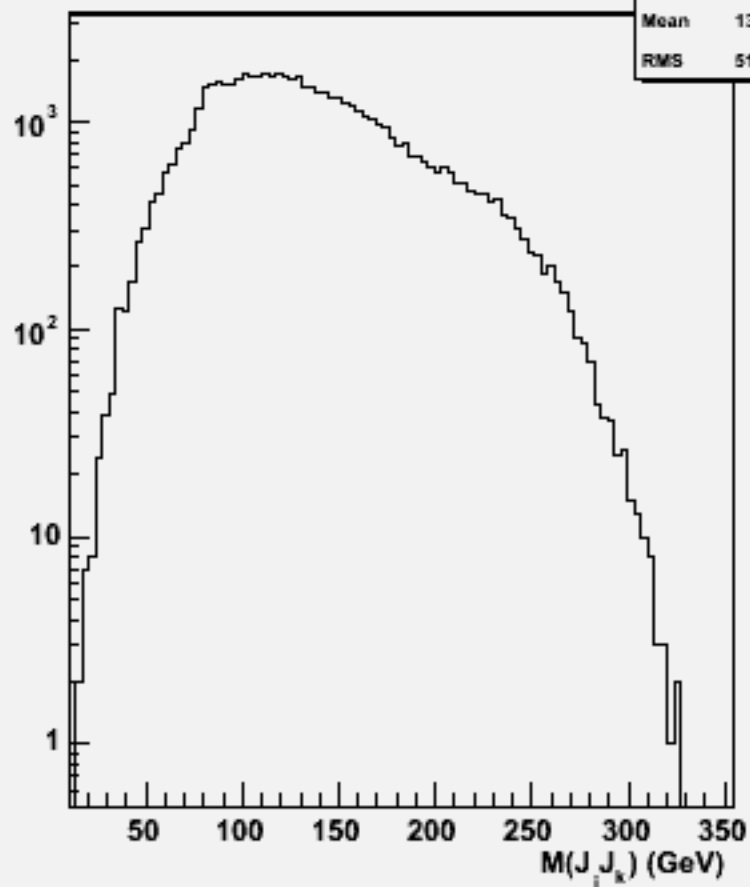
2jets mass(All comb)w104020 aa_uddu_o
