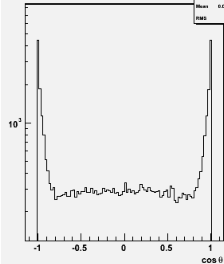
Jet cos \theta (All jets)w104020 aa_uddu_o
