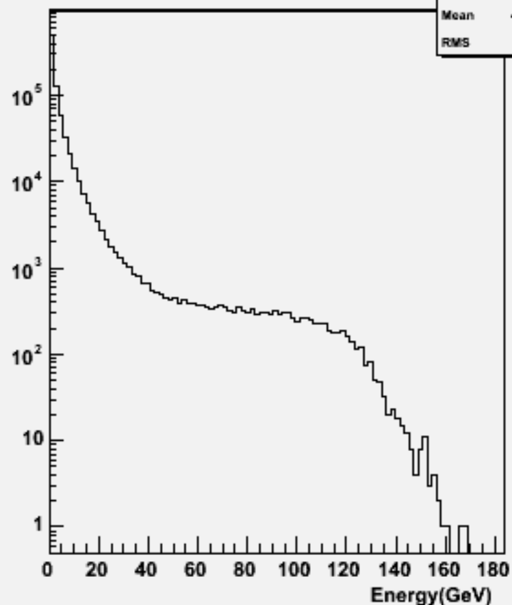
Particle Energy : w104020 aa_uddu_o
