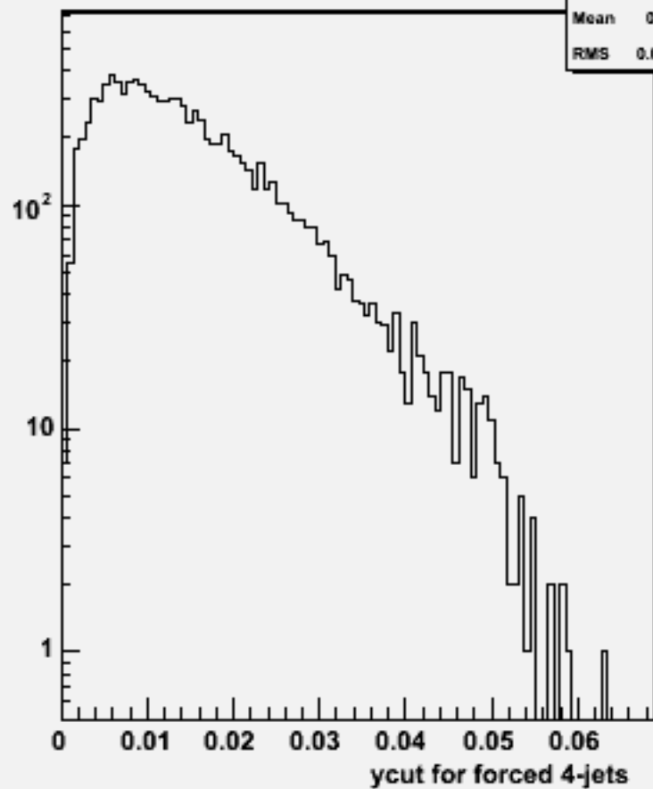
Ycut for 4-jets :w104020 aa_uddu_o
