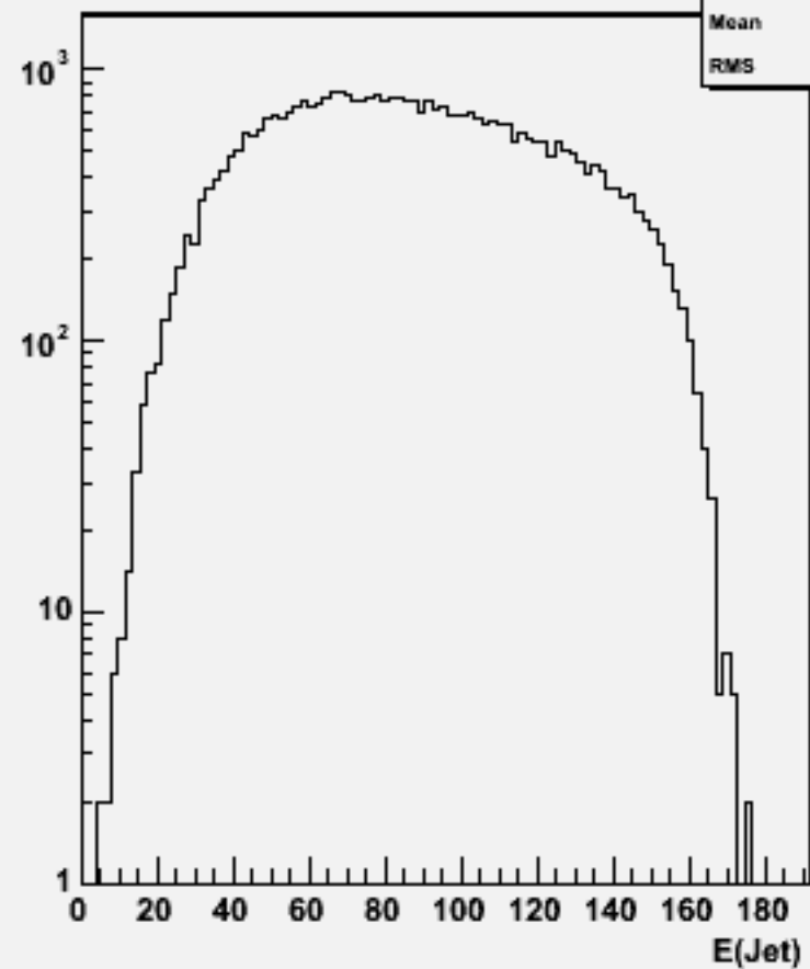
Jet energies(All jets)w104020 aa_uddu_o
