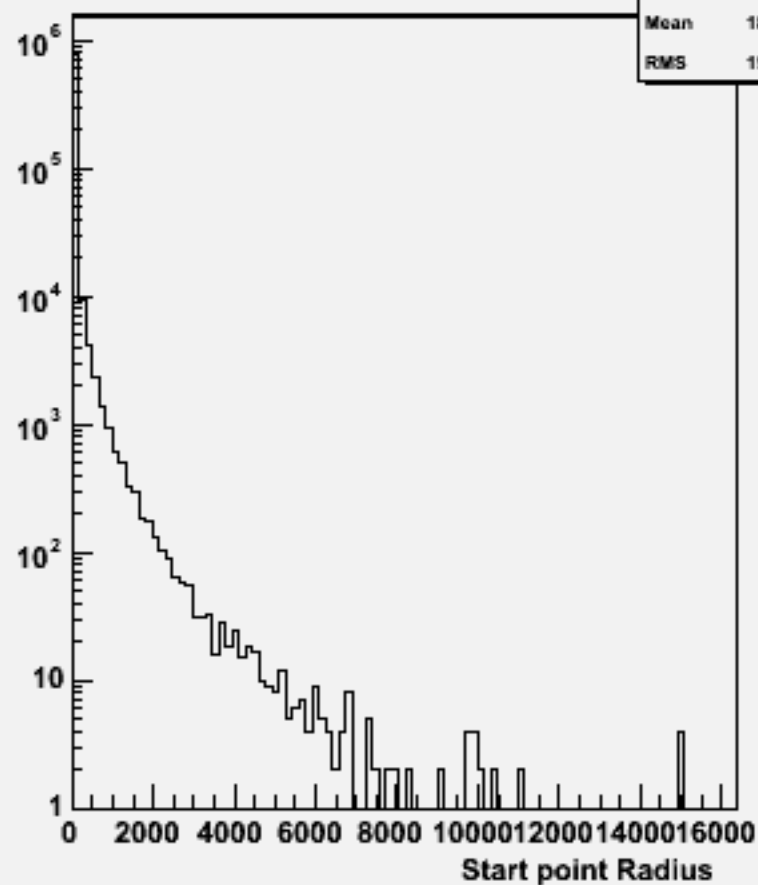
Start point R : w104020 aa_uddu_o
