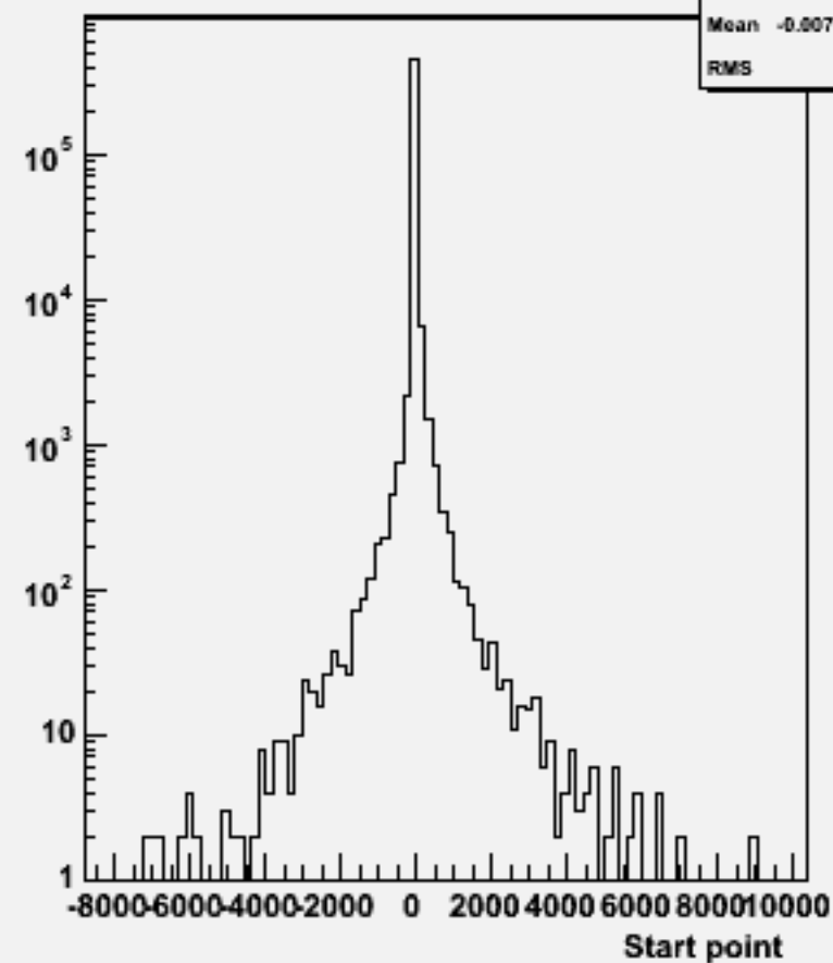
Start point Z : w104016 aa_ude3n3_o
