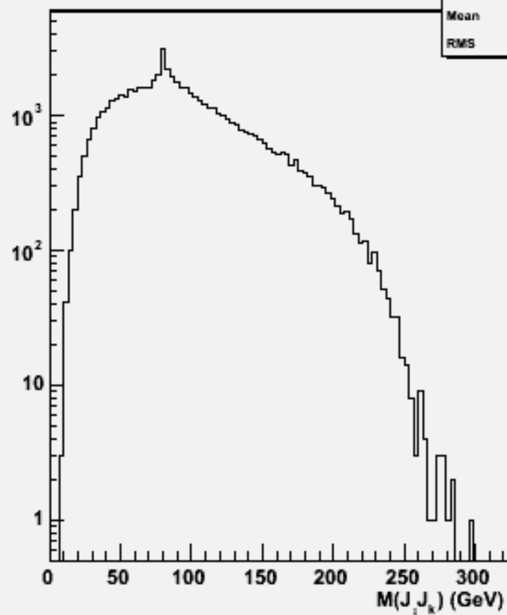
2jets mass(All comb)w104016 aa_ude3n3_o
