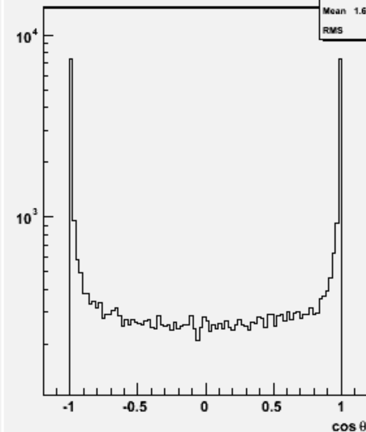
Jet cos \theta (All jets)w104016 aa_ude3n3_o
