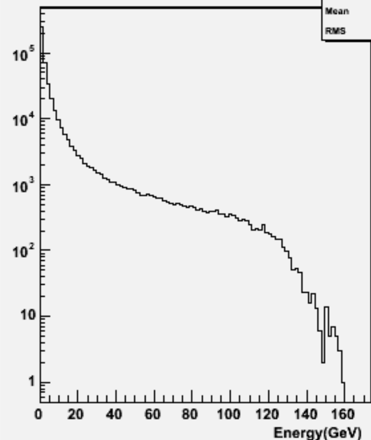
Particle Energy : w104016 aa_ude3n3_o
