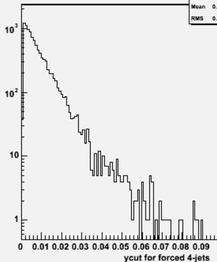
Ycut for 4-jets :w104016 aa_ude3n3_o
