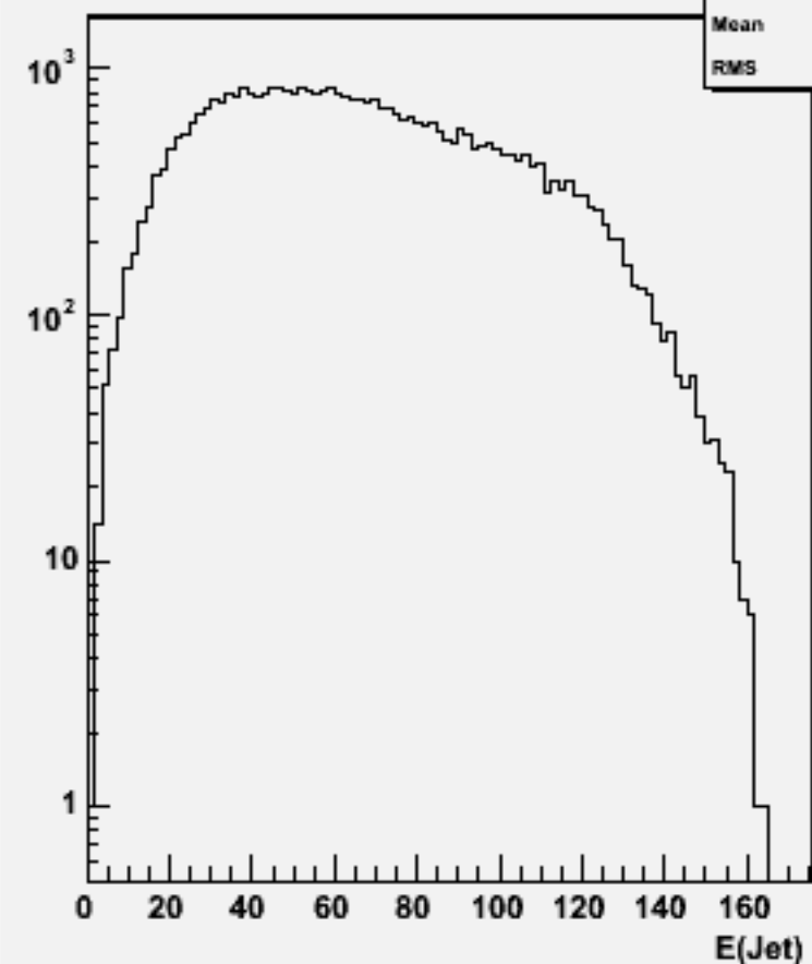
Jet energies(All jets)w104016 aa_ude3n3_o
