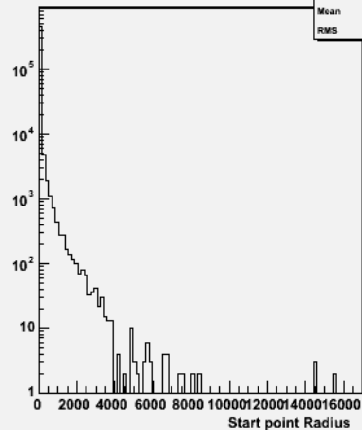
Start point R : w104016 aa_ude3n3_o
