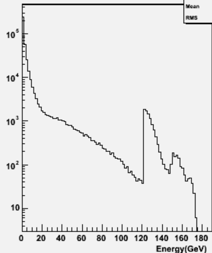
Particle Energy : w104014 aa_ude2n2_o
