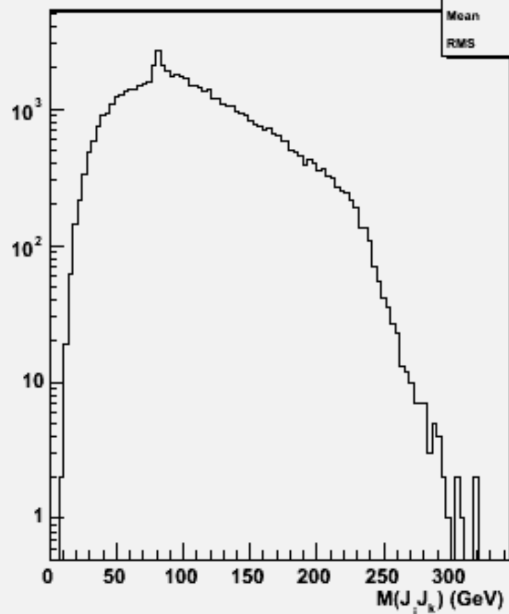
2jets mass(All comb)w104012 aa_ude2n2_o
