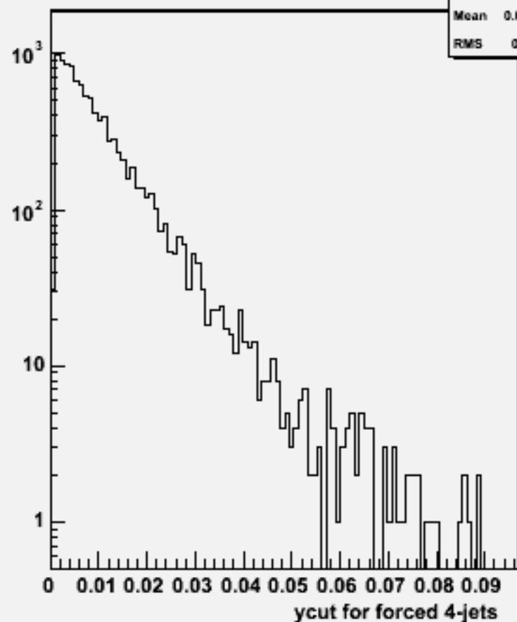
Ycut for 4-jets :w104012 aa_ude2n2_o
