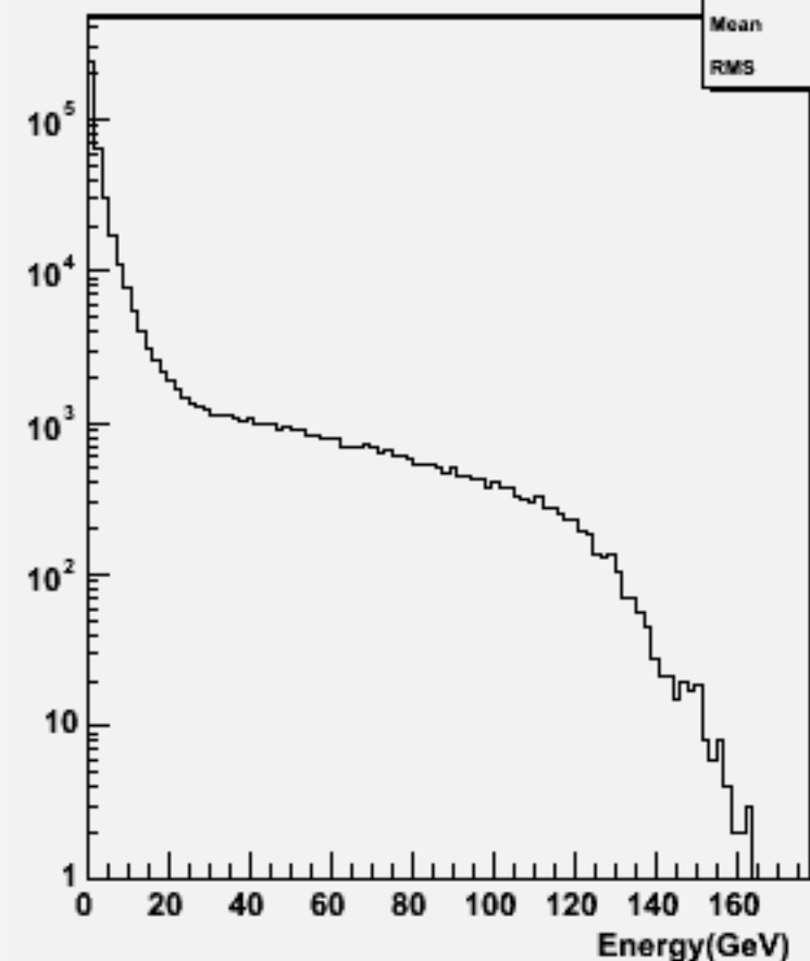
Particle Energy : w104012 aa_ude2n2_o
