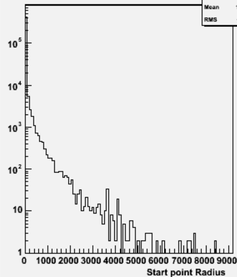
Start point R : w104012 aa_ude2n2_o
