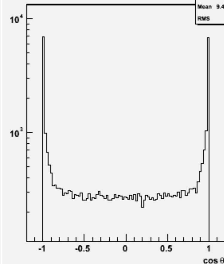
Jet cos \theta (All jets)w104012 aa_ude2n2_o
