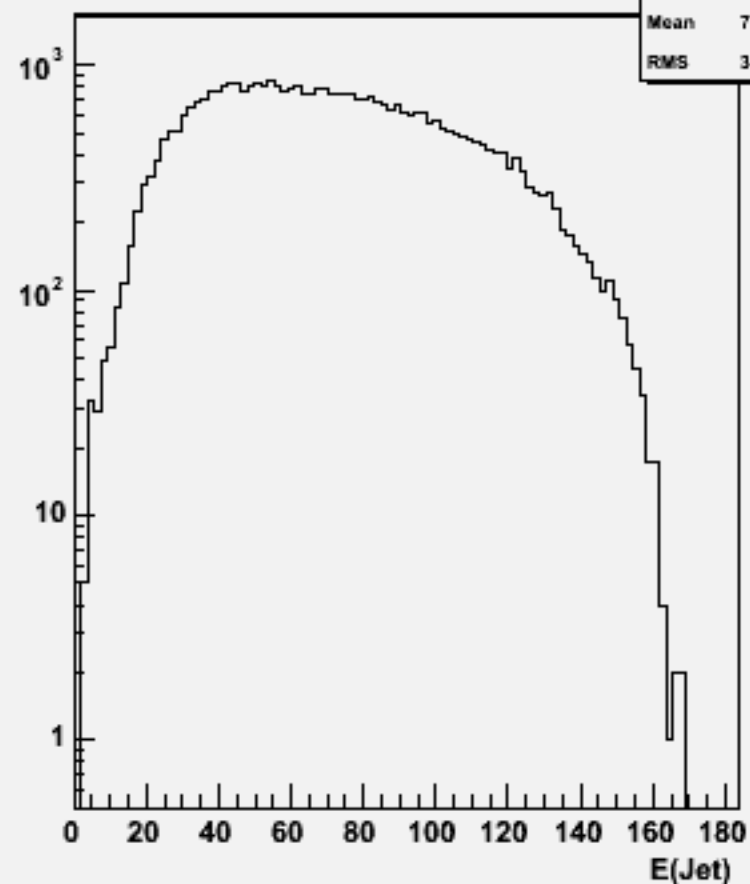
Jet energies(All jets)w104012 aa_ude2n2_o
