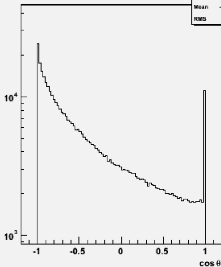
Particle cos \theta : w104010 aa_ude1n1_o
