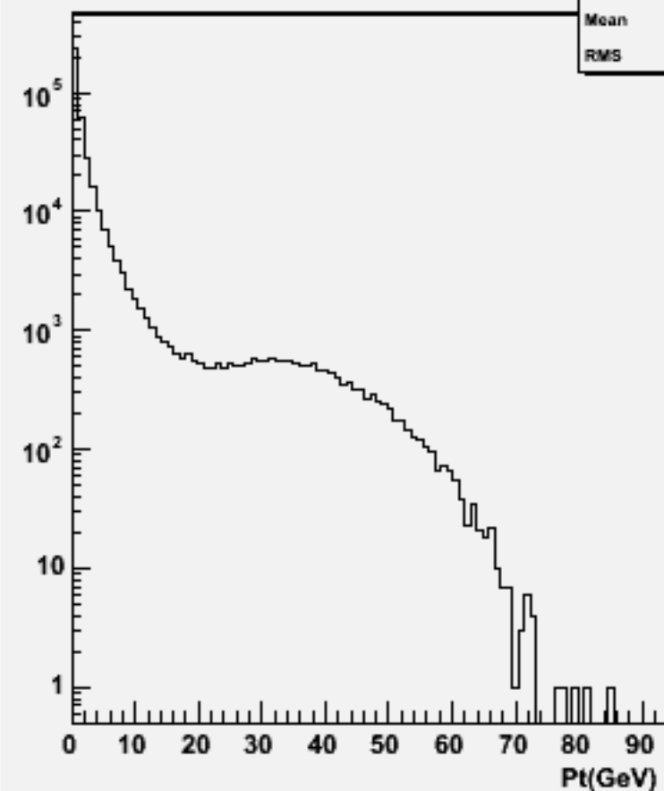
Particle Pt : w104010 aa_ude1n1_o
