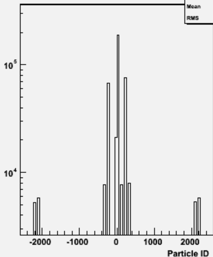
Particle ID : w104010 aa_ude1n1_o
