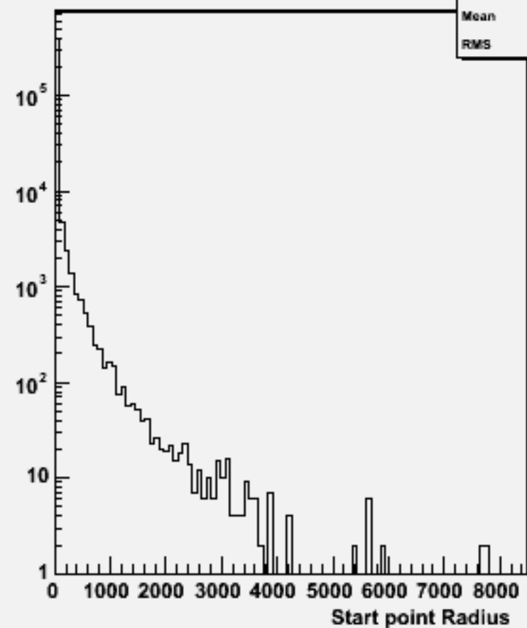
Start point R : w104010 aa_ude1n1_o
