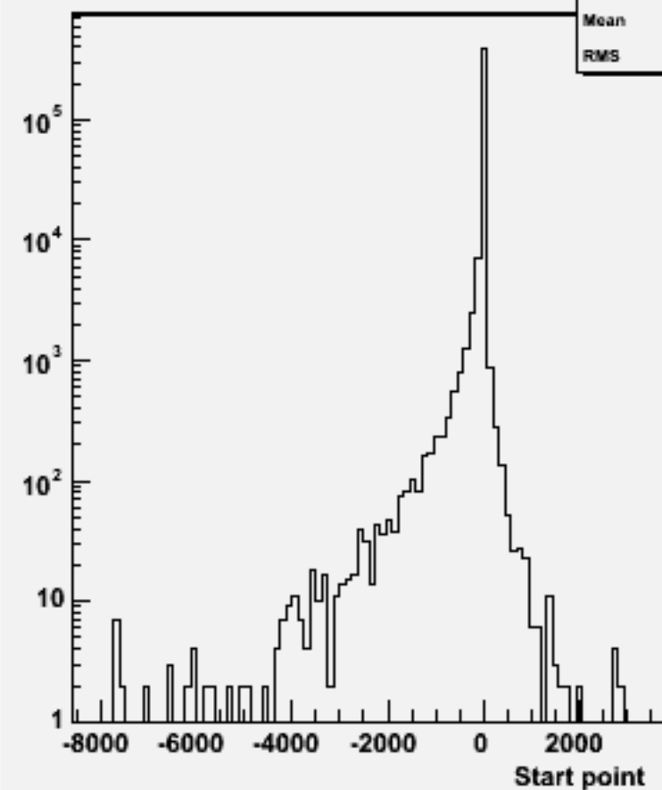
Start point Z : w104010 aa_ude1n1_o
