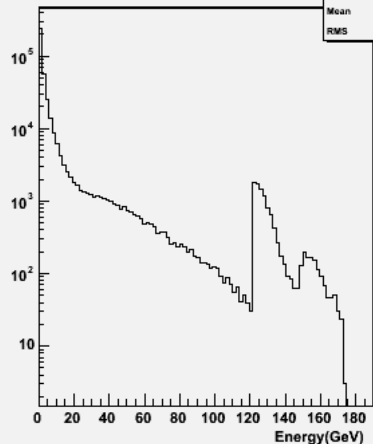
Particle Energy : w104010 aa_ude1n1_o
