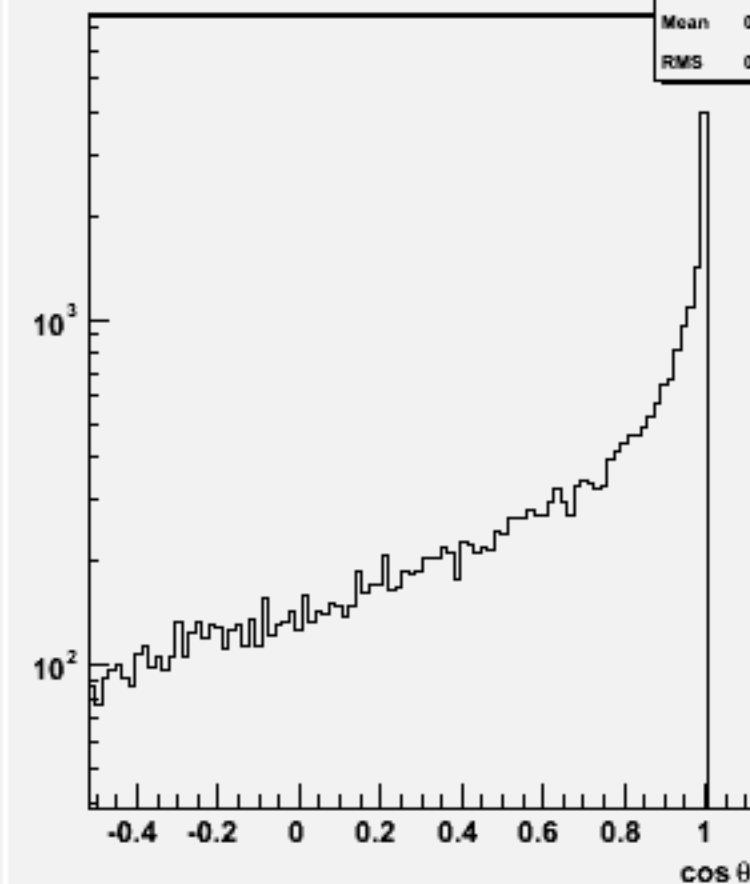
Jet cos \theta (All jets)w104009 aa_ude1n1_o
