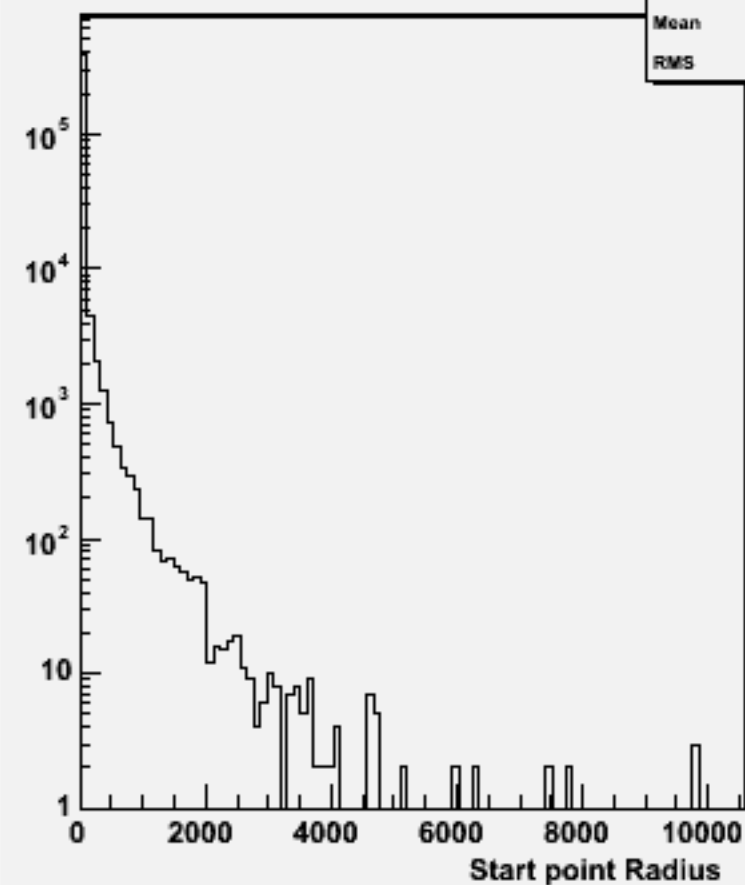
Start point R : w104009 aa_ude1n1_o
