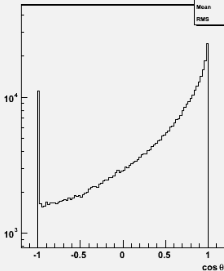
Particle cos \theta : w104009 aa_ude1n1_o
