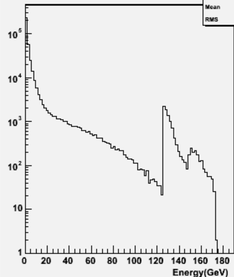
Particle Energy : w104009 aa_ude1n1_o
