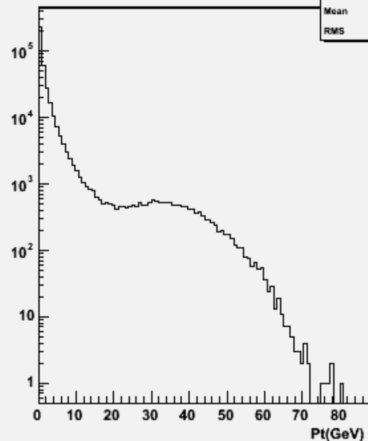
Particle Pt : w104009 aa_ude1n1_o
