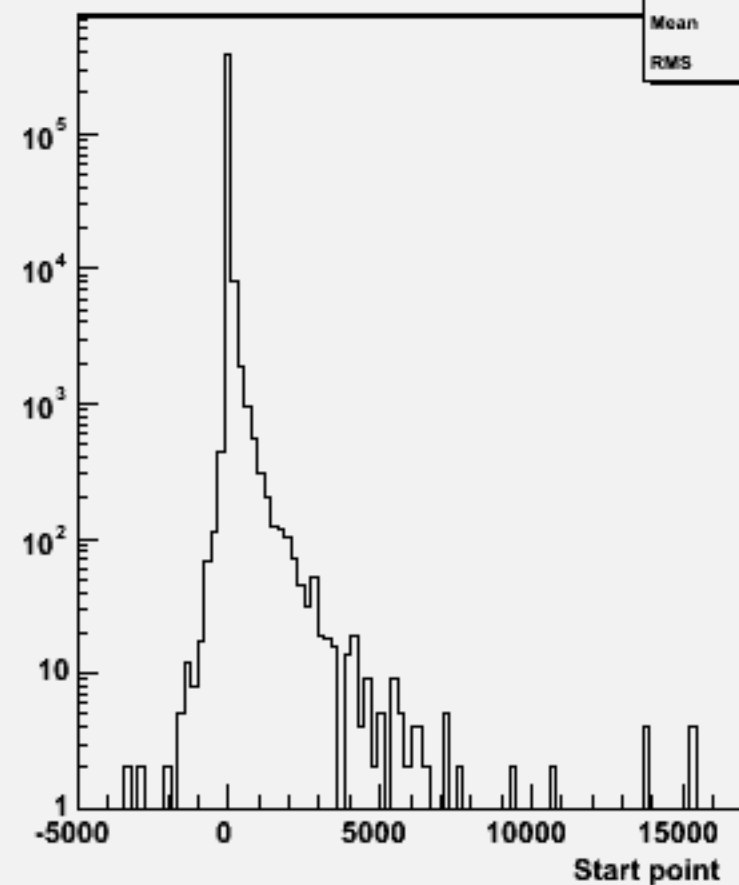
Start point Z : w104009 aa_ude1n1_o
