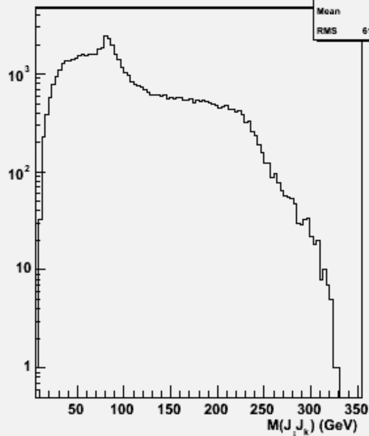
2jets mass(All comb)w104009 aa_ude1n1_o
