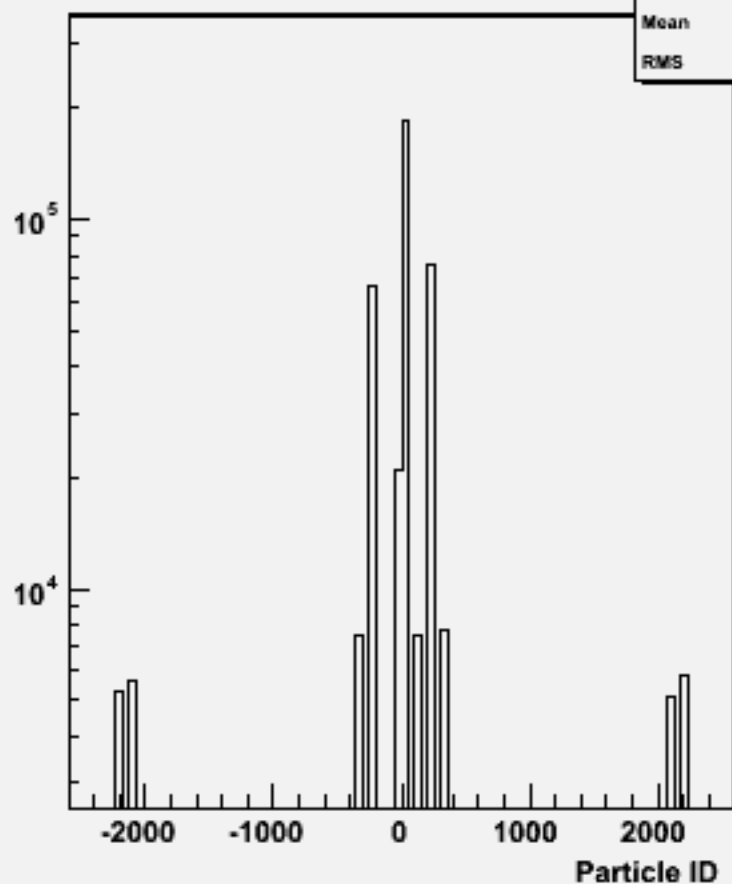
Particle ID : w104009 aa_ude1n1_o
