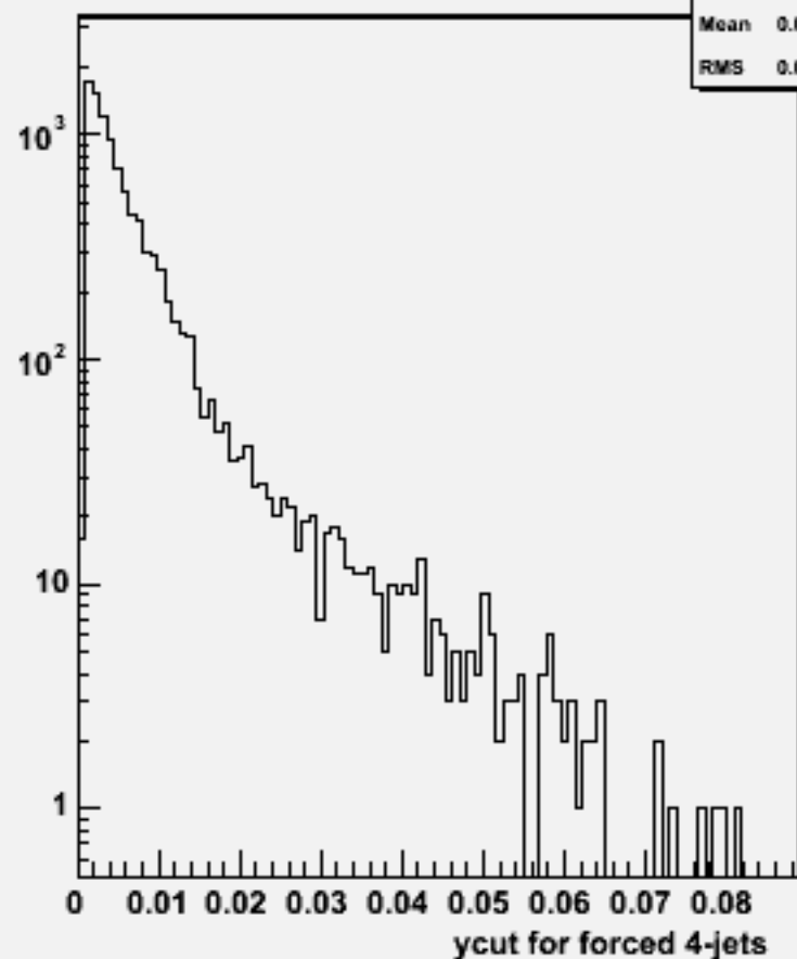
Ycut for 4-jets :w104009 aa_ude1n1_o
