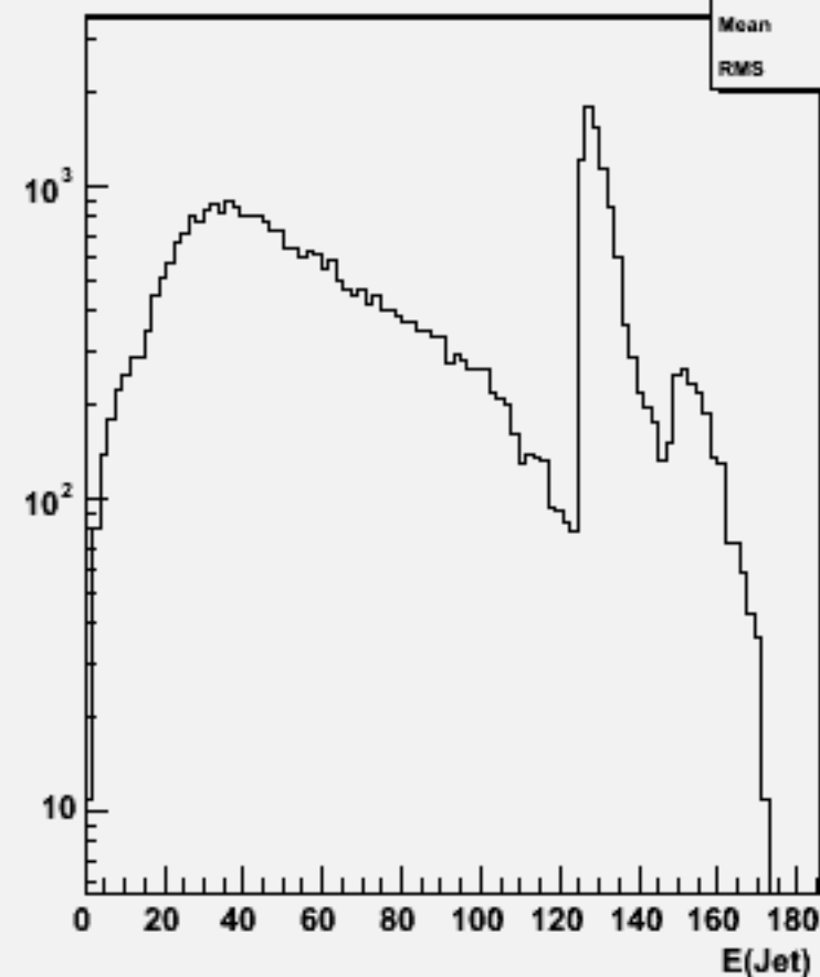
Jet energies(All jets)w104009 aa_ude1n1_o
