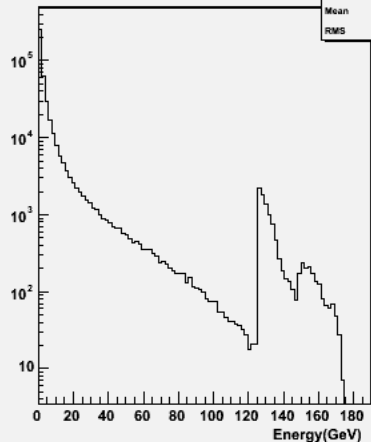
Particle Energy : w104005 aa_n3e3sc_o
