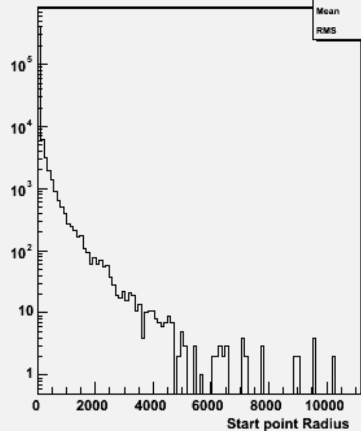
Start point R : w104005 aa_n3e3sc_o
