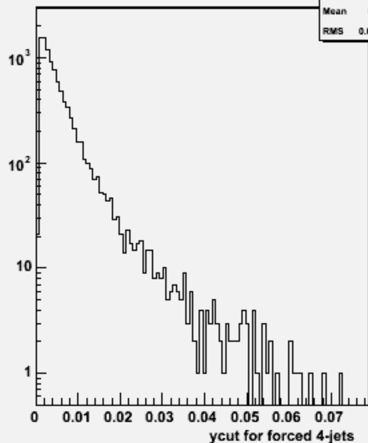
Ycut for 4-jets :w104005 aa_n3e3sc_o
