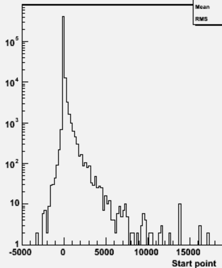
Start point Z : w104005 aa_n3e3sc_o
