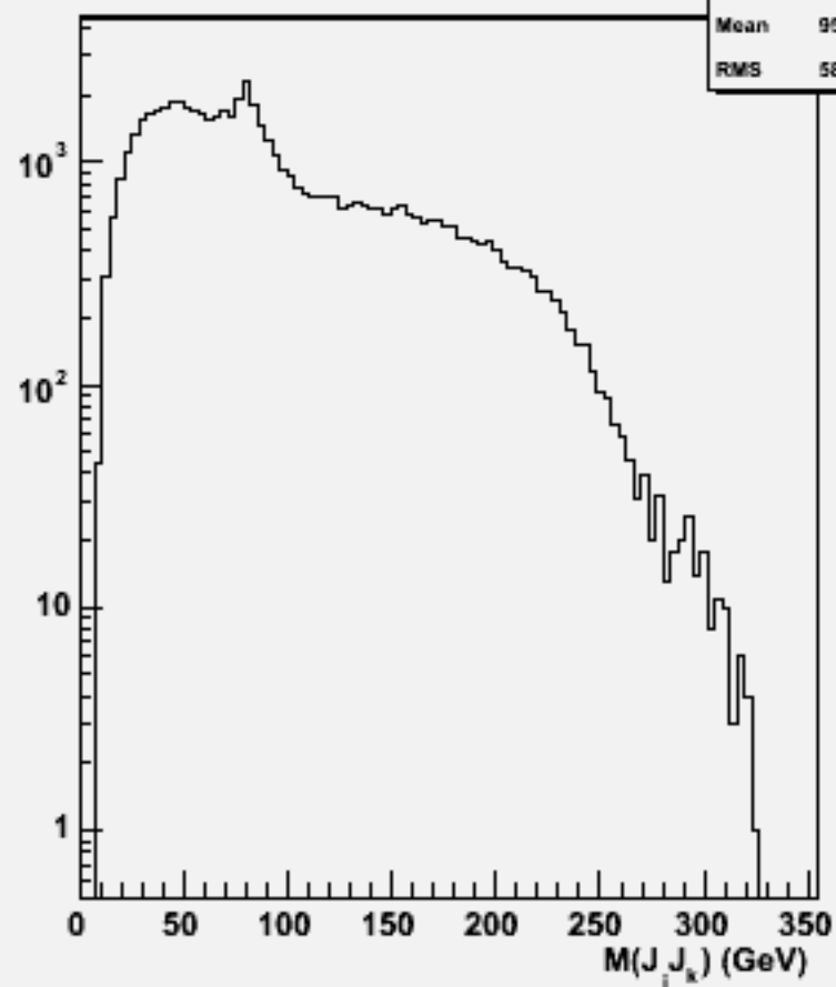
2jets mass(All comb)w104005 aa_n3e3sc_o
