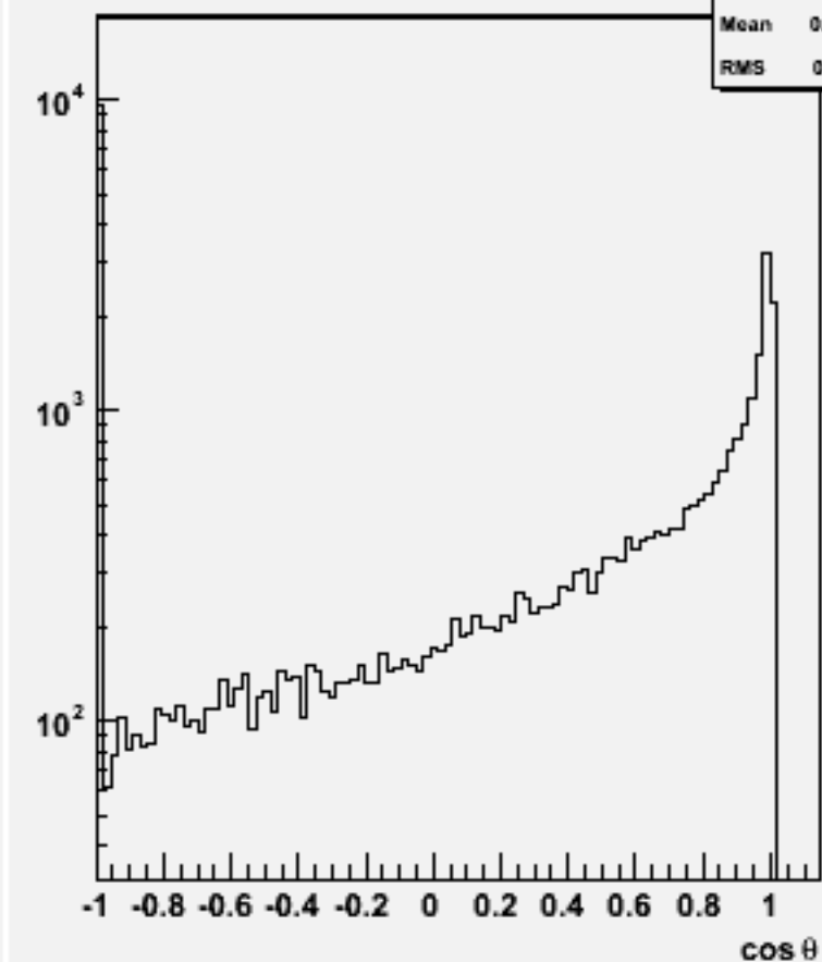
Jet cos \theta (All jets)w104005 aa_n3e3sc_o
