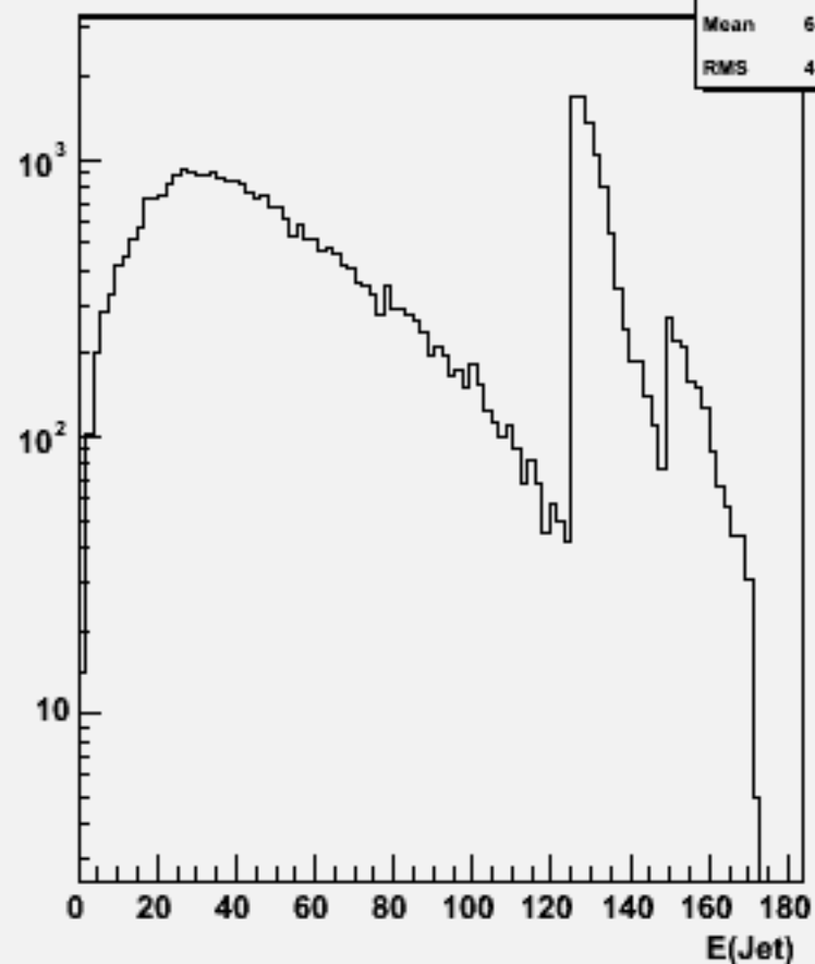
Jet energies(All jets)w104005 aa_n3e3sc_o
