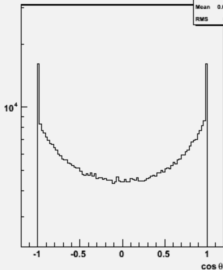
Particle cos \theta : w104004 aa_n3e3sc_o
