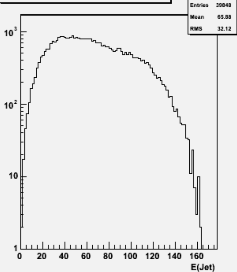
Jet energies(All jets)w104004 aa_n3e3sc_o
