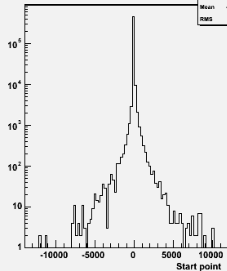
Start point Z : w104004 aa_n3e3sc_o
