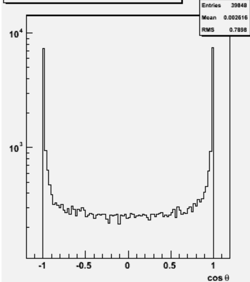
Jet cos \theta (All jets)w104004 aa_n3e3sc_o
