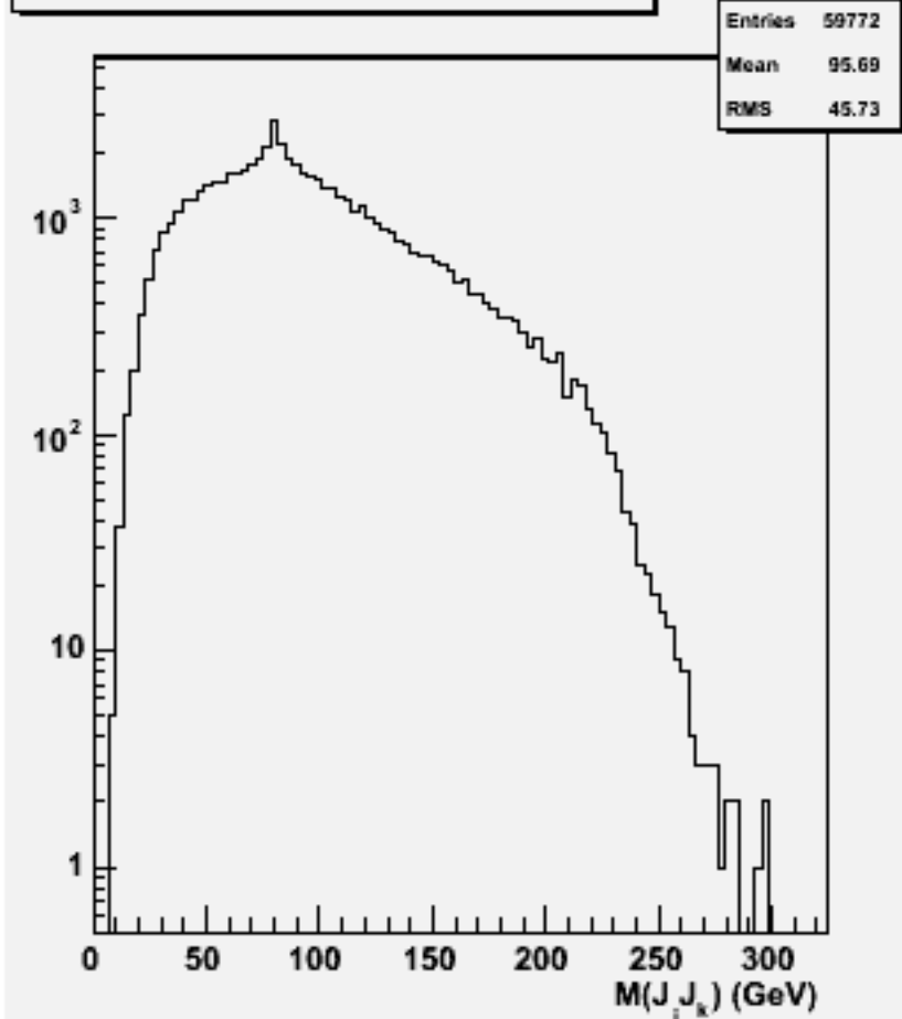
2jets mass(All comb)w104004 aa_n3e3sc_o
