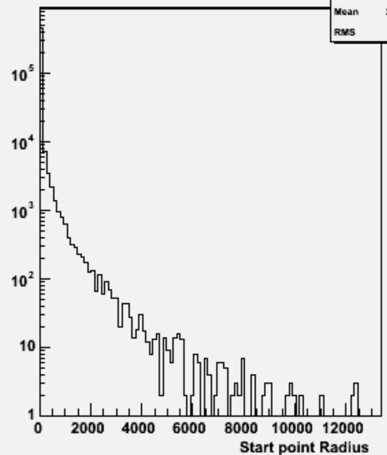
Start point R : w104004 aa_n3e3sc_o
