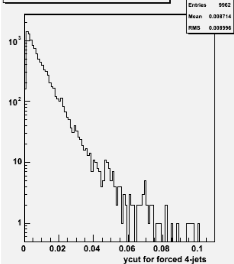
Ycut for 4-jets :w104004 aa_n3e3sc_o
