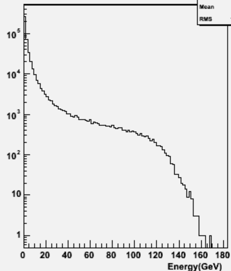
Particle Energy : w104004 aa_n3e3sc_o
